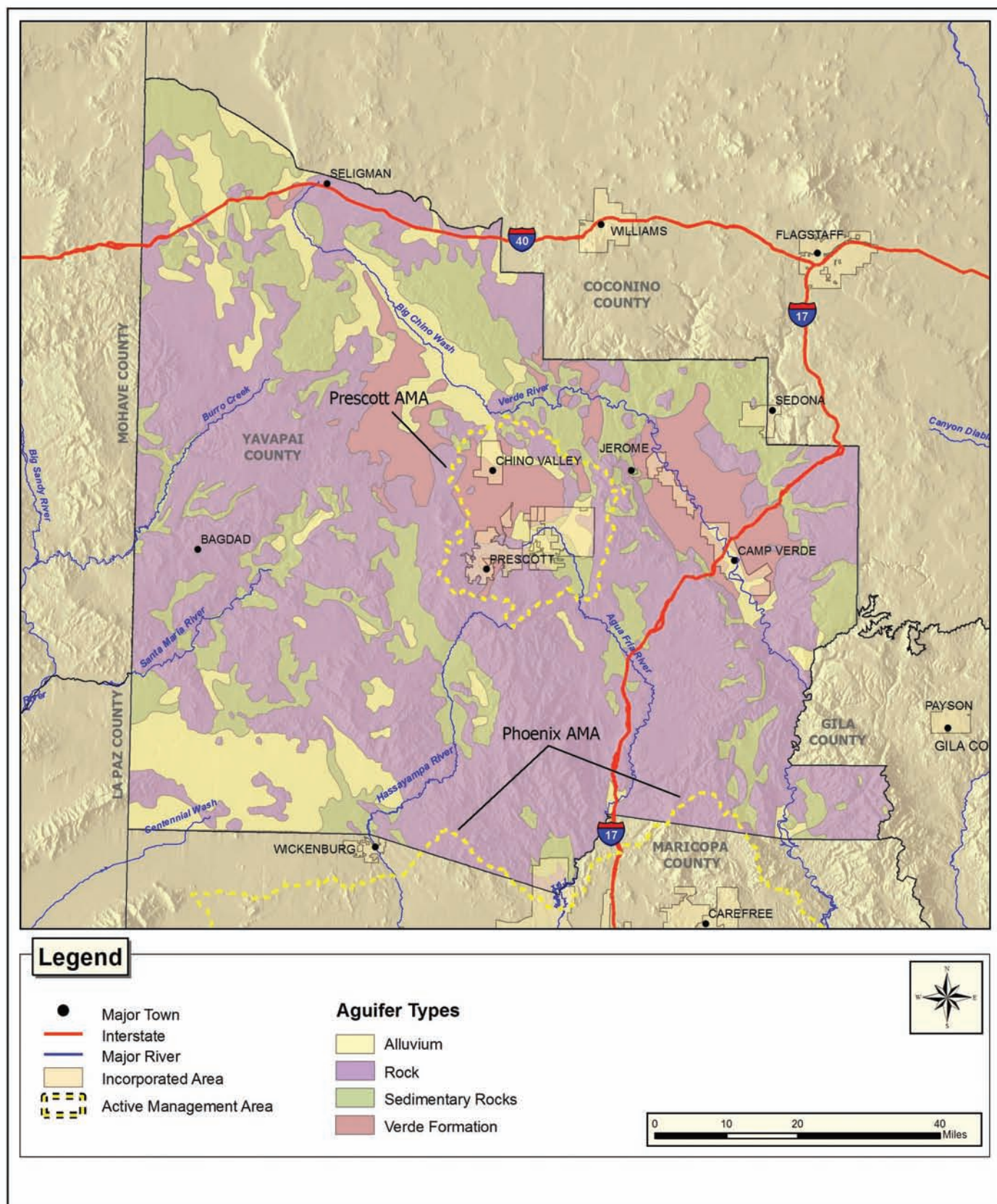
Figure 2. Yavapai County Aquifer Types and Prescott AMA
