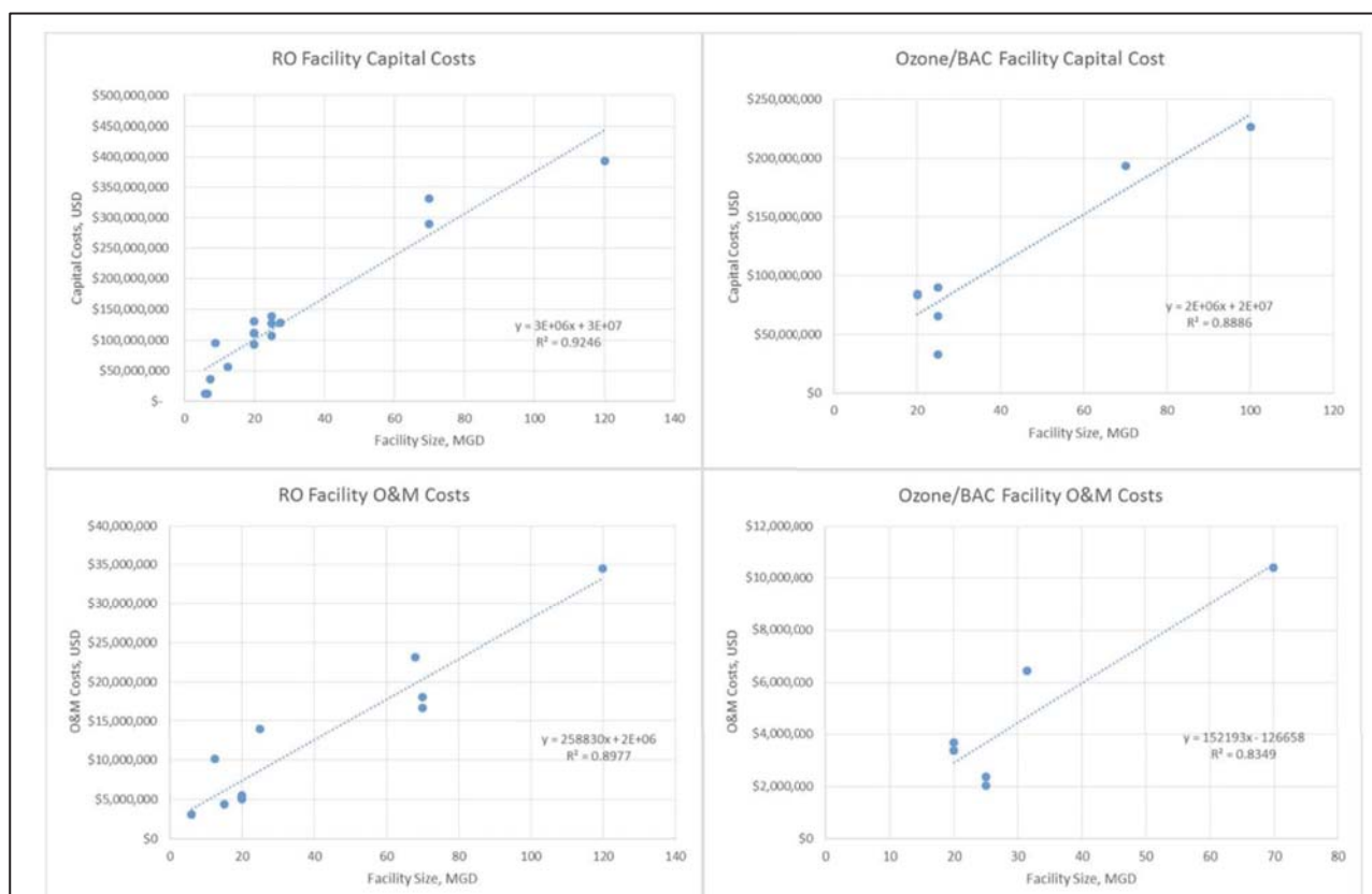
Figure 2-3: Relationship between Plant Capacity and O&M Costs for Full-Scale RO and Ozone-BAF Facilities (NMWRRI, 2017)
