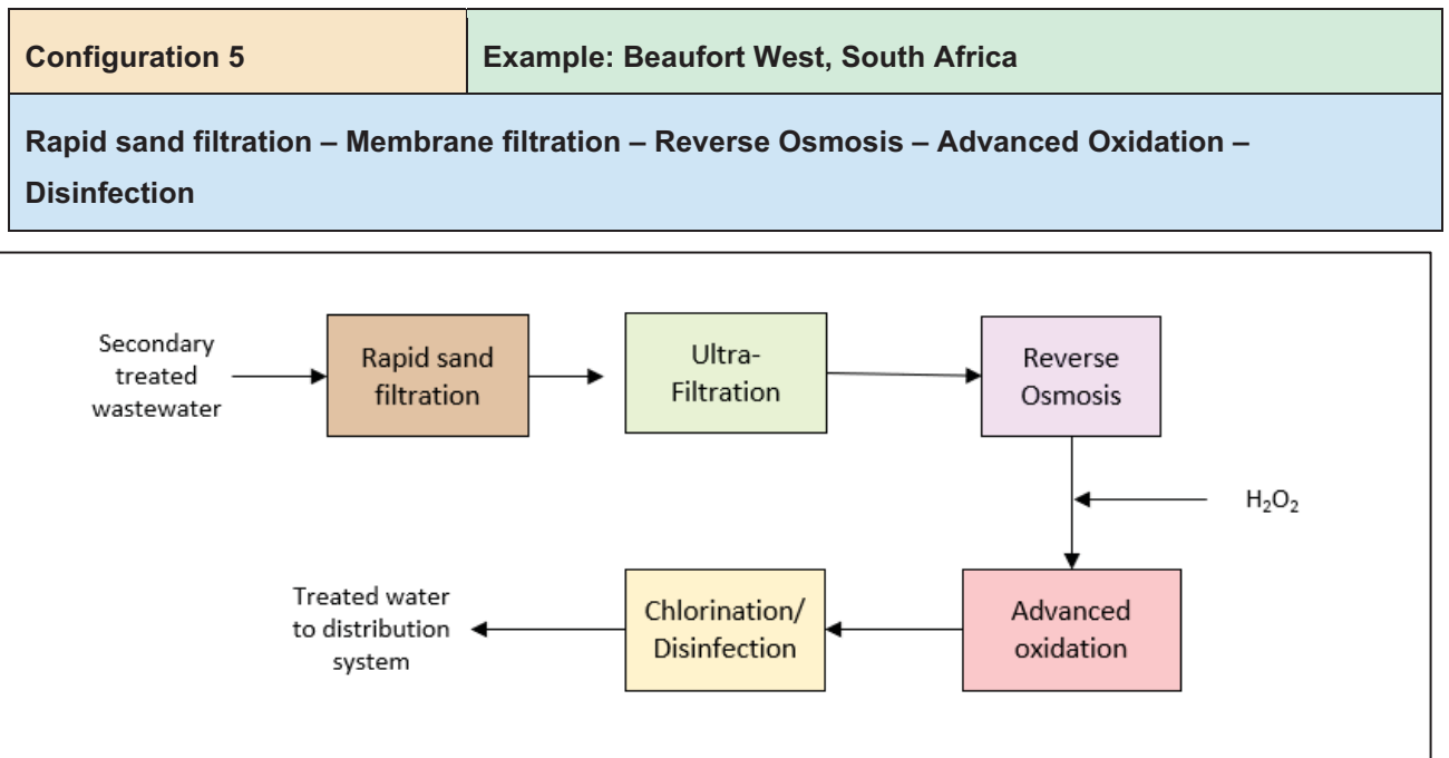
Figure 2-1: Most common process configurations used in water reclamation schemes (with examples)
