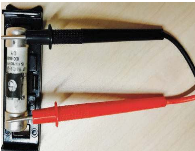
Figure 143: Fuse testing using Multimeter
