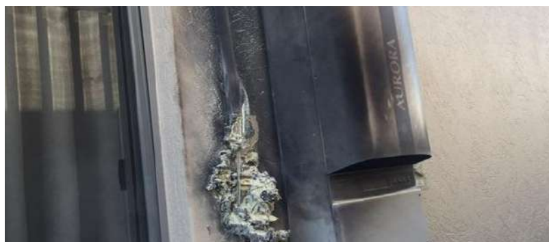
Figure 81: Inverter damage - Burn out
