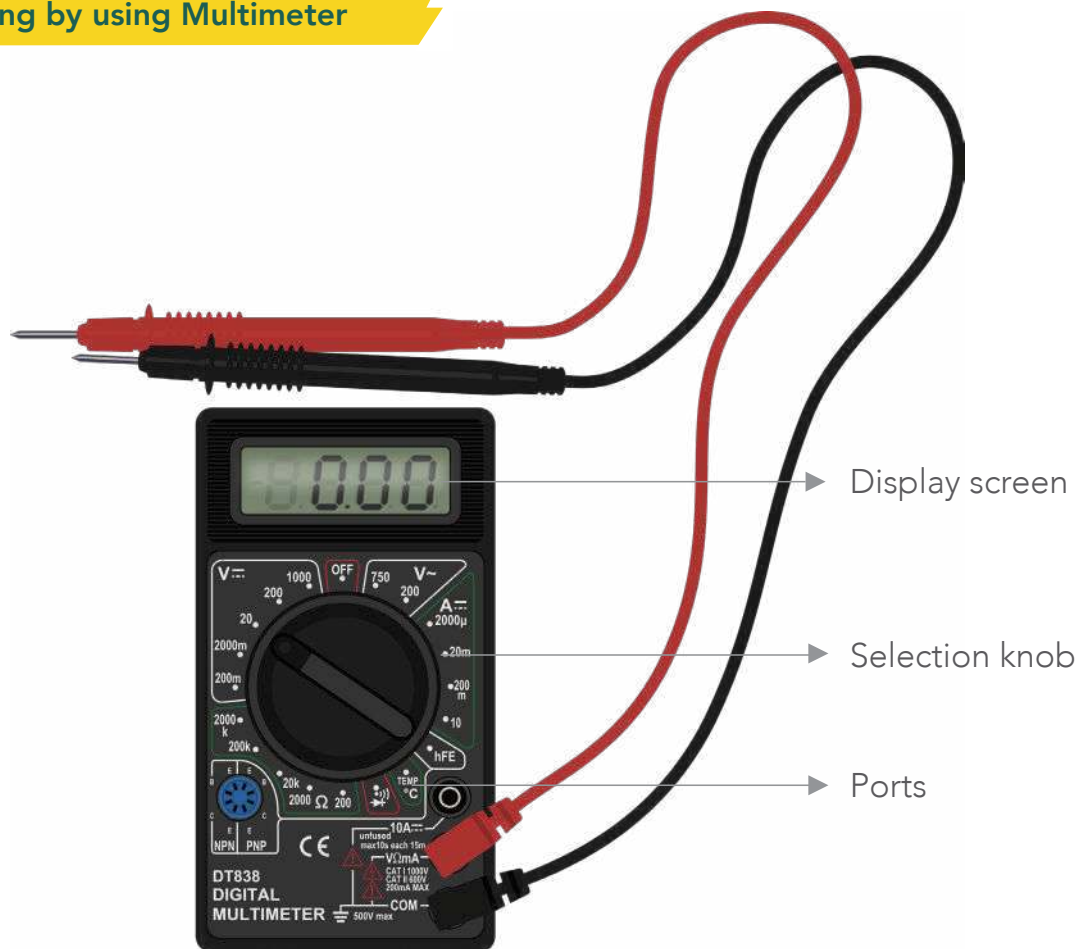
Figure 20: Digital Multimeter
