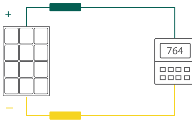
Figure 61: Voltage measurement
