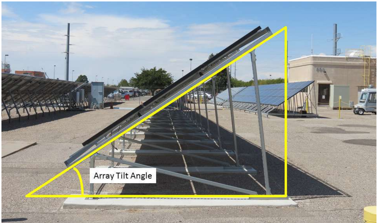
Figure 119: Tilt angle of PV Modules
