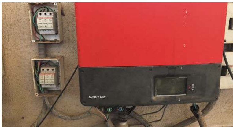
Figure 86: Inverter cables and conduits got loosed
