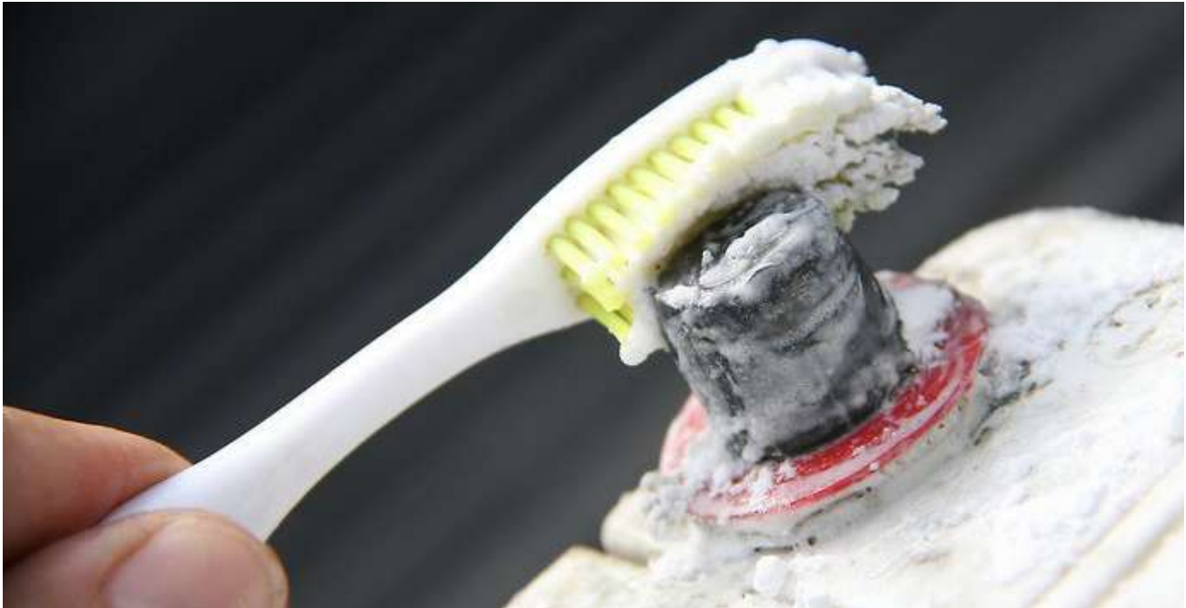
Figure 130: Battery cleaning using baking soda
