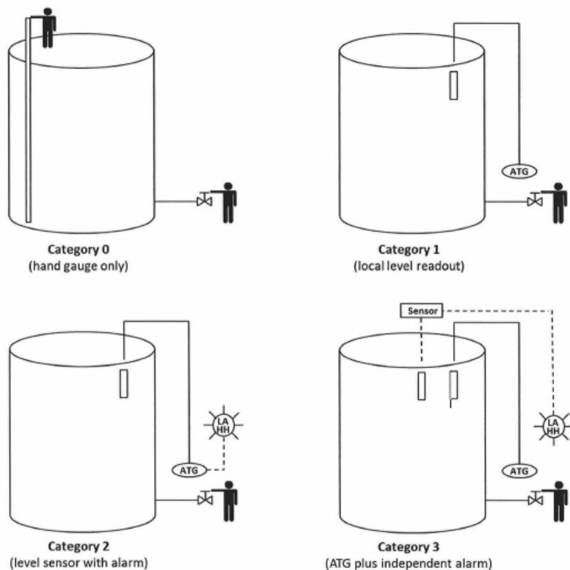
Figure 2: Definition of Overfill Protection System Categories
