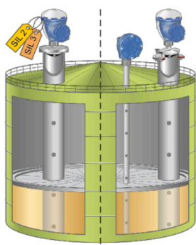
Floating Roof (Pipe)
