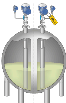
FMCW Radar (5900S)
