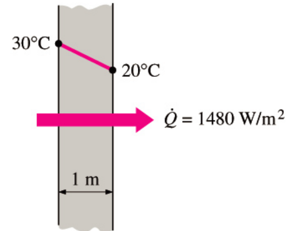
(b) Silicon ( k = 148 \text{ W/m}\cdot^\circ\text{C} )
