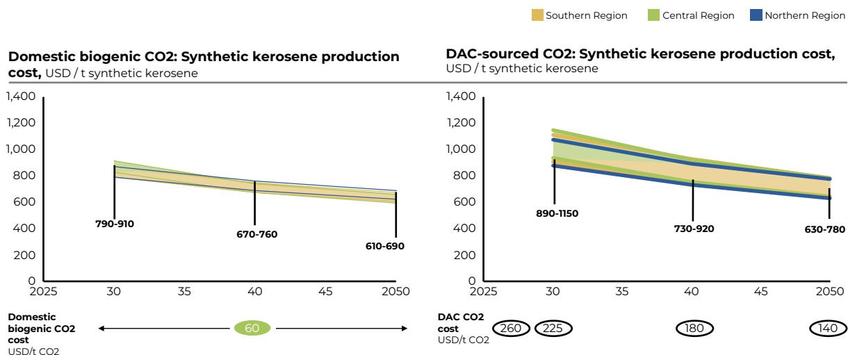
Exhibit 9: Synthetic kerosene production costs by CO 2 origin
