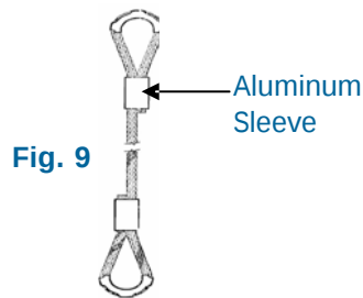
Fig. 9 FERRULE-SECURED SOFT EYE WITH STIRRUP
