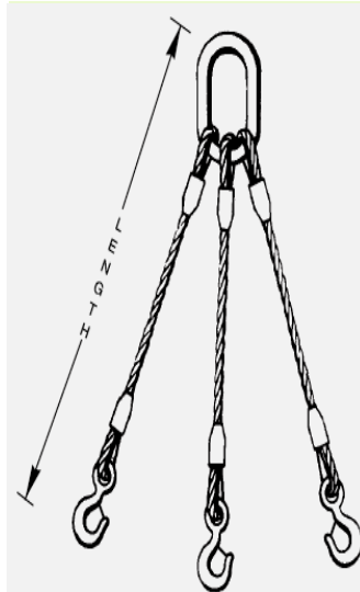
THREE-LEG SLING
