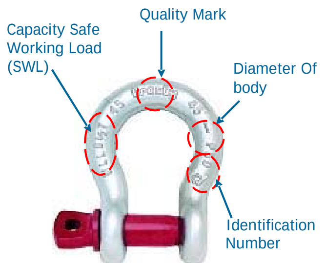
Fig. 8 BOW SHACKLE
