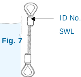
Fig. 7 FERRULE-SECURED HARD/THIMBLE EYE
