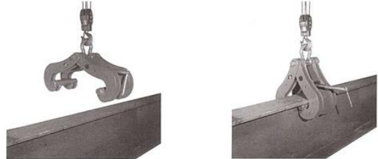
Fig. 4 ADJUSTABLE BEAM CLAMP
