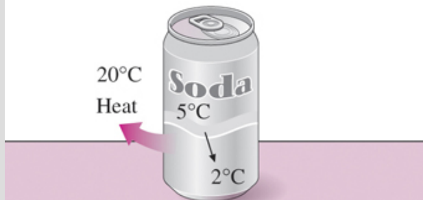
(b) An impossible heat transfer process
