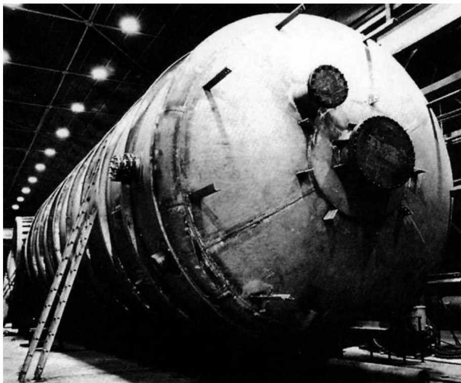
Process reactors in a petroleum refinery can either be solid stainless steel (above), clad, or protected with a weld overlay (below), such as might be used in an HDS reactor.
