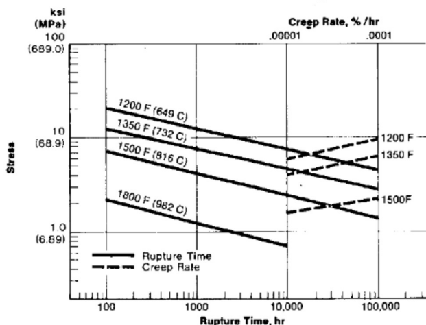
Figure 31 Stress Versus Rupture-Time and Creep-Rate Curves for Annealed Type 330 Stainless Steel Based on Average Data
