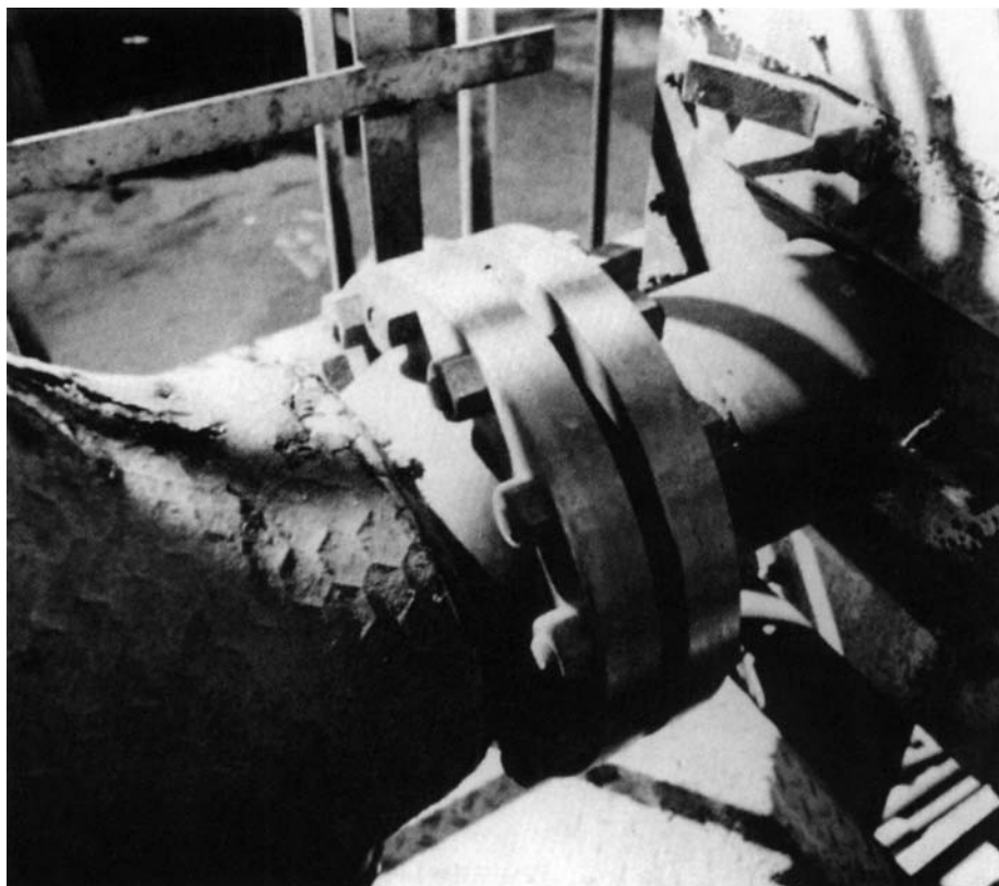
Figure 4 Type 316 flanges on a 316 outlet tube from a vacuum unit feed heater, point 10 in Figure 2. Tubing can be seamless or welded.
