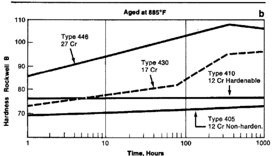
Graph of Hardness Versus Aging Time in Hours for Types 446, 430, 410 and 405 Chromium Steels. Hardening Tendency Increases with Chromium Content. Aged at 885°F.
