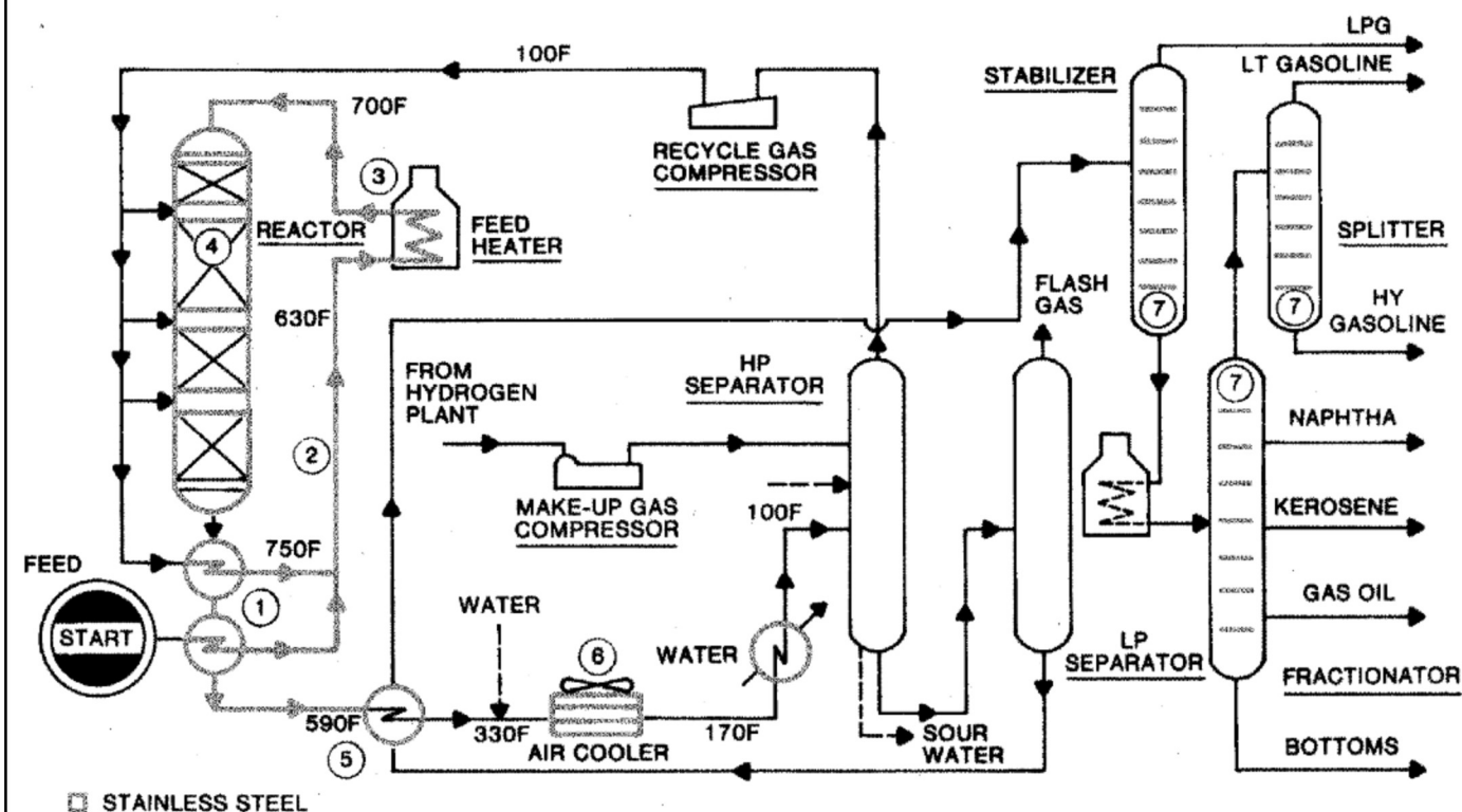
Figure 13 Hydrocracking
