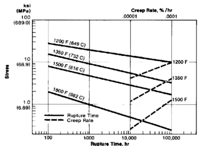
Figure 27 Stress Versus Rupture-Time and Creep-Rate Curves for Annealed Type 309 Stainless Steel Based on Average Data
