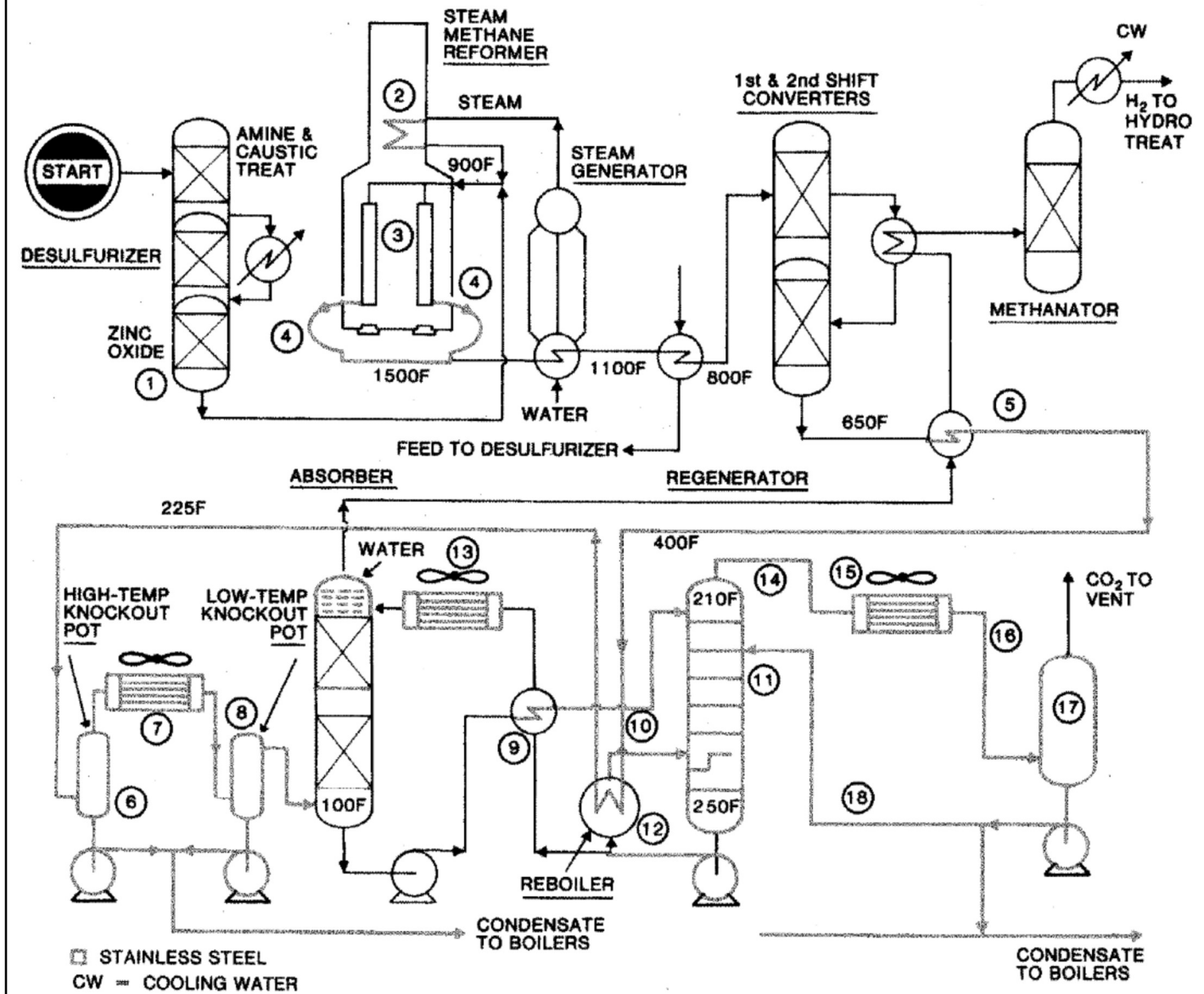
Hydrogen Plant
