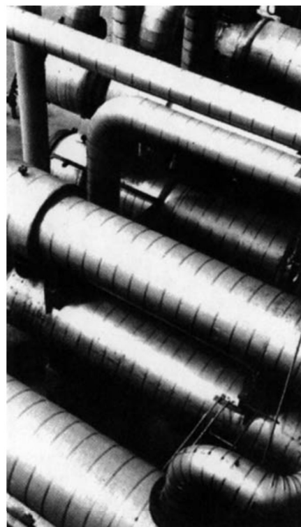
Type 430 stainless steel tubing in this feed-effluent heat exchanger operates at temperatures ranging from 300-600F (149-316C).
