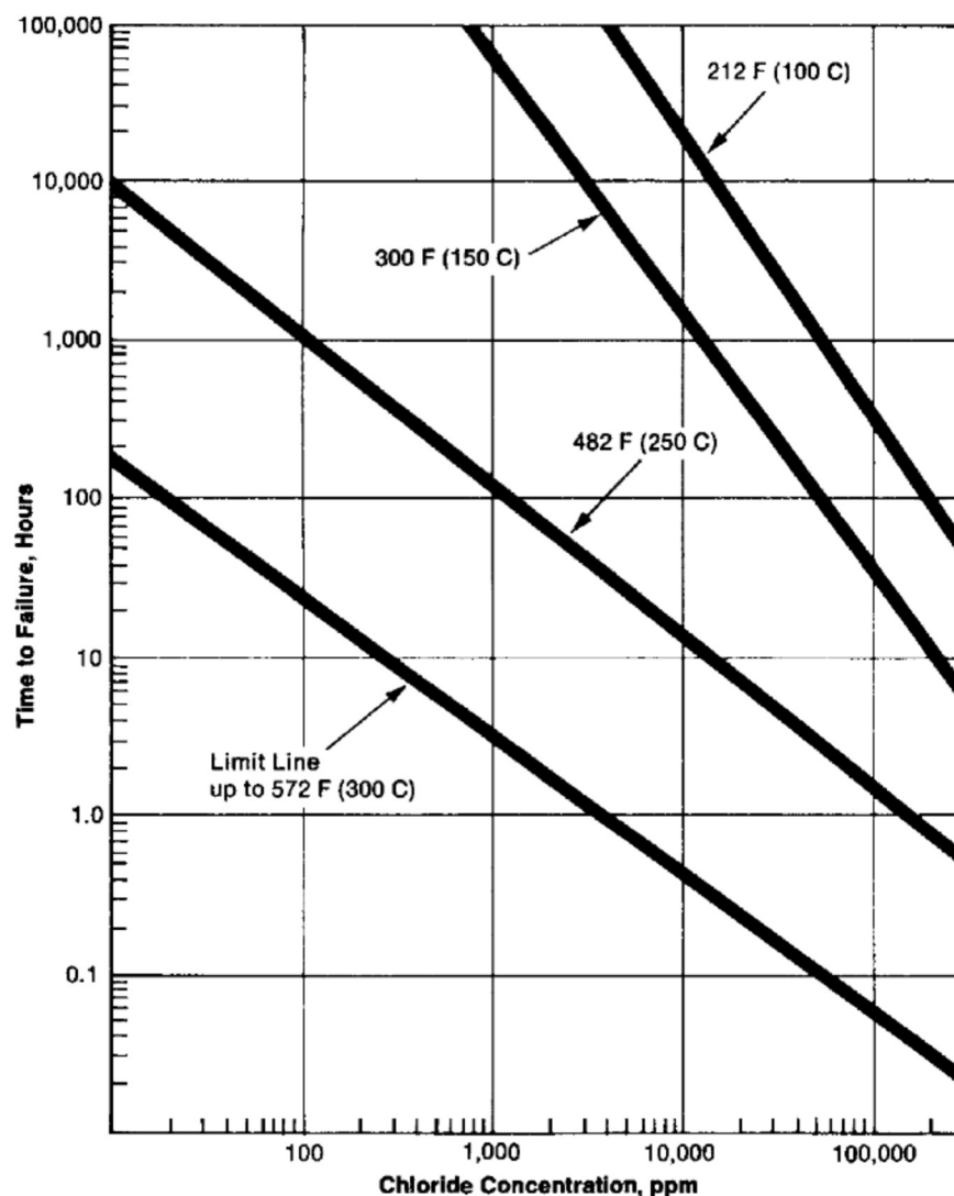
Figure 39 Stress-Corrosion Cracking of 18-8 Stainless Steel in Chloride Solutions
