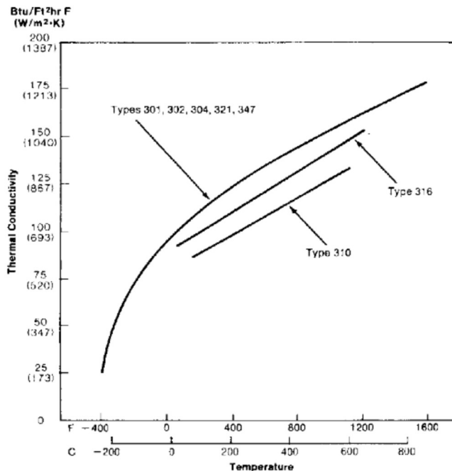
Figure 35 Effect of Temperature on the Thermal Conductivity of Chromium-Nickel Stainless Steels
