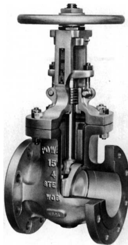
Figure 8 Numerous small parts throughout a refinery, such as valves, are constructed of stainless steel for resistance to erosion and corrosion. Stainless stems, gates, and seats assure trouble-free operation.
