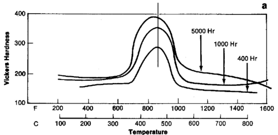
Graph of Hardness Versus Aging Temperature for 400 Hours, 1000 Hours and 5000 Hours, Using 27% Chromium Steel—Type 446.
