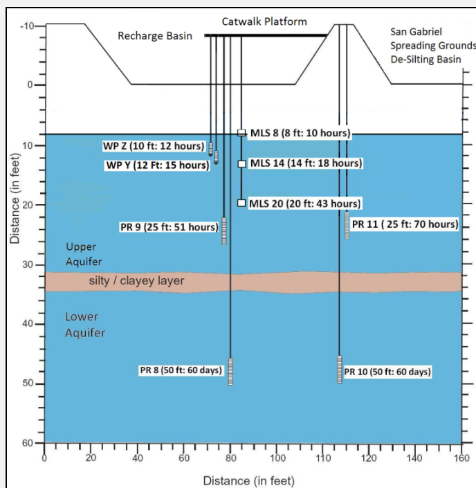
FIGURE 4-5 Instrumentation of groundwater recharge test basin associated with monitoring data provided in Table 4-3.
