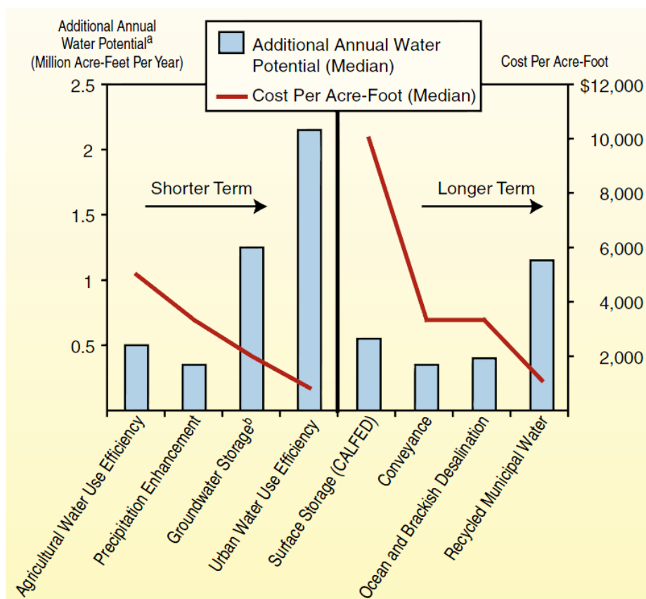
FIGURE 9-6 Costs of various water supply alternatives in the state of California. Cost estimates calculated by the California Department of Water Resources.
