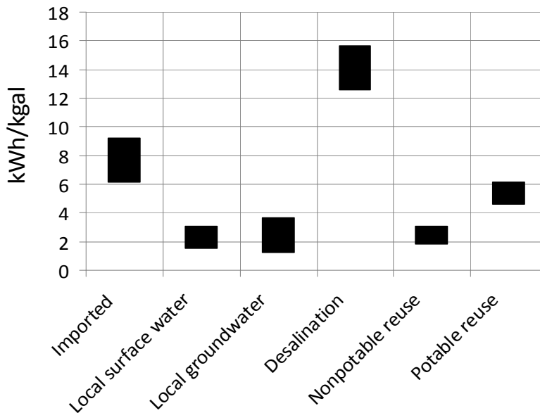
FIGURE 9-3 Power consumption for water supply alternatives for San Diego County. SOURCE: Data from Equinox Center (2010).
