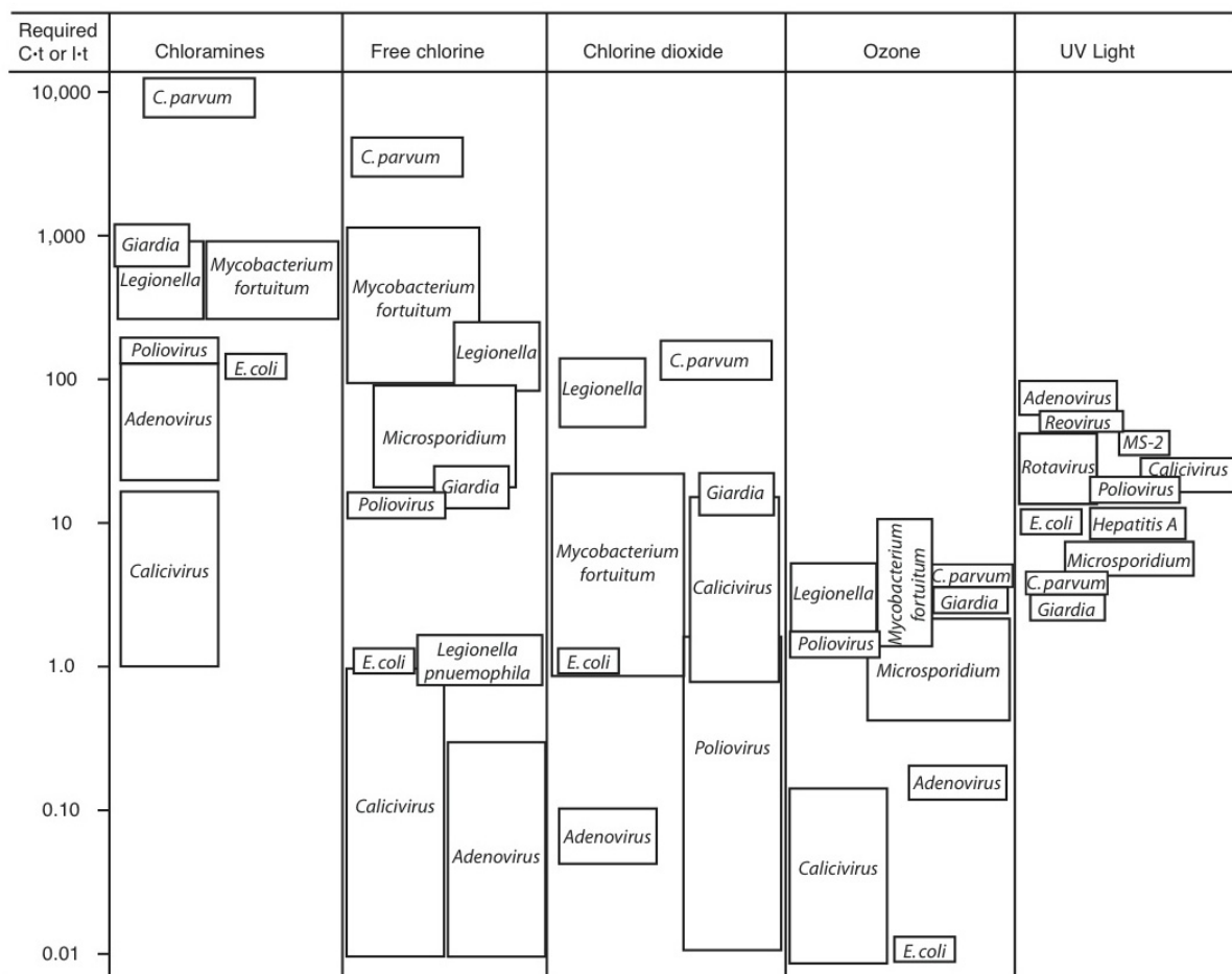
FIGURE 4-2 Required “C·t” or “I·t” for 99 percent inactivation of different organisms by different disinfectants at pH 7, 20-25 °C.
