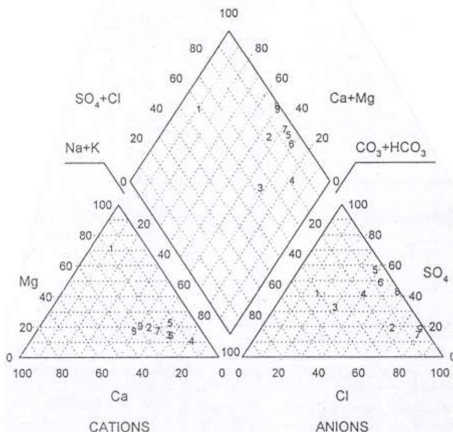
Fig. (8): Distribution of the water samples on Piper Diagram.
