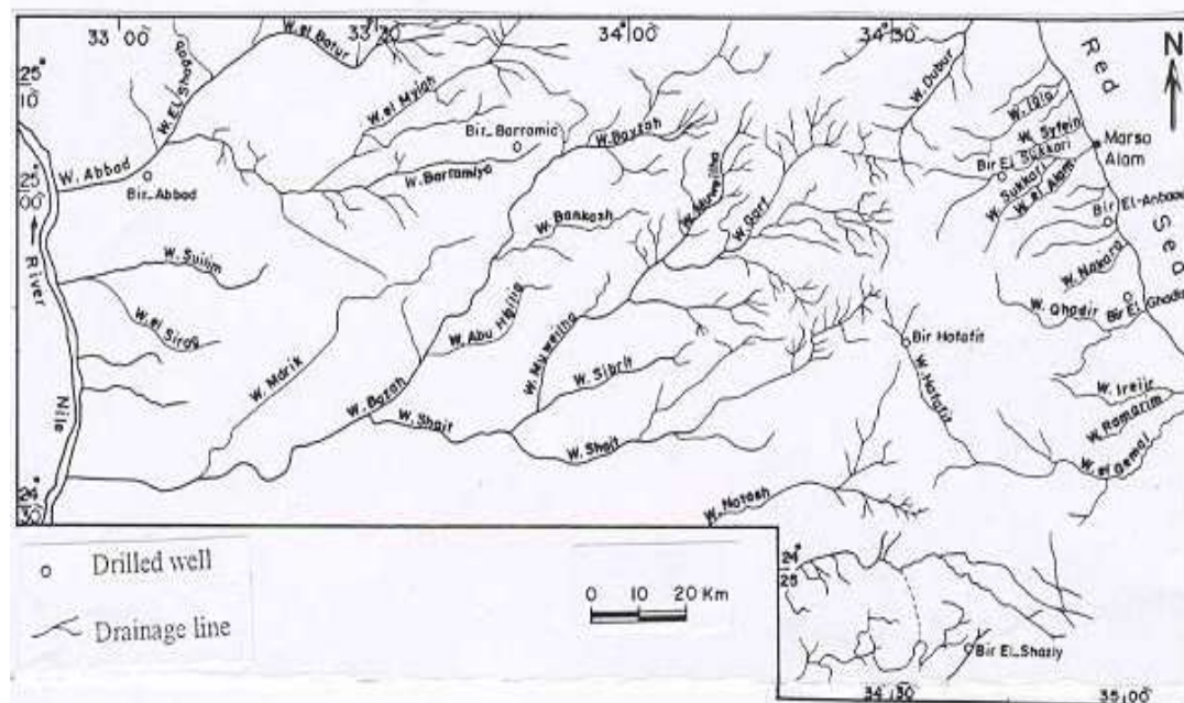
Fig. (2): The main wadies and wells in Idfu-Marsa Alam area.
