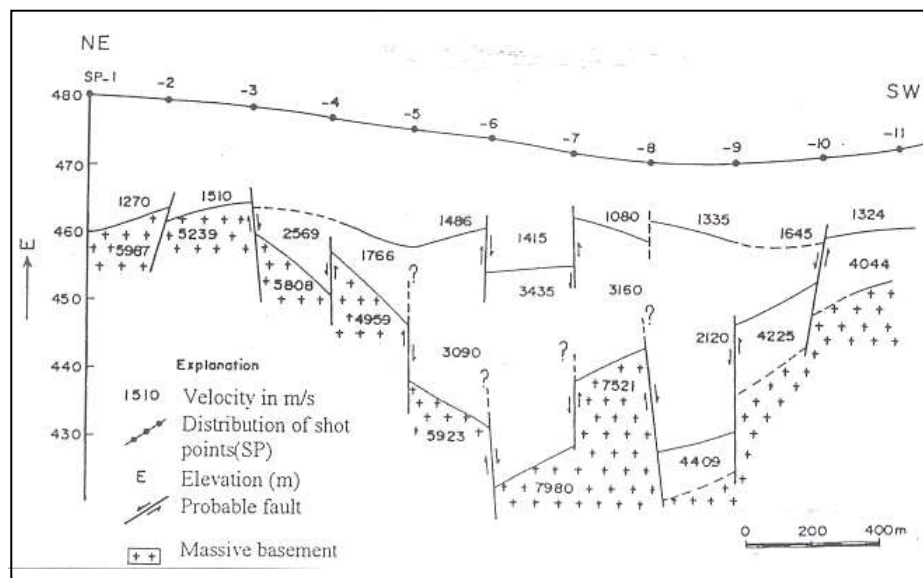
Fig.(6): Geoseismic cross-sections in the mountainous area (a in Wadi Hafafit , b in Wadi Natash and c in Wadi Abu-Hammamat).
