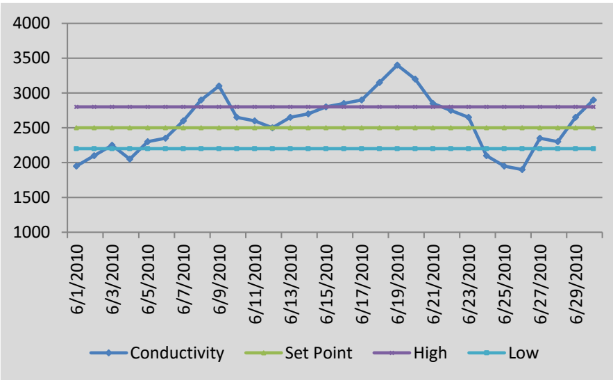
Manual Control
