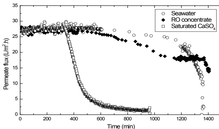
Fig. 3. Permeate flux of different saline solutions as a function of time (Permeate temperature T_p = 20^\circ\text{C} , V_f = 60 \text{ L/h} , V_p = 60 \text{ L/h} , feed volume = 10 L).
