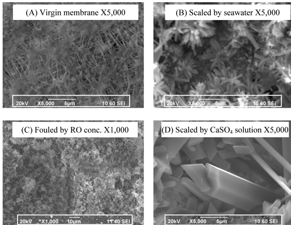
Fig. 4. SEM images of the membrane surface under clean and pre-fouled/scaled conditions: (A) virgin membrane, (B) after treating seawater, (C) after treating RO concentrate, and (D) after treating a saturated \text{CaSO}_4 solution.
