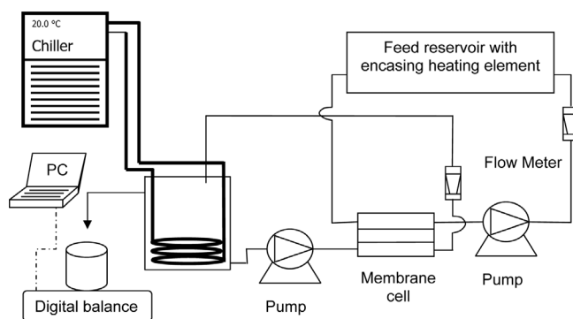
Fig. 1. Schematic diagram of the DCMD system.
