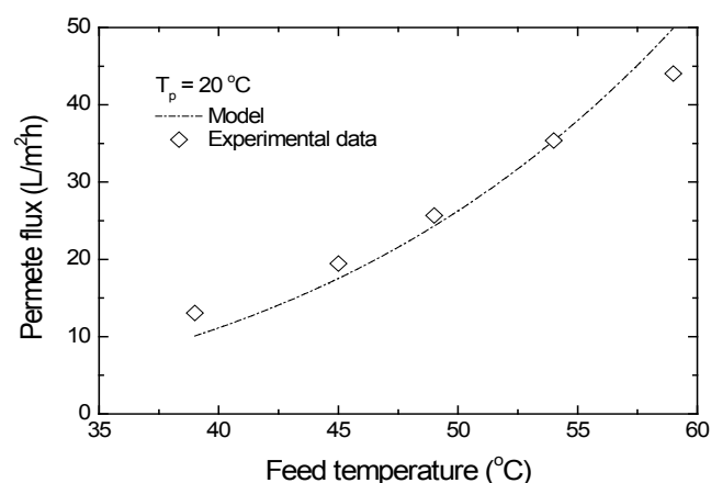
Fig. 2. Modelled and experimental permeate flux as a function of feed temperature (Permeate temperature T_p = 20^\circ\text{C} , V_f = 60\text{ L/h} , V_p = 60\text{ L/h} , tap water with pH \sim 7 ).
