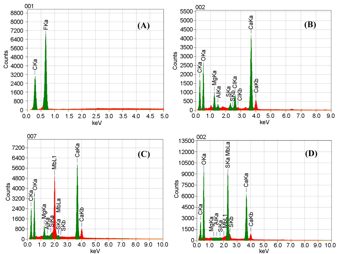
Fig. 5. EDS spectra of the membrane surface under clean and pre-fouled/scaled conditions: (A) virgin membrane, (B) after treating seawater, (C) after treating RO concentrate, and (D) after treating a saturated \text{CaSO}_4 solution.
