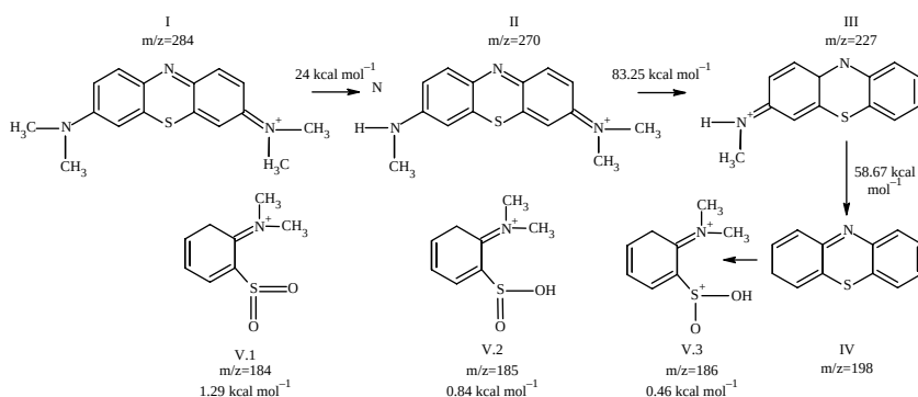
Figure 10.5 The reaction scheme of methylene blue dye ( m/z = 284 ) oxidation with all the identified intermediates by Nb-substituted goethites in the presence of \text{H}_2\text{O}_2 with the energy barrier for every intermediate (Adapted from Oliveira et al. , 2008)
