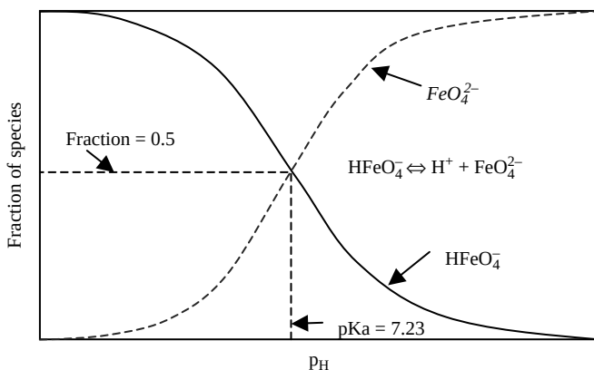
Figure 6.2 Changes in fraction of Fe(VI) species at different pH with \text{pK}_a = 7.23 at 25^\circ\text{C} (extracted from Sharma, 2008)
