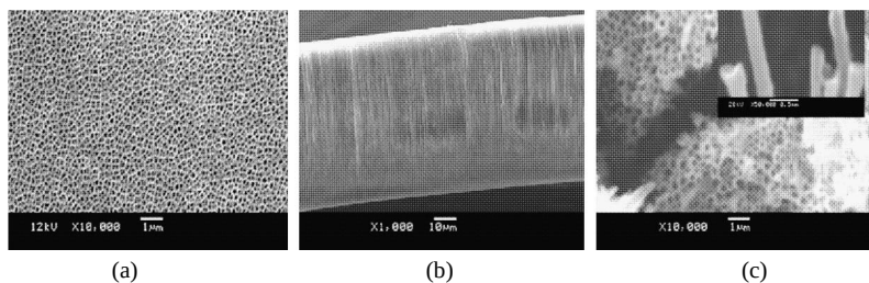
Figure 4.3 SEM photograph of: (a) the surface of 20%-silica/titania composite membrane; (b) the cross-section of 20%-silica/titania composite membrane; (c) 20%-silica/titania nanotubes ( \times 10,000 and \times 50,000 )
