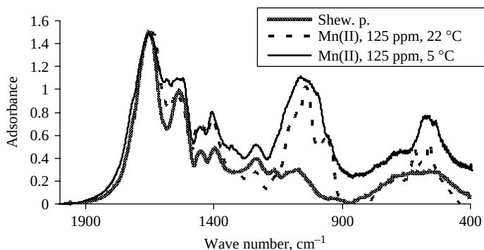
Figure 5.10 FTIR spectra of the (initially) viable Shewanella putrefaciens before and after sorption of \text{Mn}^{2+} . Batch conditions of \text{Mn(II)} sorption: contact time: 24 days, background electrolyte: 0.1N NaCl, temperatures: 5 and 22 \pm 2^\circ\text{C} , bacteria concentration: 2 \text{g}_{\text{dw}}/\text{L} (Chubar et al. , not publ.)
