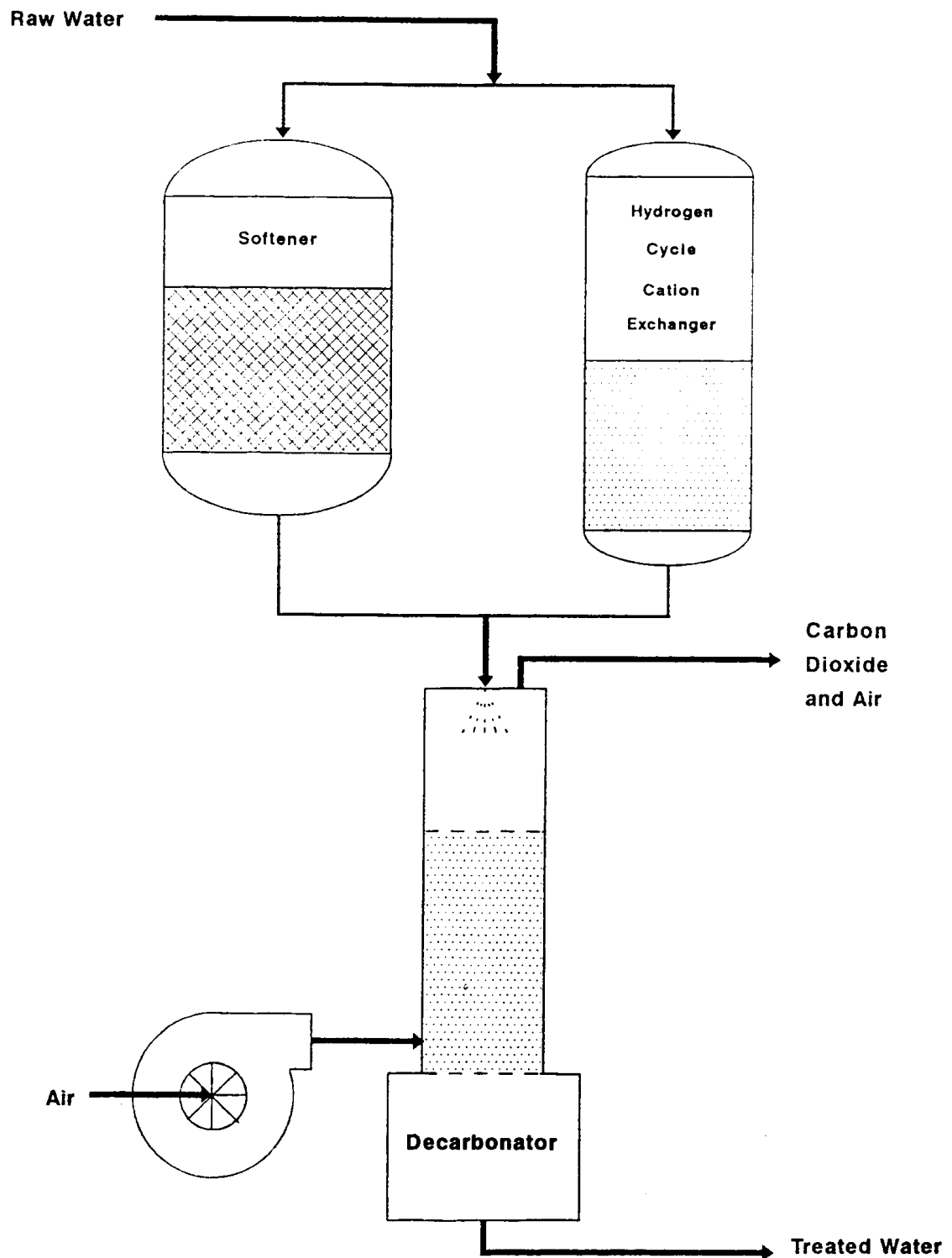
FIGURE 2-5 SPLIT STREAM DEALKALIZER
