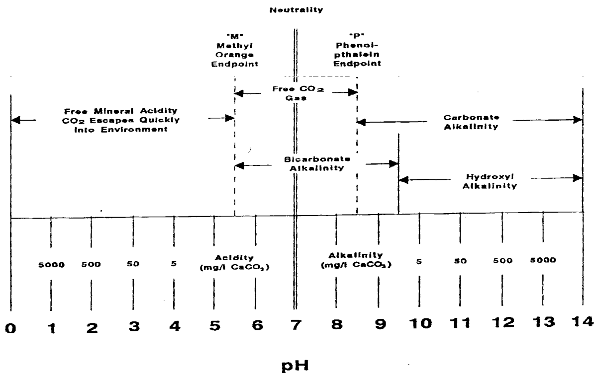
FIGURE 6-4 ACIDITY & VARIOUS TYPES OF ALKALINITY & THEIR pH RANGES
