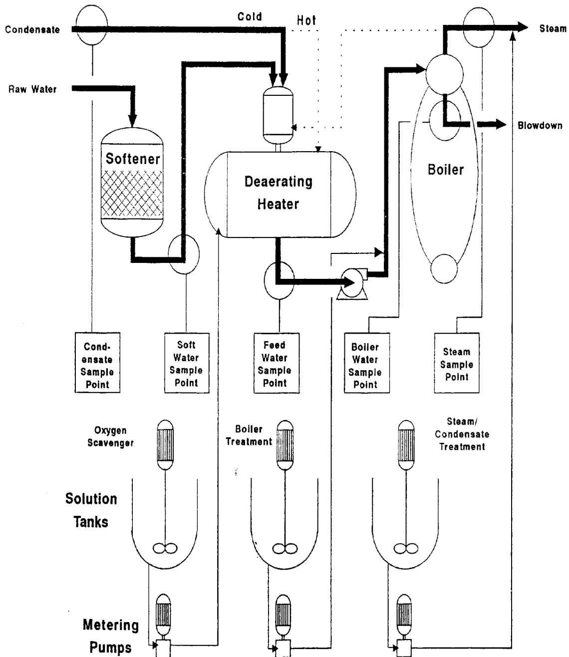
FIGURE 6-3 TYPICAL LOCATIONS FOR WATER SAMPLING POINTS IN A STEAM BOILER SYSTEM
