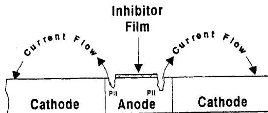
(E) Pitting Attack
