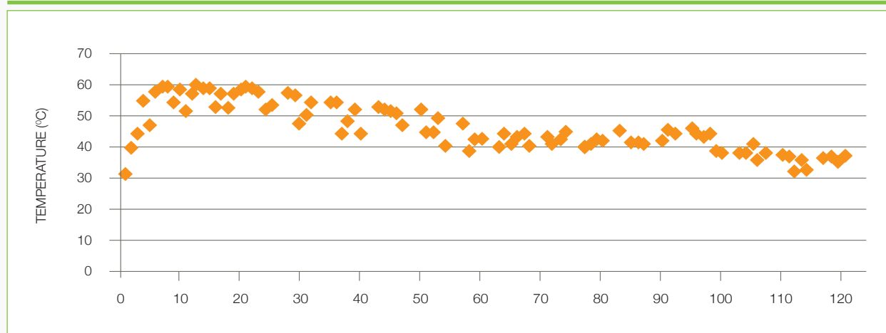
FIGURE 19. TEMPERATURE CHANGES DURING CO-COMPOSTING OF DFS:SD (1:3) HEAP.
