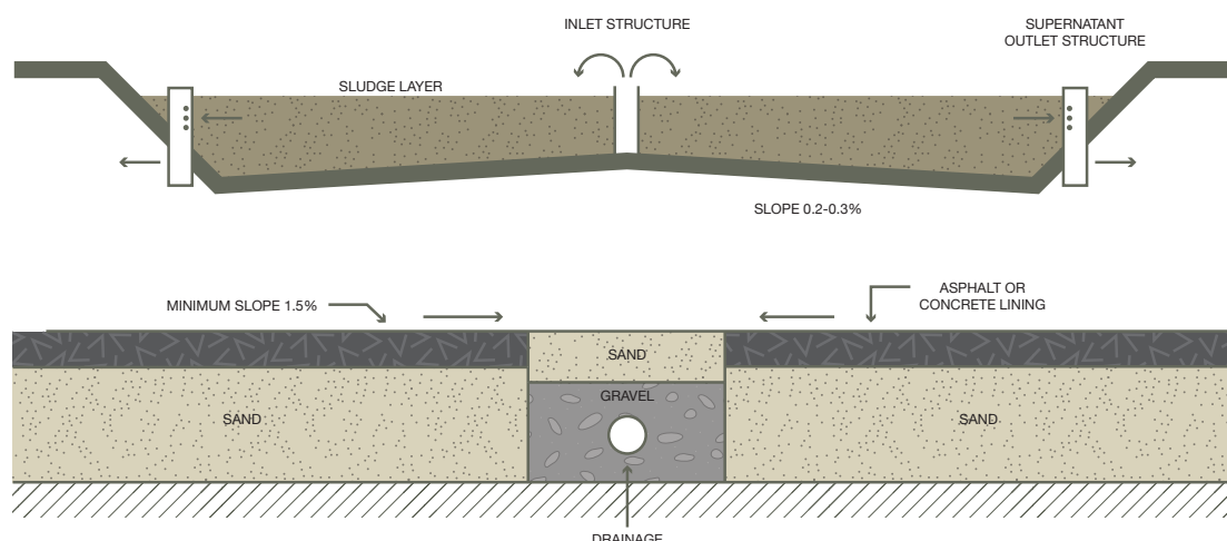
FIGURE 7. PAVED DRYING BED.
