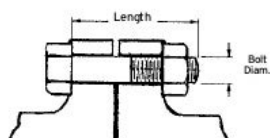
Flat faced joint illustrated
