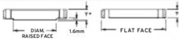
BLANK OR BLIND FLANGE
