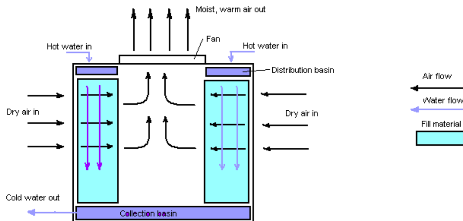
Fig 7. Crossflow type design
