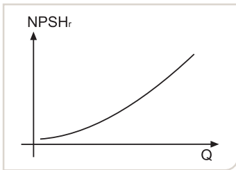
Fig. 7.3.1d NPSHr curve
