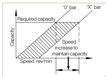
Fig. 7.6.1c Pressure effect
