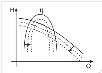
Fig. 7.3.1e Effects on Q, H and \eta
