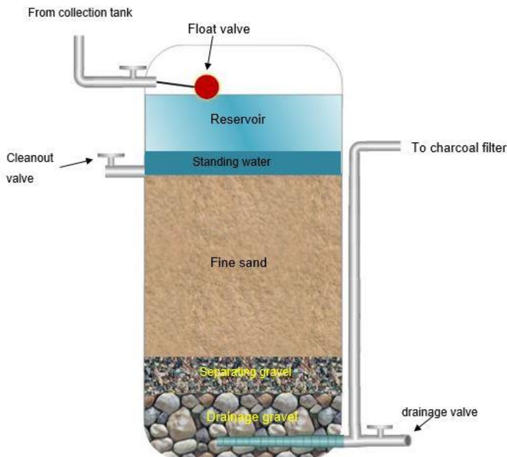
Figure 12 Conceptual design of sand filter
