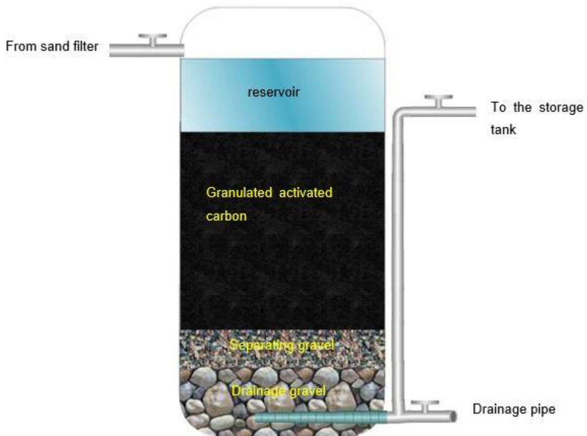
Figure 13 Activated carbon tank specifications
