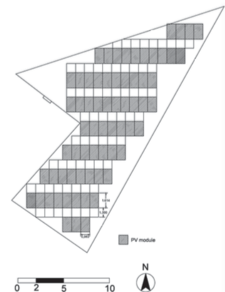
Fig. 5: Solar PV panel roof placement
