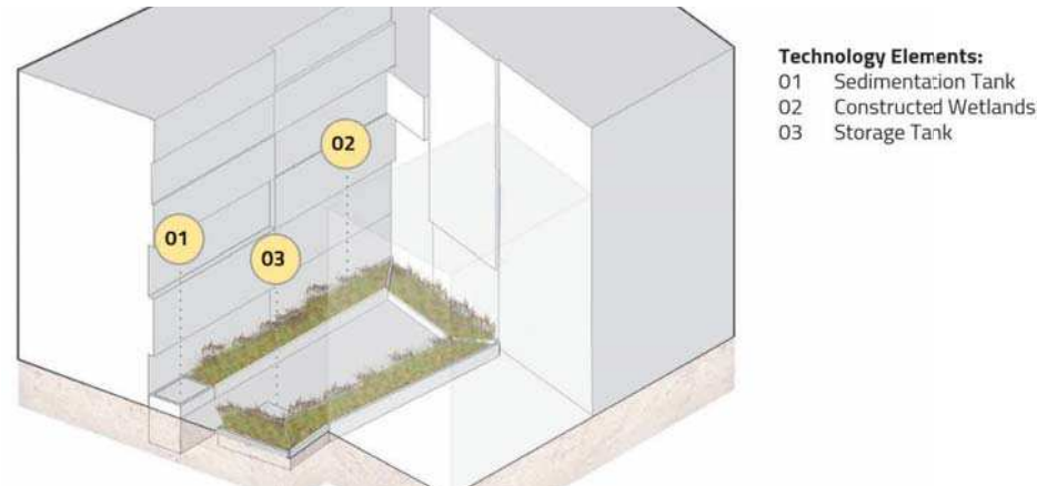
Fig. 11: View of proposed constructed wetland elements
