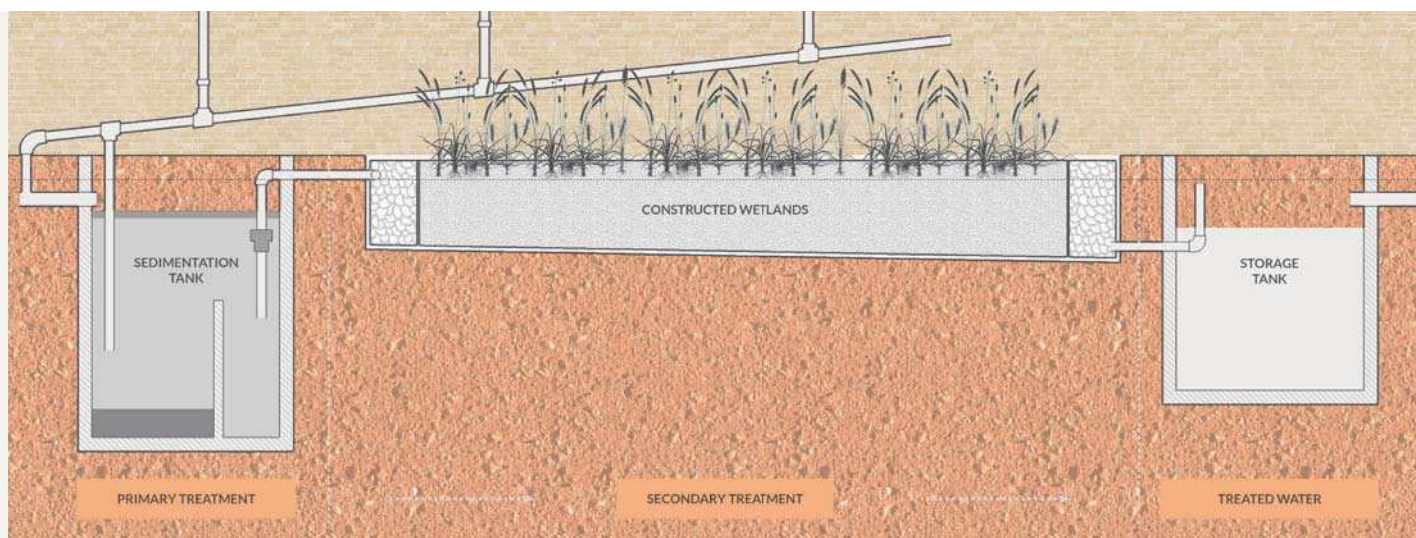
Fig. 4: Components of greywater treatment system for pilot project in El Gamaleya
