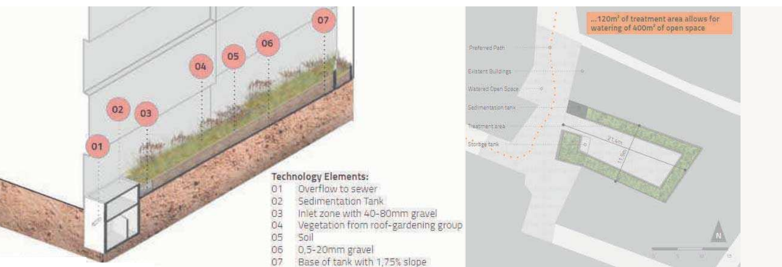
Fig. 7: Cross section (left) and plan (right) of the constructed wetland for the pilot project
