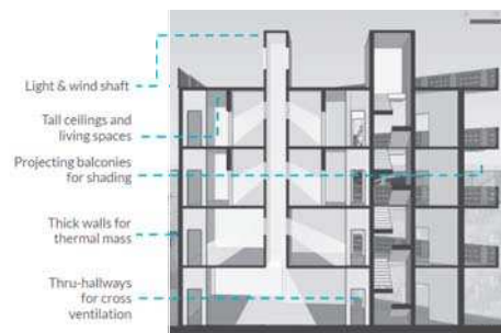
Fig. 7: Building section
