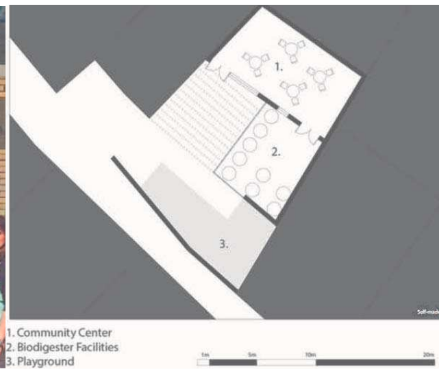
Fig. 9: Bio EnGen plan: (1) community center; (2) bio-digester facilities; (3) playground
