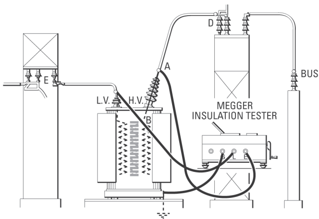
Figure 34-Connections for testing insulation resistance between high and low voltage windings without being affected by leakage to ground.
