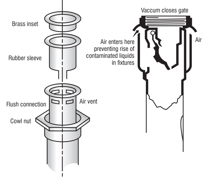
FIGURE 57. Vacuum breakers.
