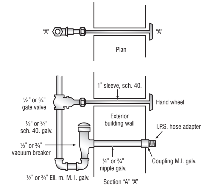
FIGURE 58. Vacuum breaker arrangement for an outside hose hydrant.
