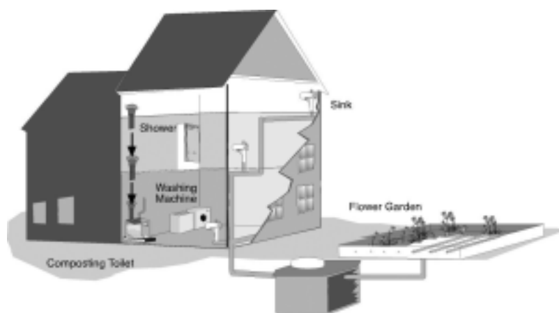
Figure 3-6. Typical graywater reuse approach
