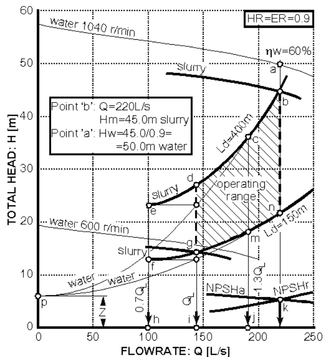
Fig.11.6 – Pump Performance and System Resistance
