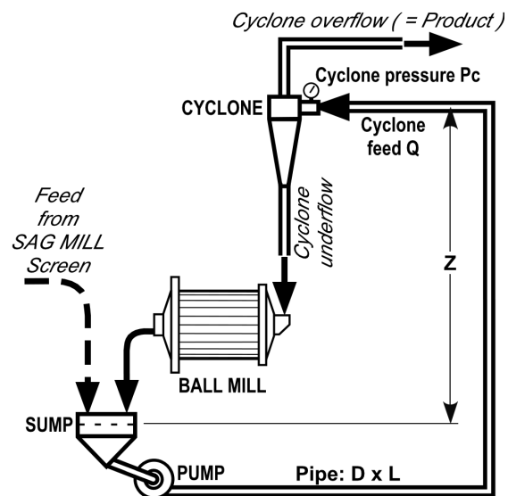
Fig.11.2 – Ball Mill, pump and cyclone circuit
