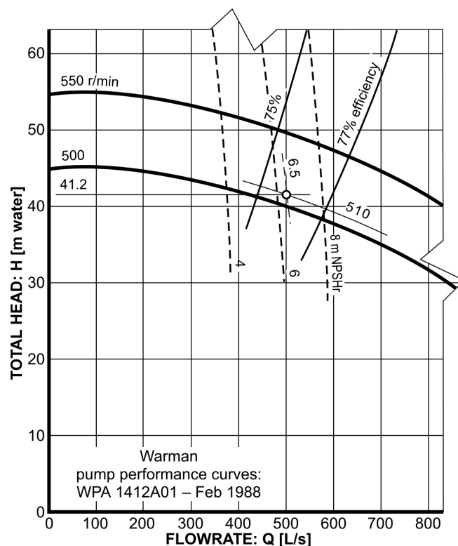
Fig.8.4 – Portion of Warman 14/12 FF- AH pump performance curves
