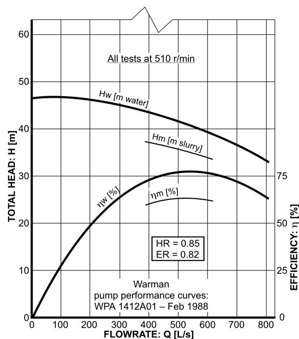
Fig.10.2 – Pump test results for Head and Efficiency ratios
