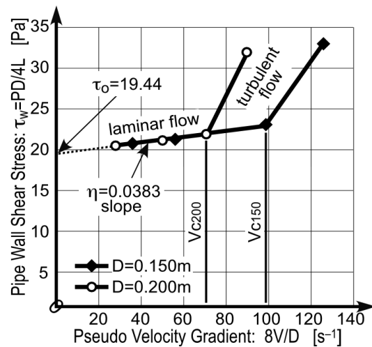
Fig.5.5 – Rheology Graph
