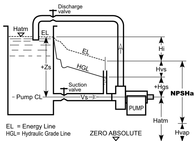
Fig.8.1 – Pump test setup for testing NPSH with positive suction conditions
