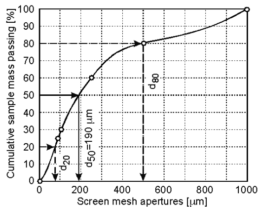
Fig.7.5 – Sizing of solids in slurry
