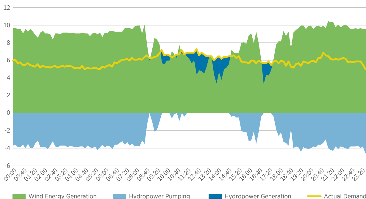
Figure 6 Gorona del Viento demand and generation, 5 September 2018
