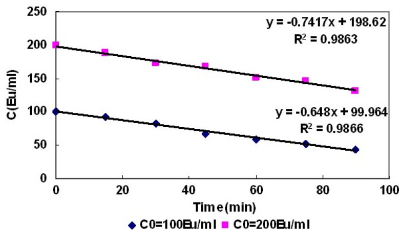
Fig. 2: Endotoxin inactivation versus reaction time (pH 7, T=20±0.5, ozone dose=0.45g/h)
