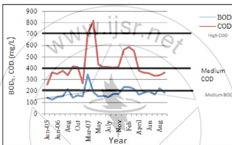
Figure 2: Average monthly variations of BOD 5 and COD of the influent wastewater of Al-Diwaniyah WWTP (2005-2016)
