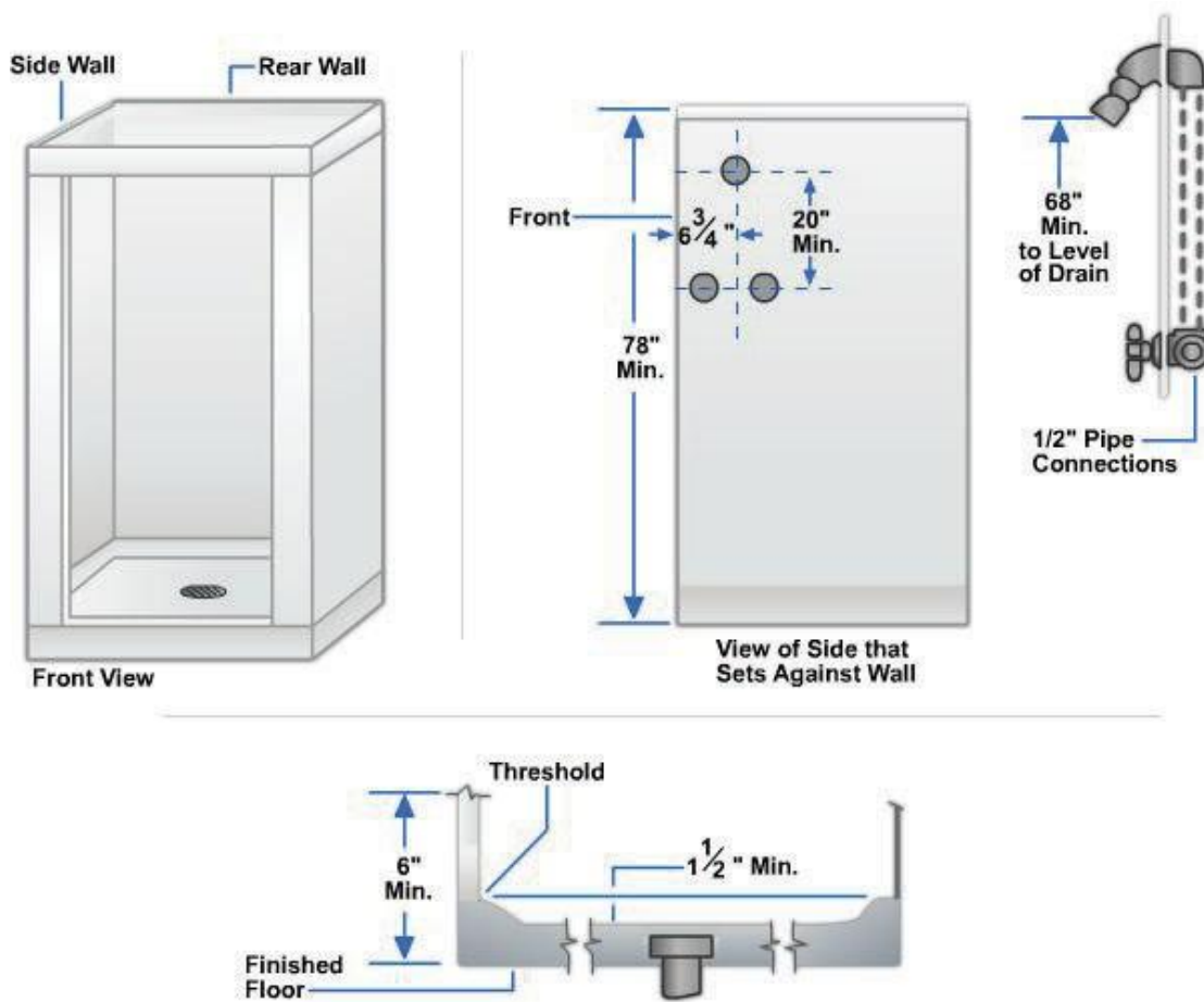
Figure 6-24 – Shower stalls and sections.
