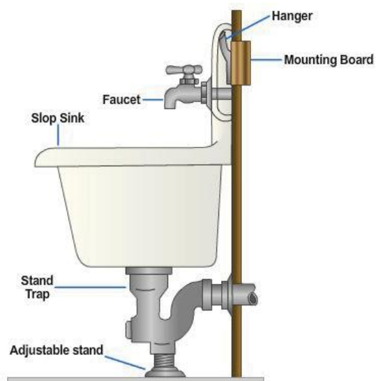
Figure 6-13 – Service (slop) sink.
