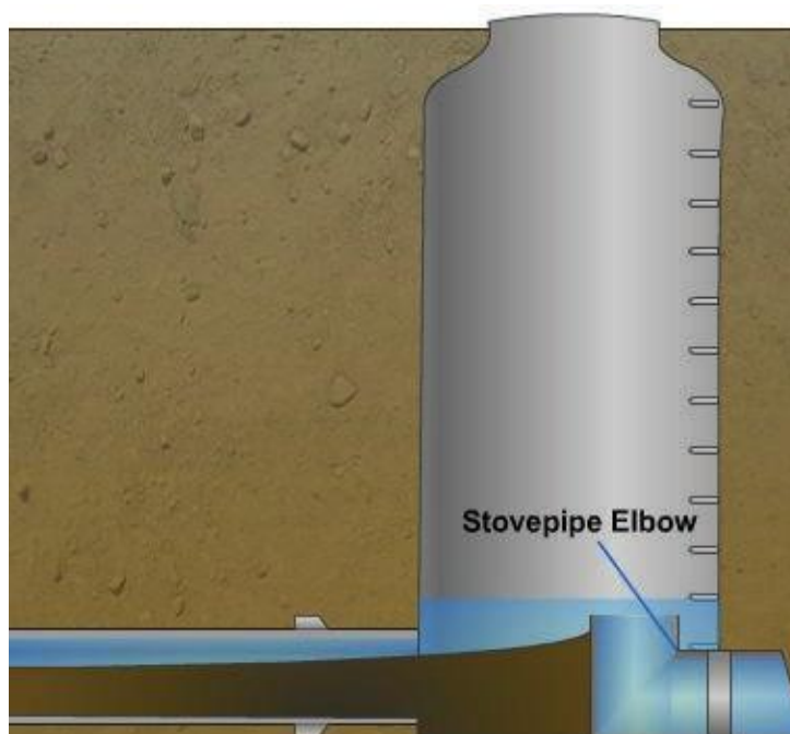
Figure 6-46 – Sand trap.
