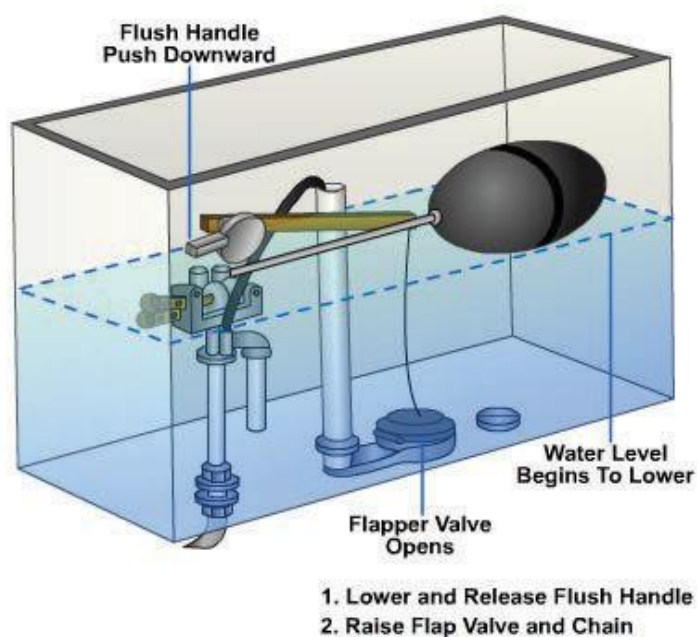
Figure 6-36 – Flush tank process.
