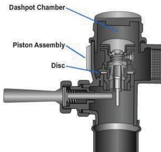
Figure 6-39 – Piston type flushometer valve.
