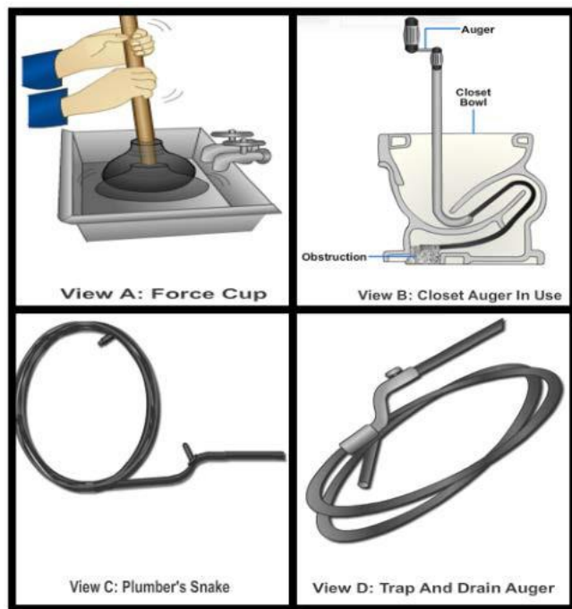
Figure 6-49 – Tools for clearing stoppages in plumbing fixtures.
