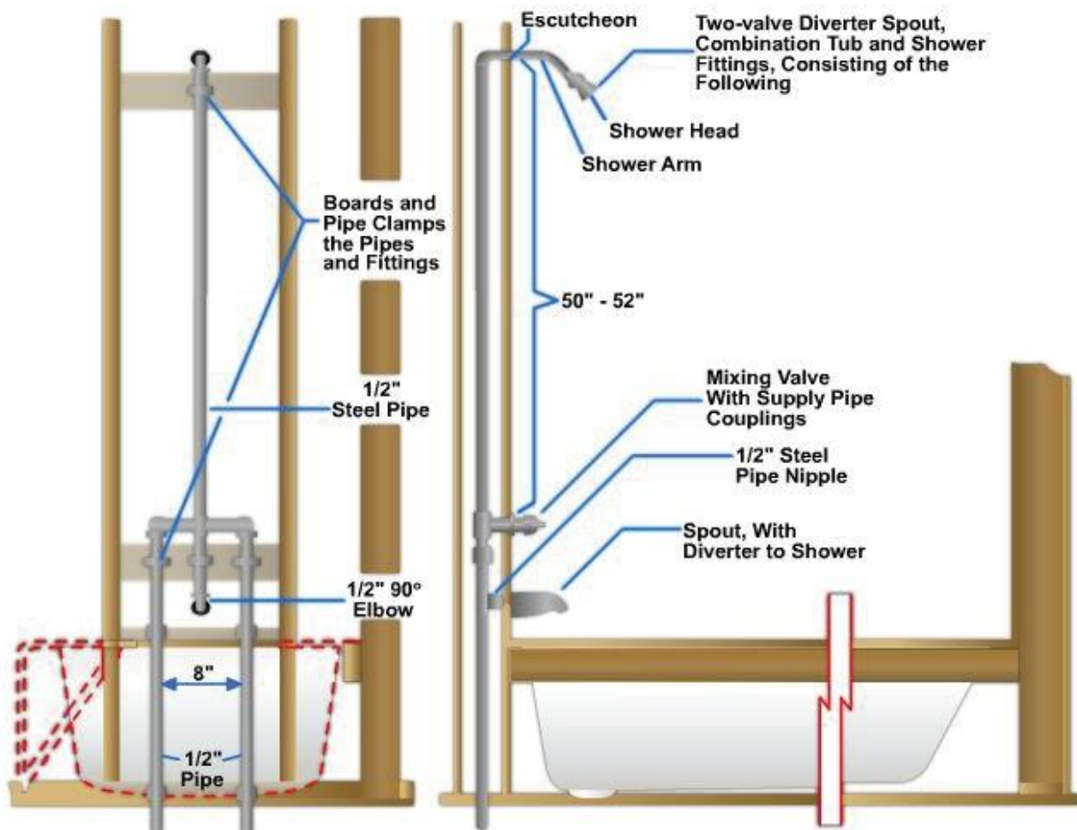
Figure 6-18 – Bathtub and shower piping combination.
