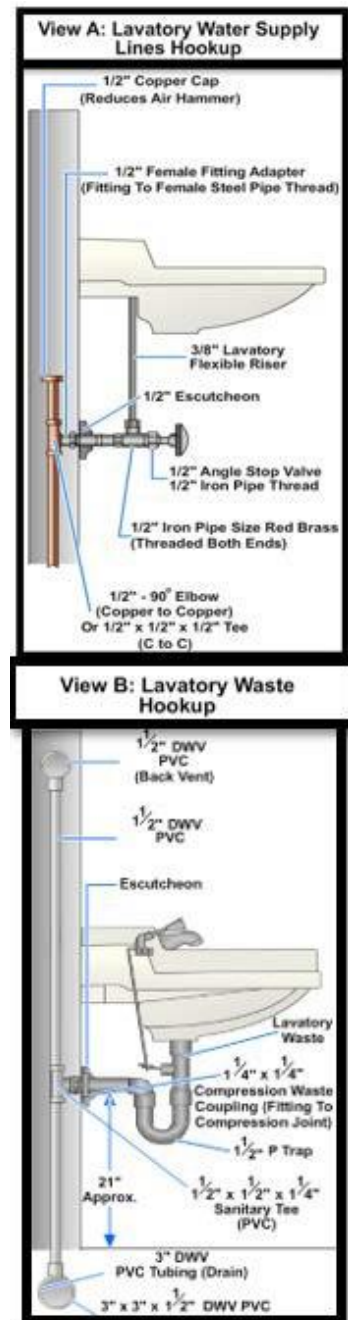
Figure 6-15 – Lavatory water supply and waste hookups.
