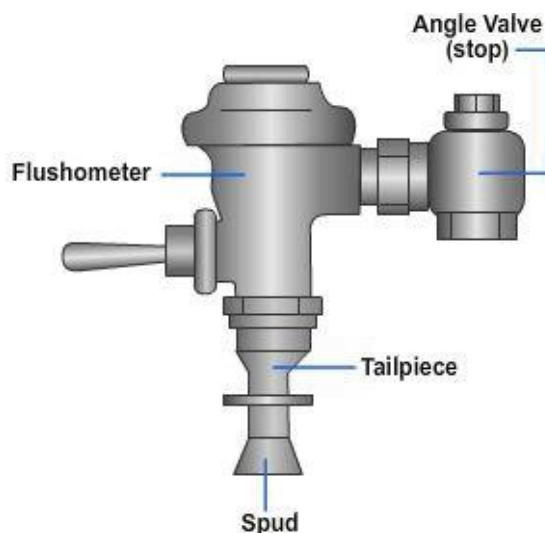
Figure 6-56 – Flushometer.
