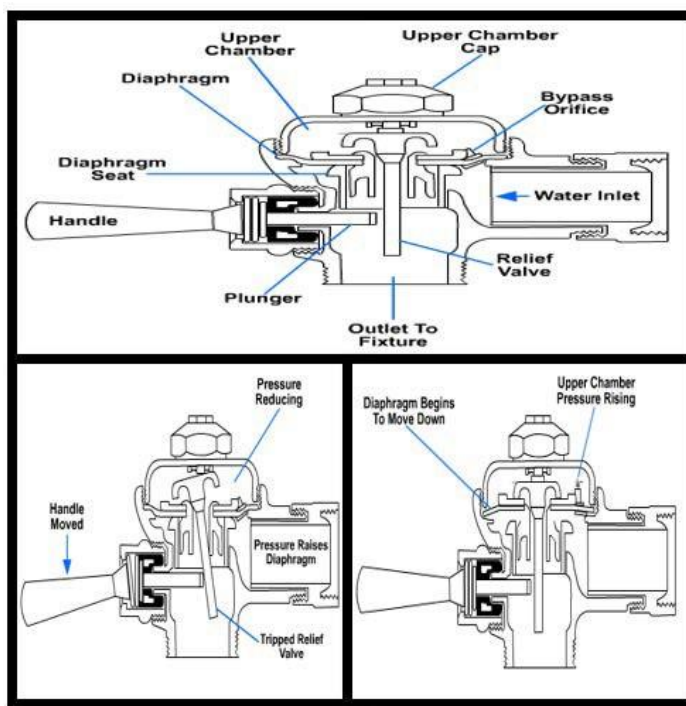
Figure 6-38 – Operation of diaphragm flushometer.
