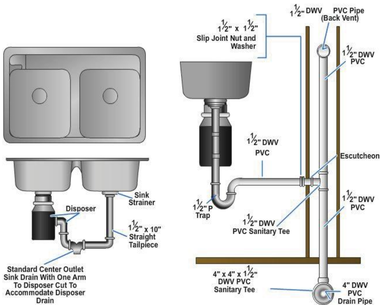
Figure 6-12 – Kitchen sink waste hookup.
