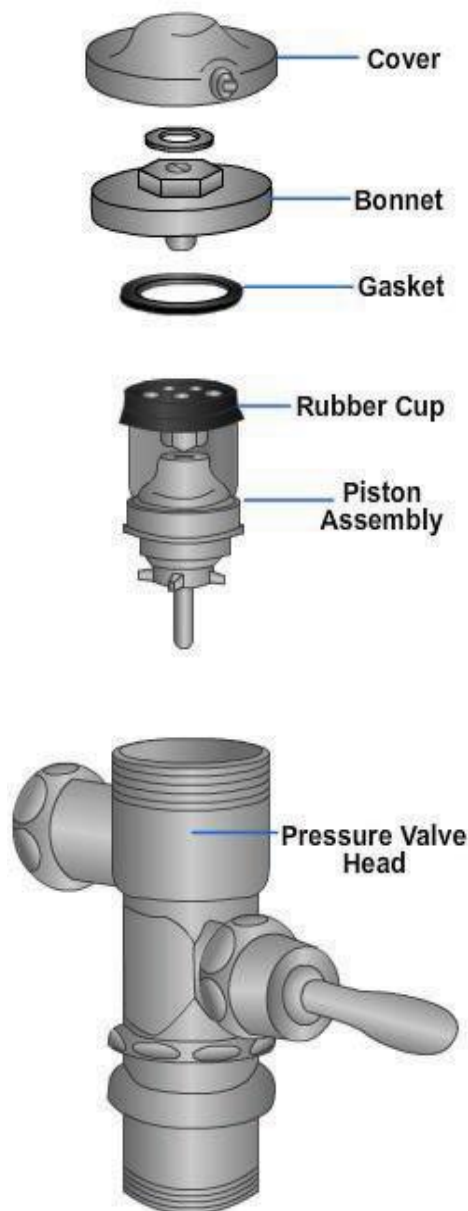
Figure 6-40 – Pressure valve head flushometer.
