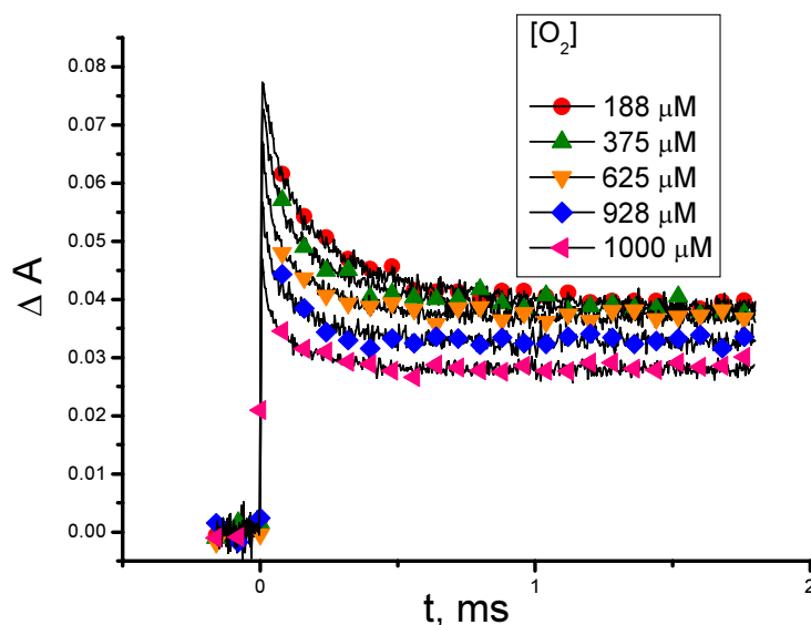
FIG. 12. Peroxylation reaction of \text{HO-CF}^\bullet at increasing \text{O}_2 concentrations, \lambda = 300 \text{ nm} , 5 \text{ cm} cell, dose = 11.0 \text{ Gy} .
