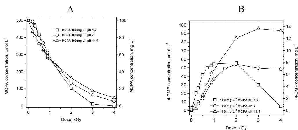
FIG. 9. (A) — decomposition of 100 ppm MCPA at different doses during \gamma irradiation at pH1.5 ( ), 7.0 (O) and 11.5 ( \Delta ). (B) — formation of 4-chloro-2-methylphenol at different doses during \gamma irradiation of 100 ppm MCPA at pH=1.5 ( ), 7.0 (O) and 11.5 ( \Delta ).
