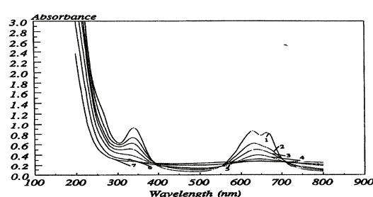
FIG. 2. Absorption spectra of unirradiated and irradiated RB15 aqueous solutions. Dye concentration: 50 ppm, [\text{H}_2\text{O}_2]=1.2 mM, Dose rate: 2.87 kGy/h, Dose (kGy): 0 (curve 1), 1 (Curve 2), 2 (curve 3), 3 (Curve 4), 5 (Curve 5), 7 (Curve 6), 9 (Curve 7).
