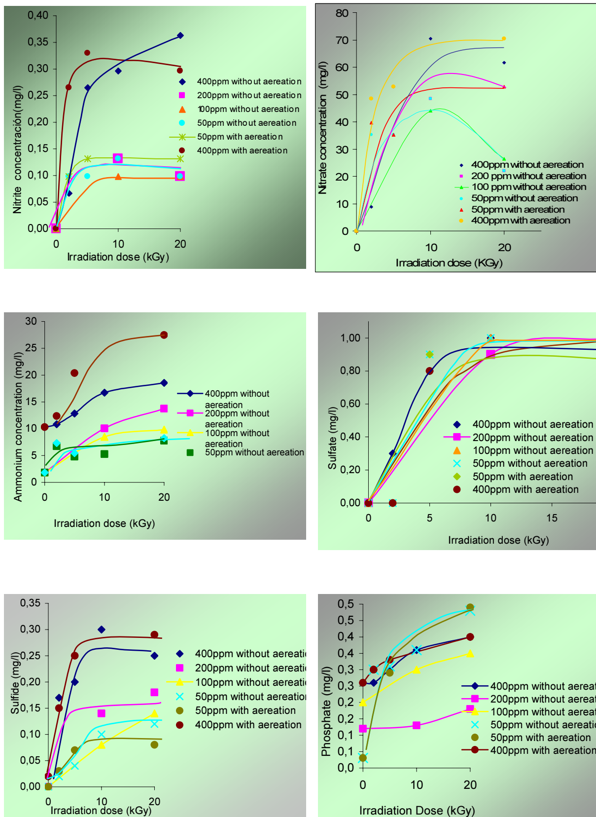
FIG. 3. Influence of electron beam on ion concentration of Diazinon pesticide, as a function of irradiation dose, with and without aeration.
