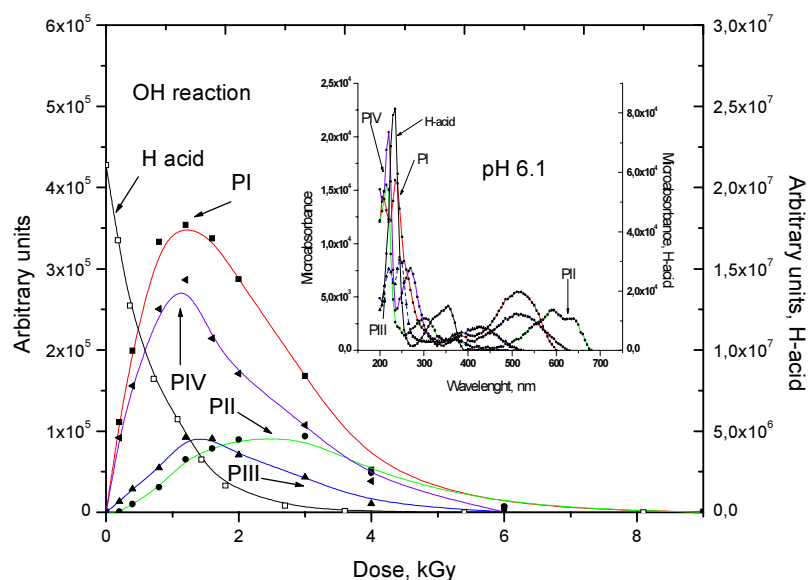
FIG. 10. Dose dependences of the absorbancies of the starting compound and the products formed in the reaction between \bullet OH radicals and I , c = 0.25 \text{ mmol dm}^{-3} . PI: maximum at 236 nm, t = 11.3 \text{ min} , PII: maximum at 592 nm, t = 15.8 \text{ min} , PIII: maximum at 334 nm, t = 16.5 \text{ min} , PIV: maximum at 240 nm, t = 21.5 \text{ min} , H-acid: maximum at 233 nm, t = 13.4 \text{ min} . The Inset shows the absorption spectra of the main compounds formed and that of the H-acid.
