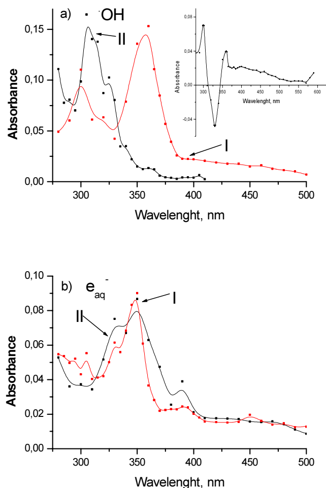
FIG. 13. Absorption spectra of the intermediate species formed in solution of I and II , respectively, 5 \mu\text{s} after the pulse. Spectra measured a , in N 2 O saturated system, b , in N 2 + 0.5 mol dm -3 tert-butanol containing system. 21 Gy/pulse, c = 0.1 \text{ mmol dm}^{-3} . Inset: uncorrected absorption spectrum taken in solution of I .
