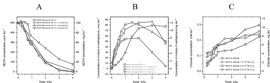
FIG. 15. Yield of decomposition of MCPA(A), formation of 4-chloro-2-methylphenol (B) and chloride (C) at different doses during \gamma irradiation of 100 ppm solution of MCPA without \text{H}_2\text{O}_2 ( ), in the presence of 1.2 mM \text{H}_2\text{O}_2 (O), 2.4 mM \text{H}_2\text{O}_2 ( \Delta ) and 4.8 mM \text{H}_2\text{O}_2 ( \nabla ).
