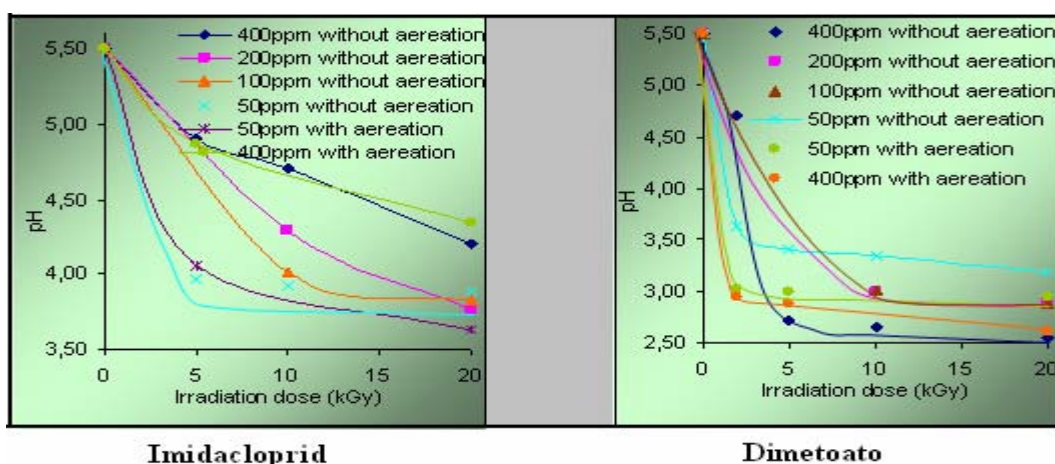
FIG. 2. Influence of electron beam on pH of Imidacloprid and dimetoato pesticides to different concentrations of pesticides as a function of irradiation dose, with and without aeration.
