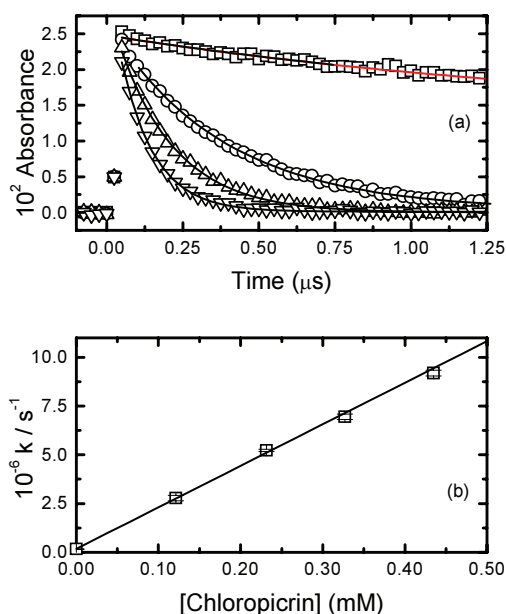
FIG. 2. a) Typical kinetic decay profiles obtained for the hydrated electron absorbance at 700 nm for the electron pulse irradiated aqueous solution at natural pH and 20^\circ \text{C} containing zero ( \square ), 1.12 \times 10^{-4} (O), 2.32 \times 10^{-4} ( \Delta ), and 4.35 \times 10^{-4} (V) M Chloropicrin, respectively. Curves shown are the average of 15 individual pulses. Solid lines correspond to rate constant fitting with the pseudo-first-order values of 1.71 \times 10^5 , 2.64 \times 10^6 , 5.26 \times 10^6 , and 9.30 \times 10^6 \text{ s}^{-1} , respectively. (b) Second-order rate constant determination for the reaction of the hydrated electron with Chloropicrin. Single-point error bars are one standard deviation, as determined from the average of at least three kinetic traces. Solid line corresponds to weighted linear fit, giving k = (2.13 \pm 0.03) \times 10^{10} \text{ M}^{-1} \text{ s}^{-1} .
