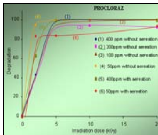
FIG. 1. Influence of electron beam on degradation percentage of Diazinon, imidacloprid, dimetoato, carbofuran, metiocarb and prochloraz pesticides, as a function of irradiation dose to different concentrations of pesticide, with and without aeration.
