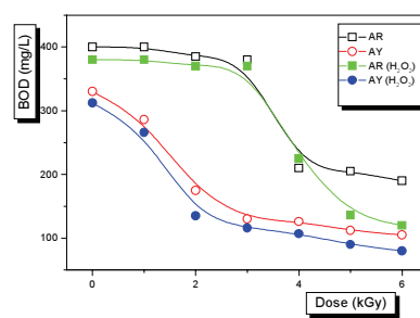
FIG. 19. BOD values for AR and AY dye solutions gamma irradiation. [\text{AR}] = [\text{AY}] = 0.200 \text{ g/L} , [\text{H}_2\text{O}_2] = 1.2 \text{ mM} . Dose rate: 0.14 kGy/h. (Solid symbols are used for AR and AY concentrations containing \text{H}_2\text{O}_2 .)
