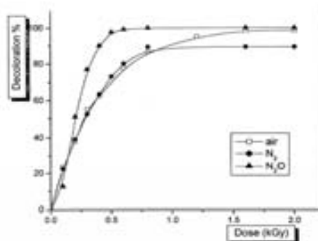
FIG. 12. Effect of additives on degree of decoloration for RB5 aqueous solutions. [Dye]=50ppm.
