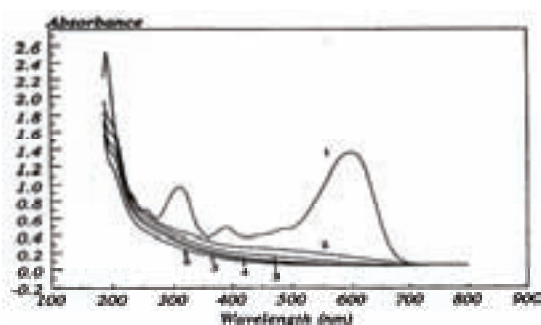
FIG. 3. Absorption spectra of unirradiated and irradiated RB5 aqueous solutions. Dye concentration: 50 ppm, Dose rate: 2.87 kGy/h, Dose (kGy): 0 (curve 1), 1 (Curve 2), 2 (curve 3), 3 (Curve 4), 4 (Curve 5), 5 (Curve 6).
