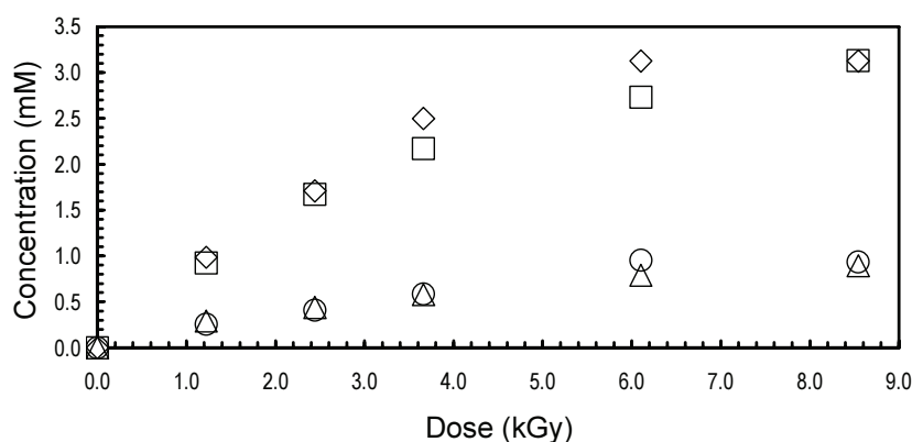
FIG. 3. Comparison of experimental (◇) and modeled (○) results for ^{60}\text{Co} irradiated [\text{TCNM}]_0 = 1.13 \text{ mM} .
