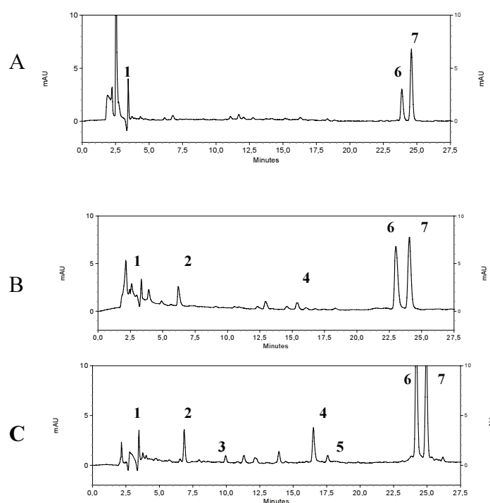
FIG. 8. Effect of pH of irradiated solutions on RP-HPLC chromatograms for 100 ppm solution of MCPA obtained after \gamma irradiation with 3 kGy dose. A- pH 1.5, B- pH 7.0, C- pH 11.5. Peak assignments: (1) hydroquinone, (2) catechol, (3) phenol, (4) o-cresol, (5) 4-chlorophenol, (6) MCPA, (7) 4-chloro-2-methylphenol.
