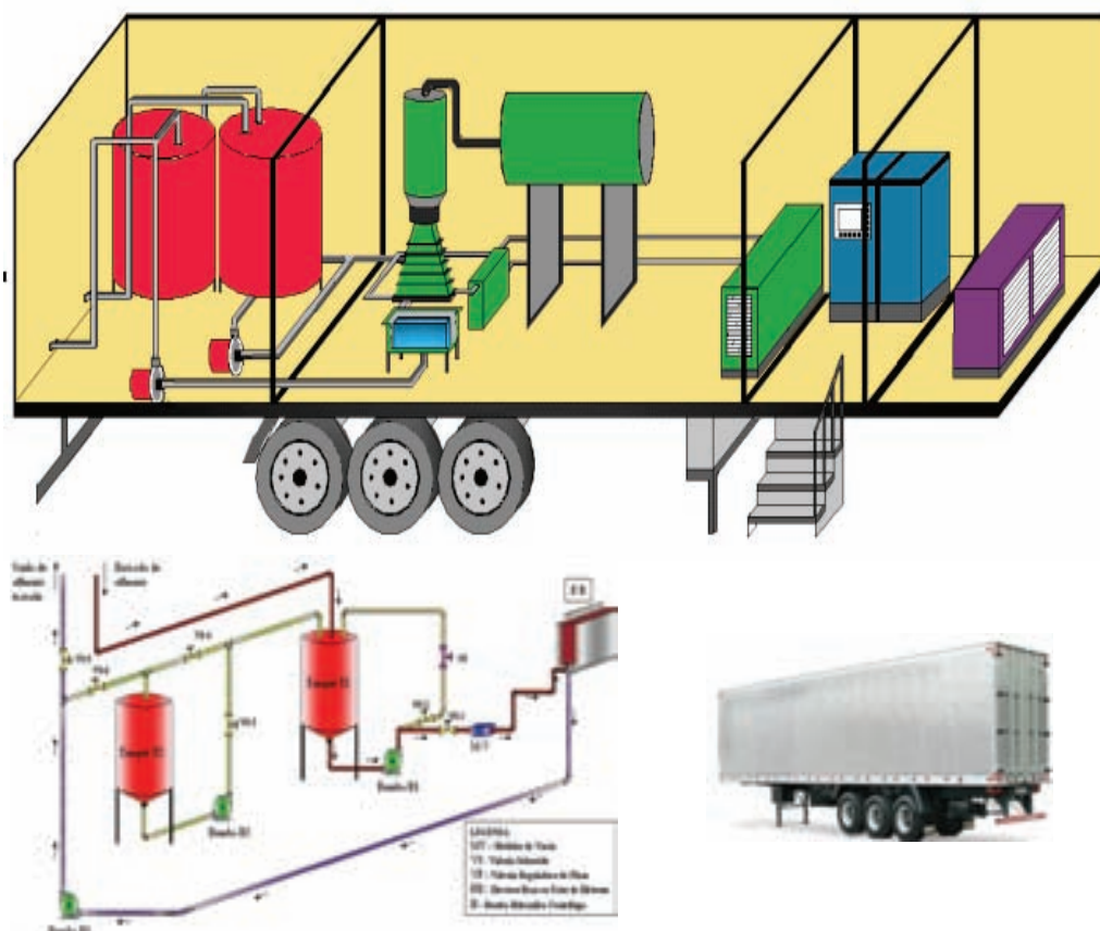
FIG. 8. Mobile irradiation facility.
