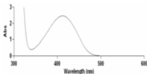
FIG. 14. Light-Absorption spectra of formaldehyde complex. \lambda_{max} = 412 \text{ nm}
