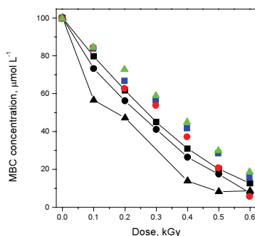
FIG. 20. Comparison of experimental data with kinetic modeling for yield of degradation of carbendazim at initial concentration 100 \mu\text{M} in aerated solution of different pH. Data for pH3 experimental (■) and calculated (□), data for pH7 experimental (●) and calculated (○), data for pH10 experimental (▲) and calculated (△).
