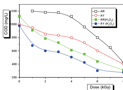
FIG. 18. COD values for AR and AY dye solutions gamma irradiation. [\text{AR}] = [\text{AY}] = 0.200 \text{ g/L} , [\text{H}_2\text{O}_2] = 1.2 \text{ mM} . Dose rate: 0.14 kGy/h. (Solid symbols are used for AR and AY concentrations containing \text{H}_2\text{O}_2 .)
