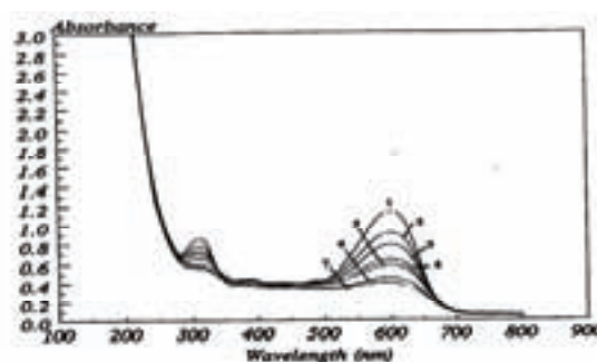
FIG. 4. Absorption spectra of unirradiated and irradiated RB5 aqueous solutions. Dye concentration: 50 ppm, [\text{H}_2\text{O}_2]=1.2 mM, Dose rate: 2.87 kGy/h, Dose (kGy): 0 (curve 1), 0.4 (Curve 5), 0.5 (Curve 6), 0.6 (Curve 7).
