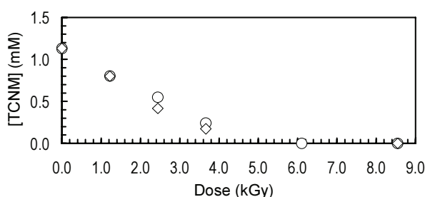
FIG. 3. Comparison of experimental (◇) and modeled (○) results for ^{60}\text{Co} irradiated [\text{TCNM}]_0 = 1.13 \text{ mM} .
