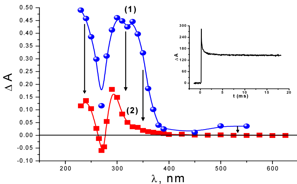
FIG. 10. (1): observed spectrum 9 \mu\text{s} after the pulse, dose = 11.5 Gy. (2 : observed spectrum 9 ms after the pulse, dose = 62.4 Gy. [\text{CF}] = 100 \mu\text{M} , 5 cm cell. Inset: decay of \text{CF}^\bullet in the absence of oxygen at 300 nm.
