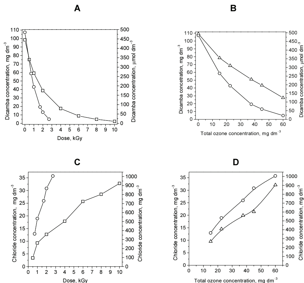
FIG. 13. The effect of ozone on EB degradation of dicamba (A,B) and of chloride release from 110 ppm dicamba solution (C,D) carried out in groundwater matrix, EB irradiation ( \square ) EB/O 3 (O) ozonation ( \Delta ).
