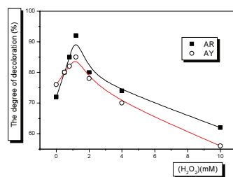
FIG. 17. Effect of hydrogen peroxide on the degree of decoloration. Irradiation dose: 3.0 kGy, [AR]=[AY]=0.200 g/L, Dose rate: 0.14 kGy/h.
