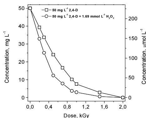
FIG. 14. Decomposition of 2,4-D at different doses during \gamma -irradiation of 50 \text{ mg L}^{-1} without ( ) and with 1.7 mM of \text{H}_2\text{O}_2 .
