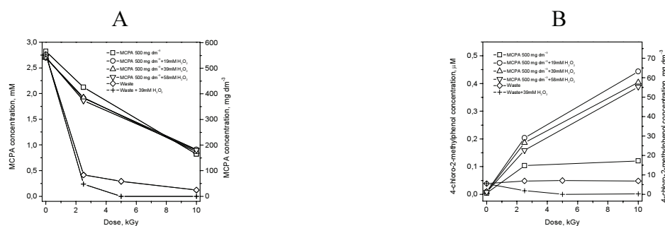
FIG. 25. Decomposition of MCPA (A) and formation of 4-chloro-2-methylphenol (B) during irradiation of solution 500 mg mg dm -3 MCPA ( ), 500 mg mg dm -3 MCPA with 19 mM H_2O_2 (O), 500 mg mg dm -3 MCPA with 39 mM H_2O_2 ( \Delta ), 500 mg dm -3 1 MCPA with 58 mM H_2O_2 ( \nabla ), waste ( \diamond ), waste with 39 mM H_2O_2 (+).
