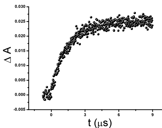
FIG. 8. Product build up of the reaction OH + CF at 300 nm, 5 cm cell.
