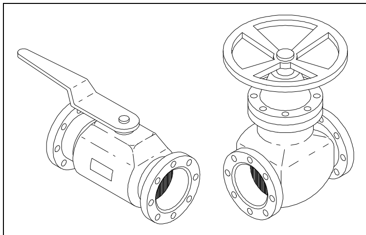
Figure 30 Fixed Handwheel
