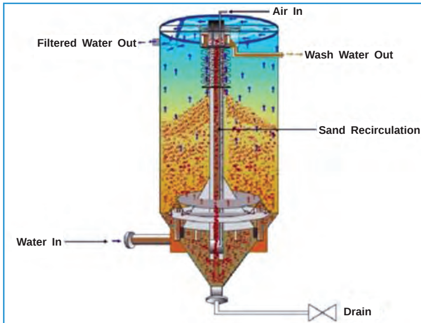
Fig 3.12 – Cross section drawing of continuous sand filter
