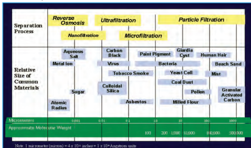
Fig 7.1 - Filtration spectrum
