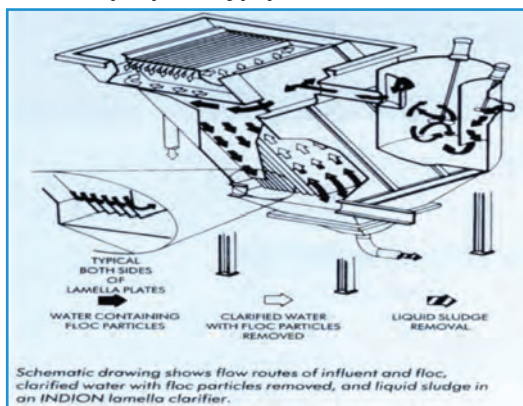
Fig 3.7 - Cross section drawing of lamella clarifier
