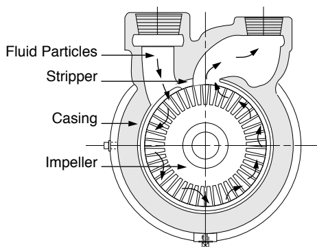
FIGURE 7. Turbine Pump
