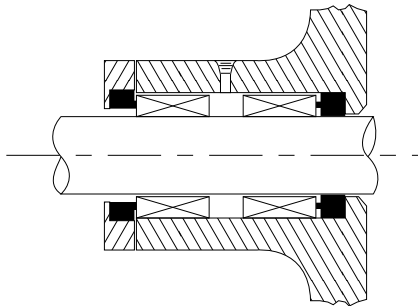
FIGURE 42. Double Seal
