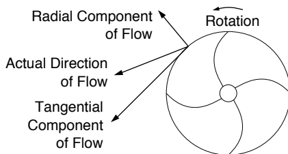
FIGURE 25. Liquid Flow Direction
