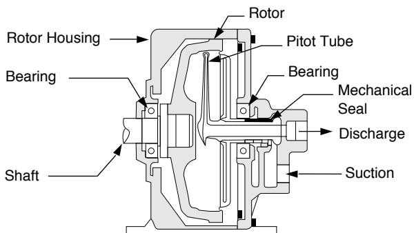
FIGURE 10. Rotating Case Pump
