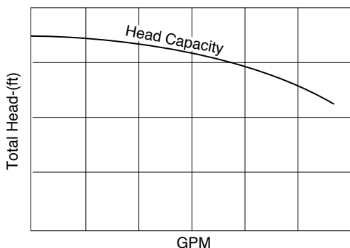
FIGURE 45. Head-Capacity Curve
