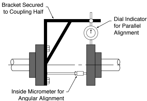
FIGURE 81. Method of Checking Alignment on a Spacer Coupling
