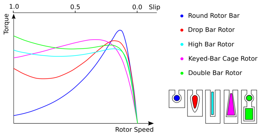
Figure 8: Influence of the shape of rotor bars (5), (6)
