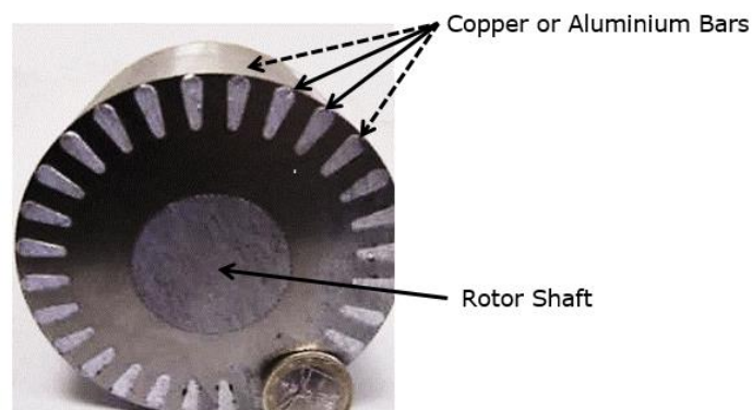
Figure 5: Cross section of a squirrel cage rotor with drop shaped bars (4)
