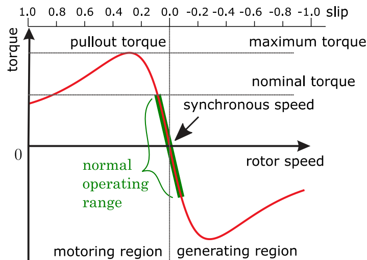
Figure 6: Torque-vs.-speed diagram of the IM (5)
