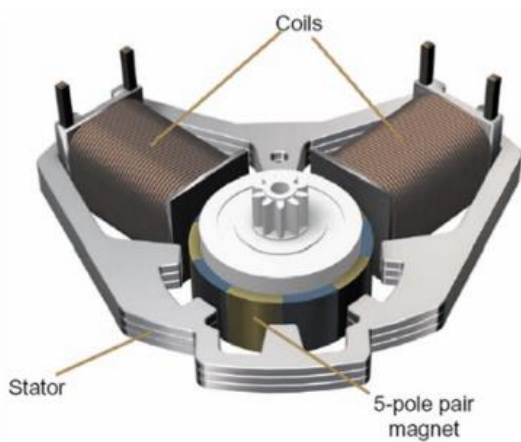
Figure 64: Coils of the example permanent magnet stepper motor (33)
