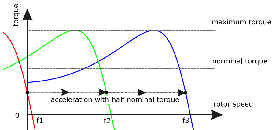
Figure 11: Torque for V/f control (5)
