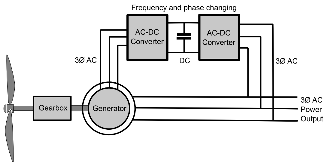
Figure 17: Doubly-fed induction generator connected to a wind turbine (11)
