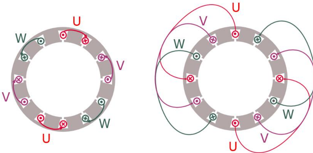
Figure 21: Concentrated (left) vs. distributed (right) winding system
