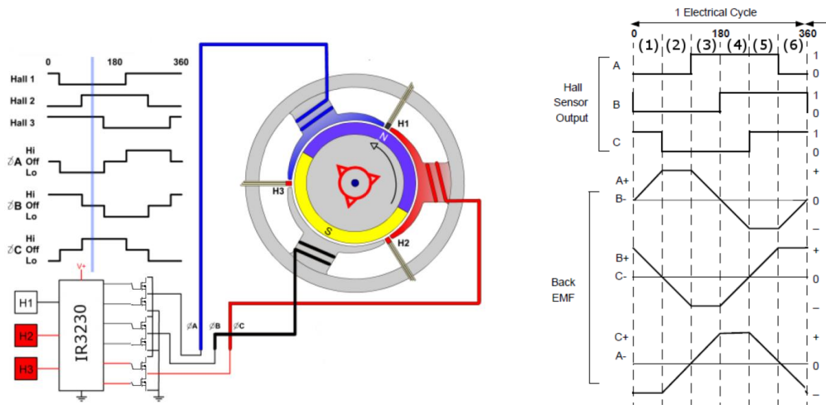
Figure 44: Control of a BLDC motor with Hall sensors (left), exemplary hall sensor output and back emf waveforms (right) (25)
