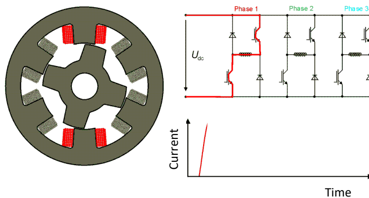
Figure 51: Current flow of the magnetization state (5)
