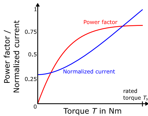
Figure 14: Normalized current and power factor over torque (5)
