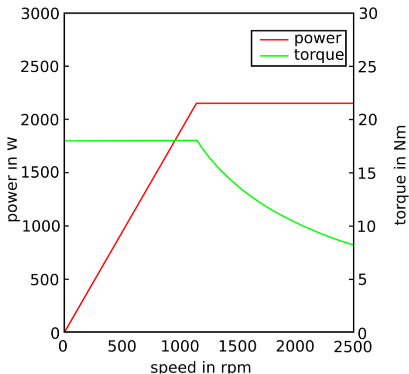
Figure 48: Torque and power over-speed curve of a SRM (7; 5)
