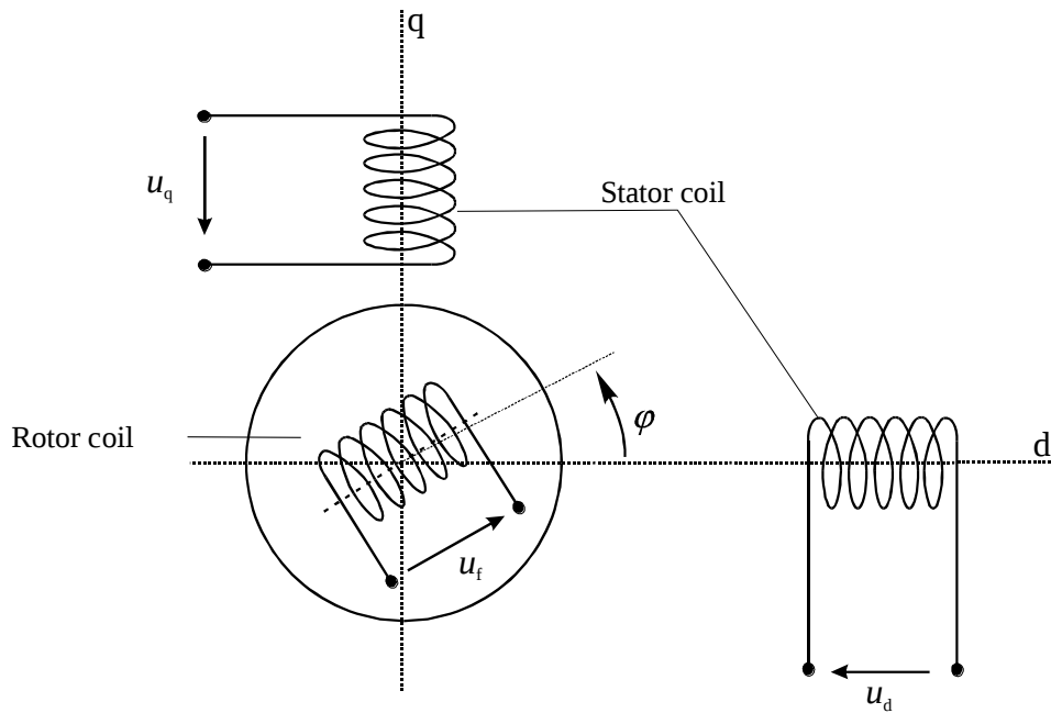
Figure 87: Resolver for absolute position measurement (5)
