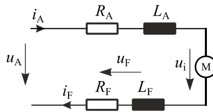
Figure 34: Series wound DC machine (5)
