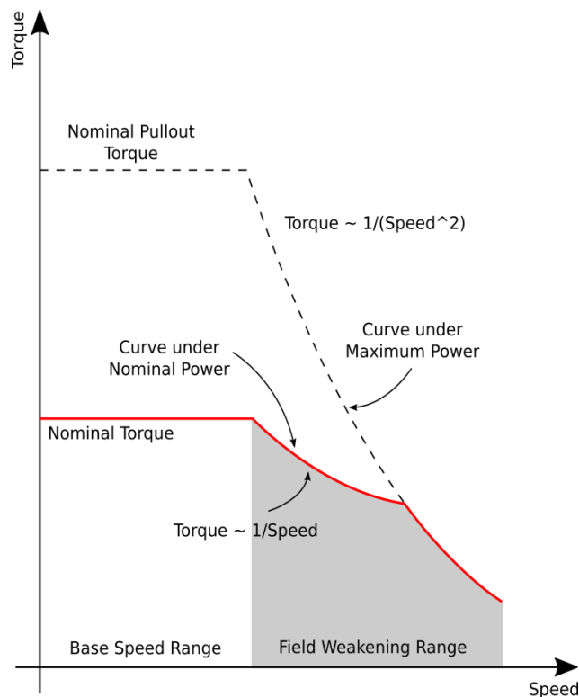
Figure 13: Operating range of the induction motor (5)
