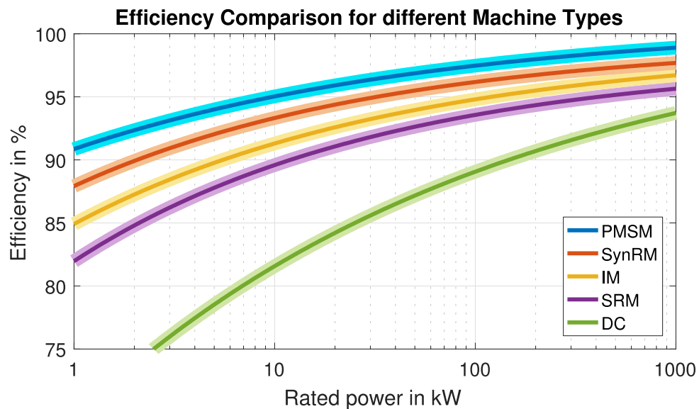
Figure 100: Example comparison of efficiency for different machines (60), (61)
