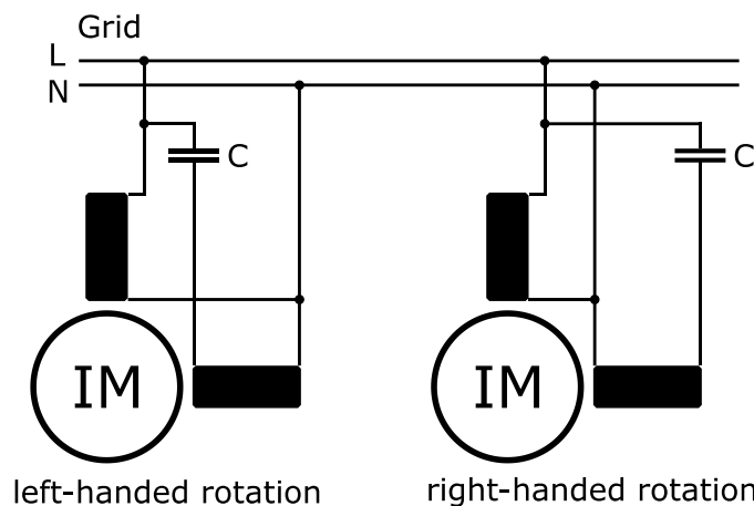
Figure 18: One-phase induction motor as capacitor motor (5)
