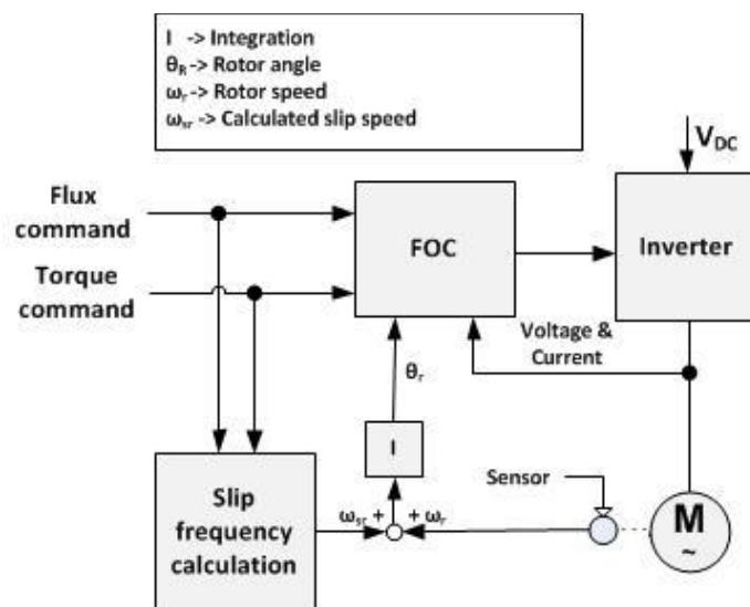
Figure 93: Block diagram of indirect field-oriented control (IFOC) (49)
