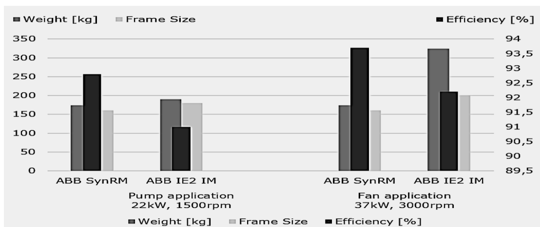
Figure 26: Comparison of efficiency and power density aspects for synchronous reluctance vs. induction machines (data originating from ABB (17))
