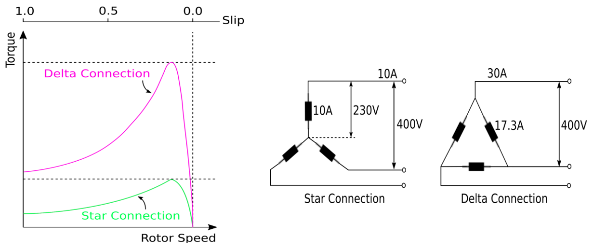
Figure 9: Star- and delta-connected IM (5)
