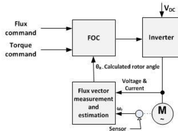
Figure 94: Block diagram of direct field-oriented control (DFOC) (50)
