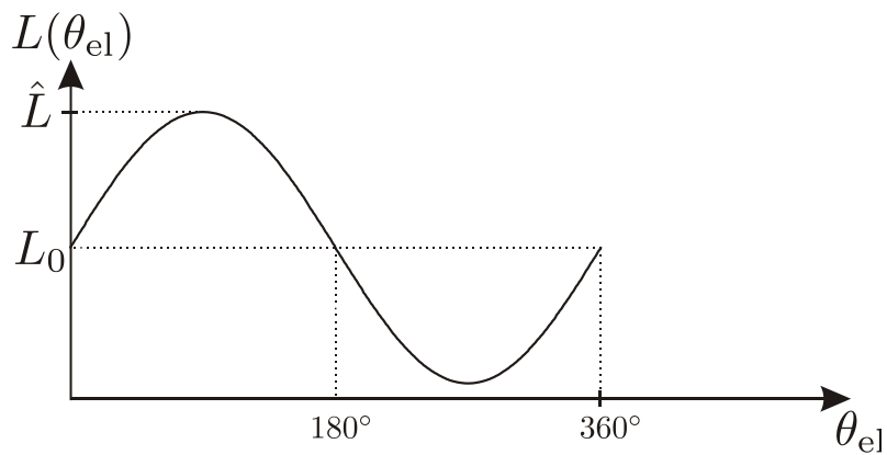
Figure 89: VR-Resolver: Change of inductance as function of the rotor position (5)
