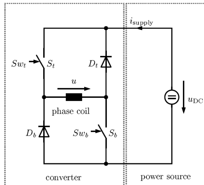
Figure 50: SR drive with asymmetric half-bridge converter topology (7; 5)
