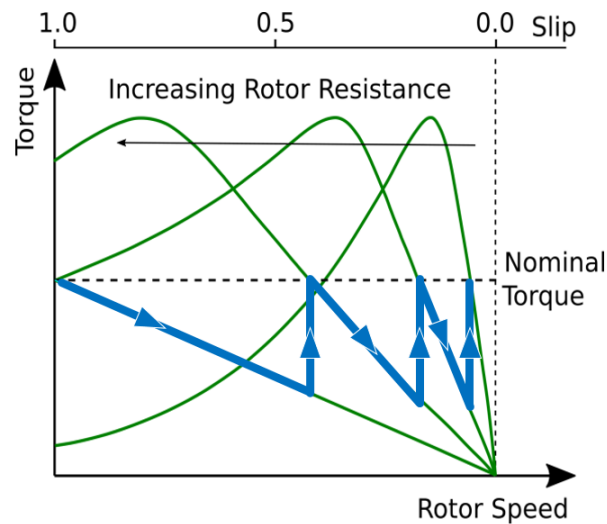
Figure 7: Influence of the rotor resistance (5)
