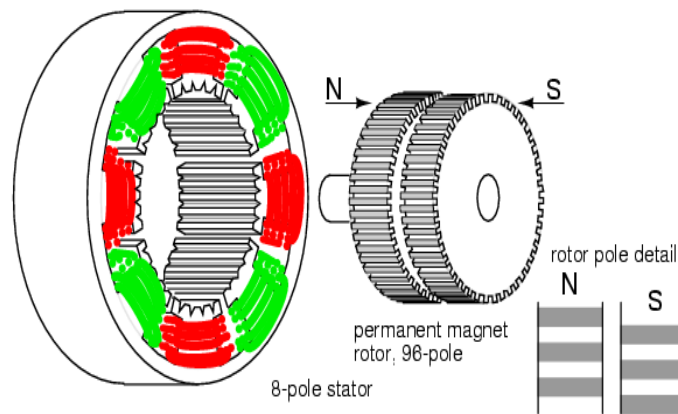
Figure 69: Hybrid synchronous stepper motor (31)
