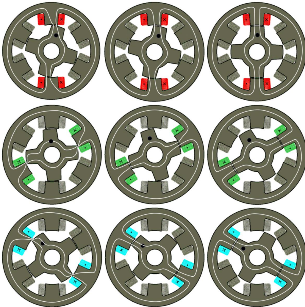
Figure 47: Continuous rotation of switched reluctance motors (5)
