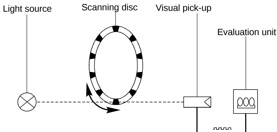
Figure 84: Optical incremental position encoder (5)
