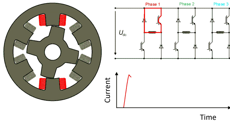
Figure 52: Current flow of the free-wheeling state (5)
