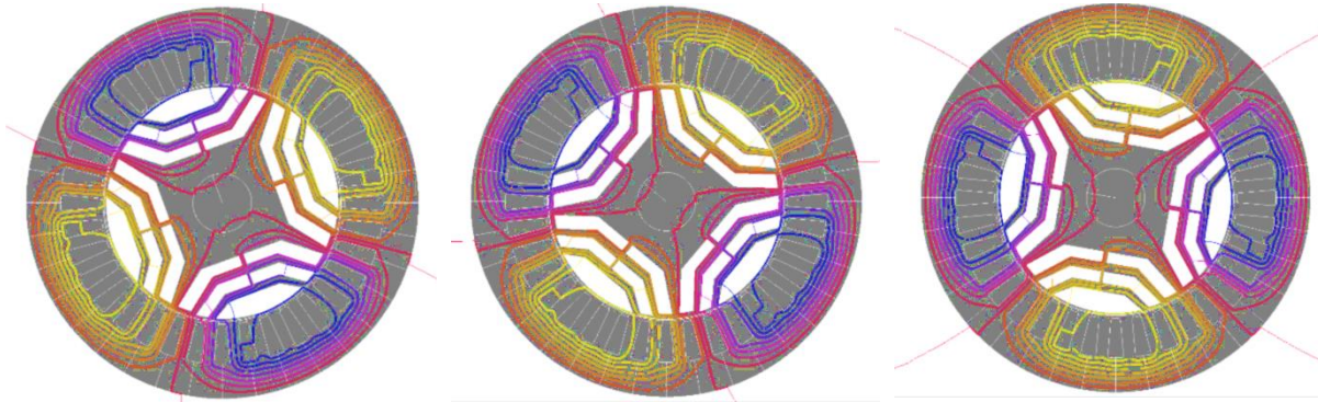
Figure 25: Magnetic flux paths within the synchronous reluctance machine with anti-clockwise rotation (5)
