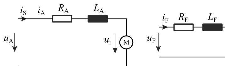
Figure 32: Separately excited DC machine (5)
