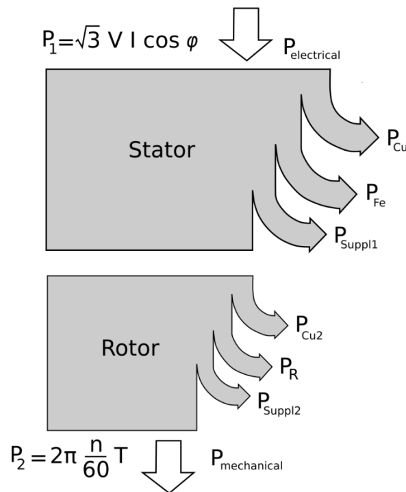
Figure 96: Breakdown example of losses in an electric machine, e.g. induction machine (5) (53)
