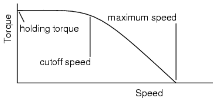
Figure 74: Speed torque characteristics (31)
