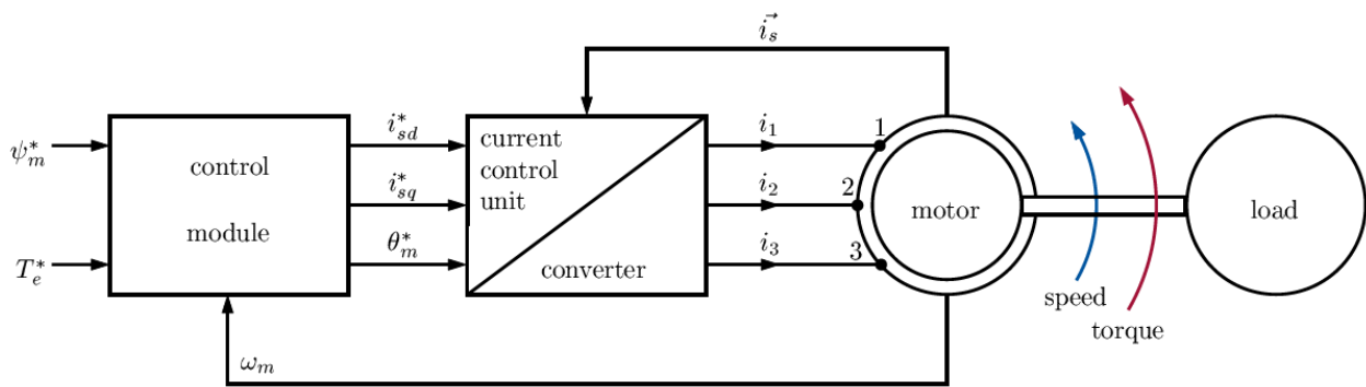
Figure 92: Field-oriented control drive structure (7)
