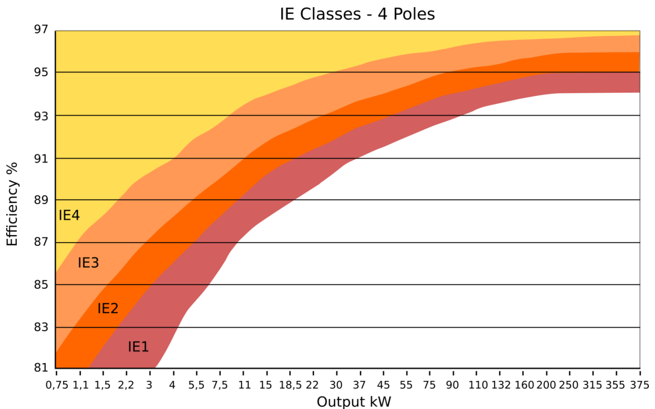
Figure 98: IE efficiency classes for 4-pole (2 pole pairs) motors at 50 Hz (5) (57)
