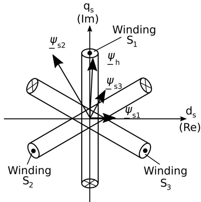
Figure 82: Flux linkage of a three-phase system (5)
