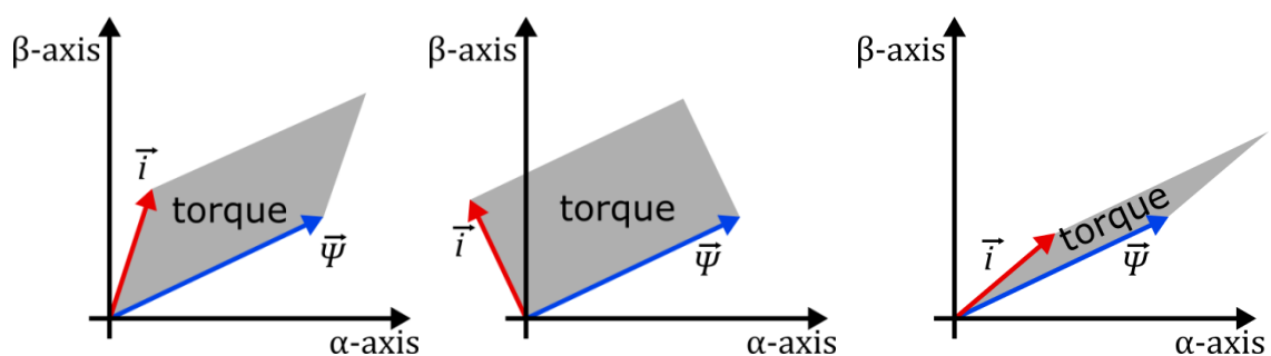
Figure 79: Relationship between current / flux linkage space vectors and torque (5)
