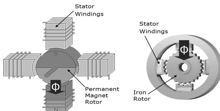
Figure 60: Function overview of permanent magnet [left] (29) and variable reluctance stepper motor [right] (30)
