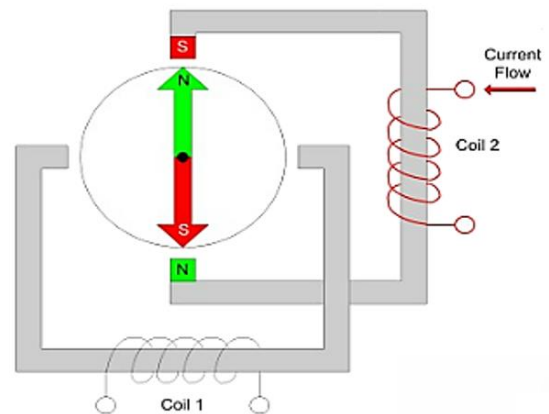
Figure 65: Position hold by current in two phases (33)
