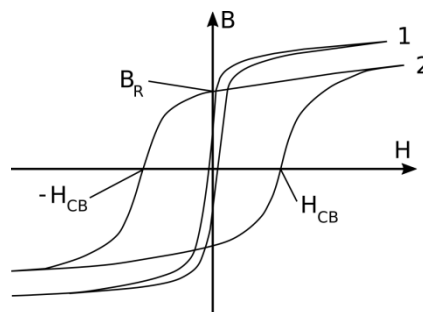
Figure 97: B(H)-characteristic of magnetic materials (5) (55) 1 = soft-magnetic material, e.g. iron 2 = hard-magnetic material, e.g. permanent magnets
