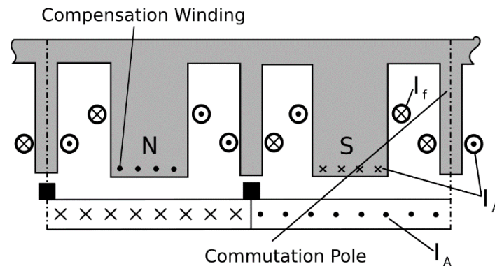
Figure 30: Compensation windings and commutation pole of a separately excited DC machine (5)
