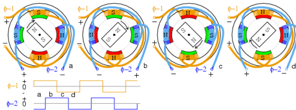
Figure 67: Simplified permanent magnet stepper in full-step drive (31)
