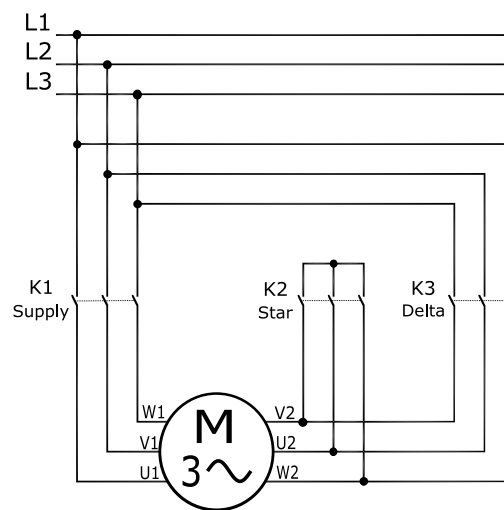
Figure 10: Star-Delta-Switching using contactors (5)
