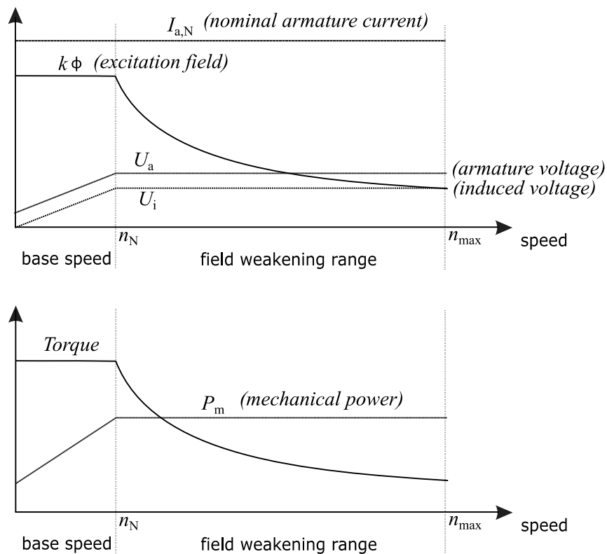
Figure 37: Operating limits of the separately excited DC machine (5)
