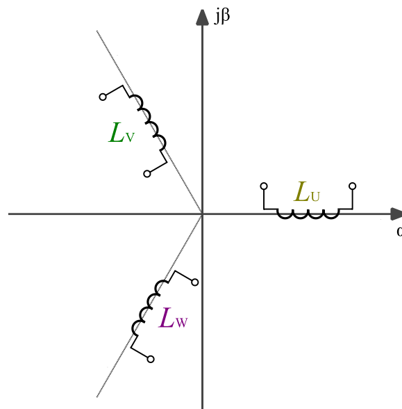
Figure 90: Arrangement of the \alpha\beta -coordinate system (48)
