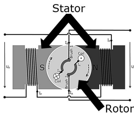
Figure 29: Schematic representation of an electrically excited DC machine (here: "separately excited")
