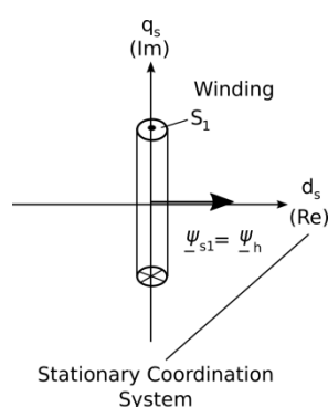
Figure 81: Producing flux linkage with one winding (5)
