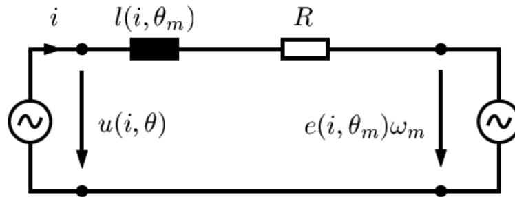
Figure 49: Equivalent circuit of one phase of a switched reluctance machine (7)
