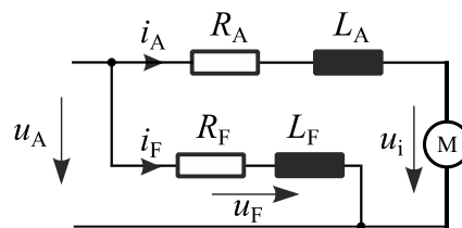
Figure 36: Parallel wound DC machine (5)
