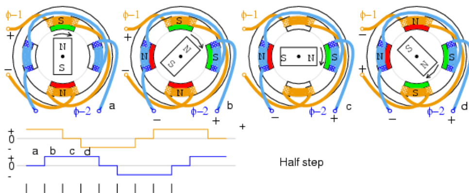
Figure 68: Simplified permanent stepper motor in half step drive (31)
