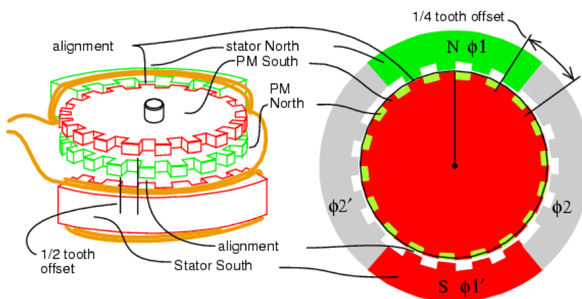
Figure 70: Simplification of hybrid stepper motor (31)
