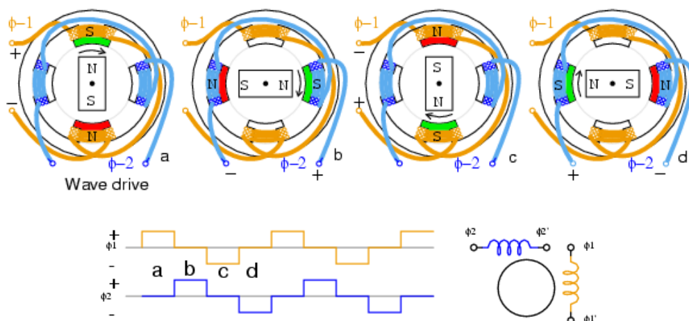
Figure 66: Simplified permanent magnet stepper in wave drive (31)
