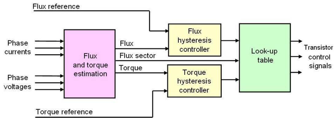
Figure 95: Block diagram of direct torque control (DTC) (52)
