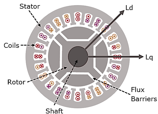
Figure 24: Cross section of a synchronous reluctance machine by ABB (15) (left), and a schematic cross section (right)
