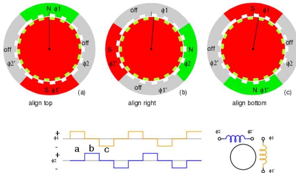
Figure 71: Hybrid stepper motor rotation sequence (31)
