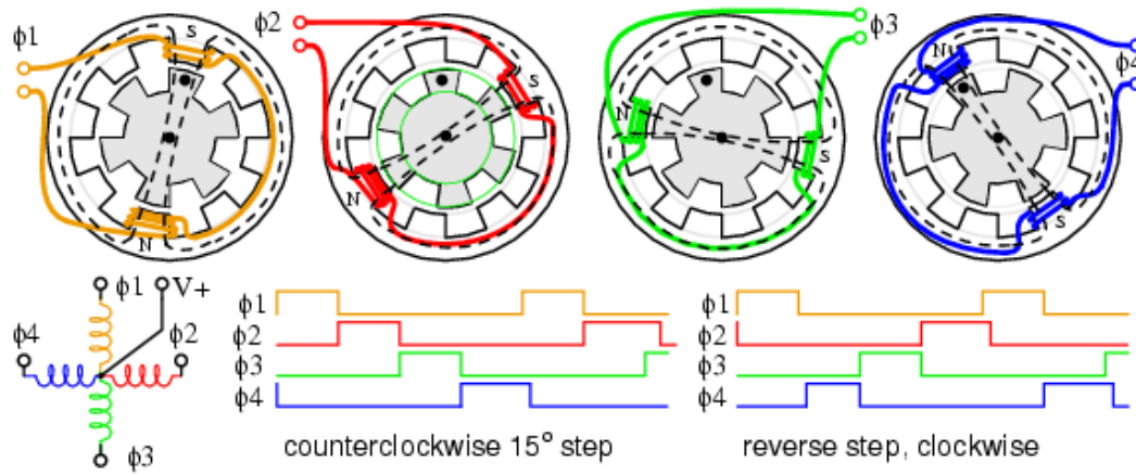
Figure 62: Stepping sequence for variable reluctance stepper (31)
