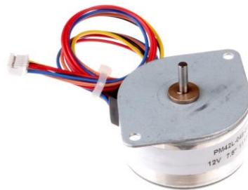
Figure 63: Example of a permanent magnet stepper motor (32)
