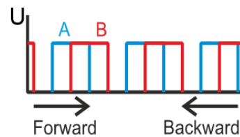
Figure 86: Magnetic incremental position encoder (electrical pulses) (5)
