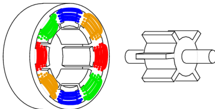
Figure 61: Variable reluctance stepper motor (31)
