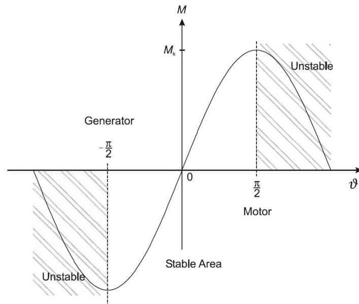
Figure 22: Torque as a function of load angle at constant voltage operation (5)
