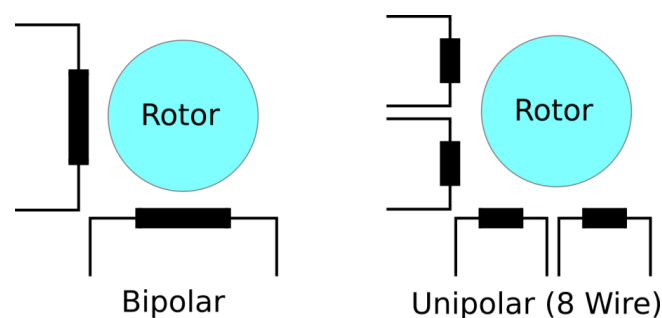
Figure 72: Bipolar and unipolar winding arrangements (34)
