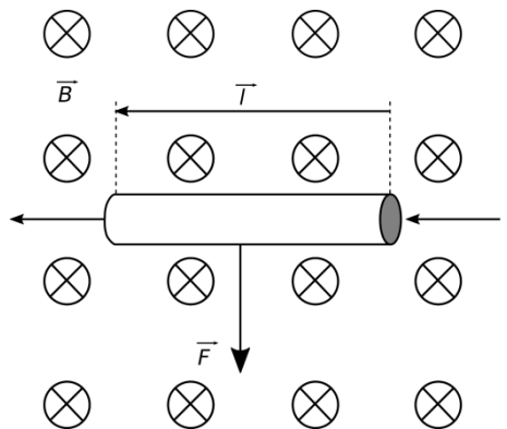
Figure 77: Lorentz force on a current carrying conductor in a magnetic field (5)
