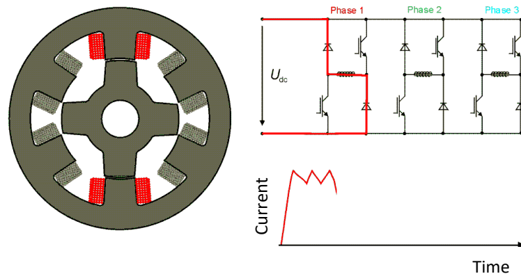
Figure 53: Current flow of the de-magnetization state (5)
