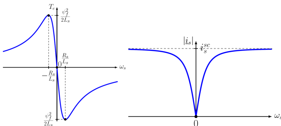
Figure 23: Short circuit torque and current compared to rotor speed (5) (7)
