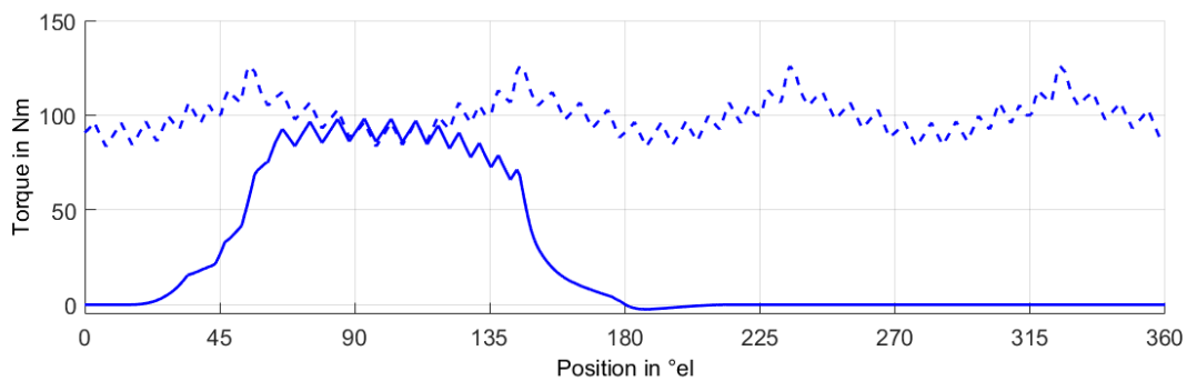
Figure 58: Torque production of a four phase SRM (5)
