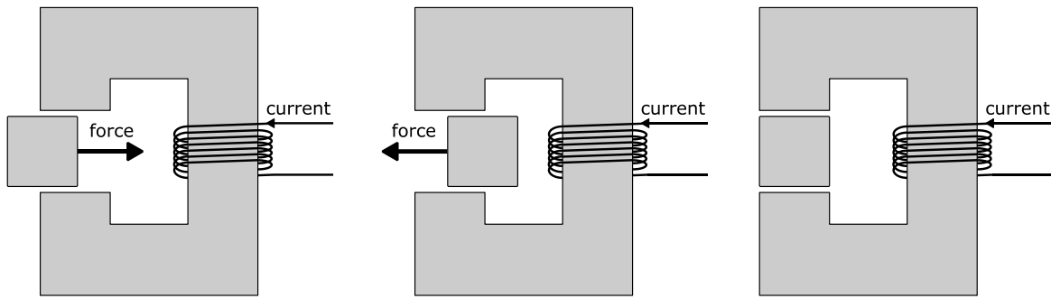
Figure 80: Reluctance force in a magnetic circuit (5)
