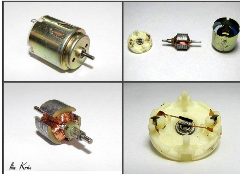
Figure 27: Mechanical structure of permanent magnet externally excited DC motor; clockwise: fully packaged, decomposed, brushes and rotor (18)
