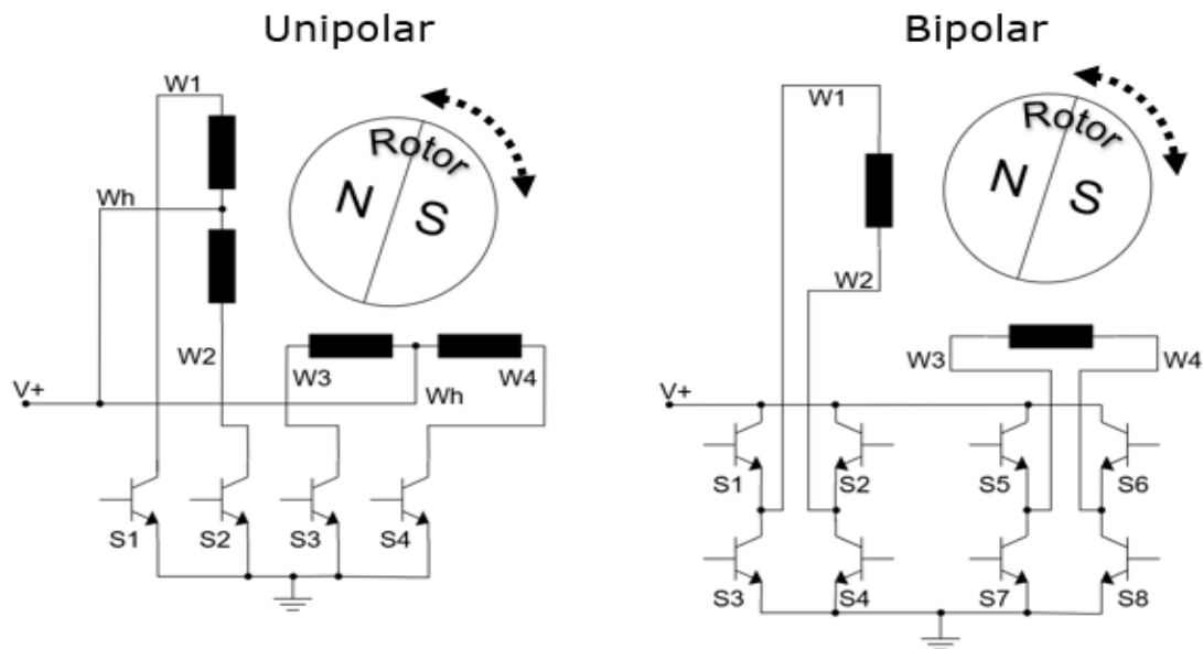
Figure 73: Switches for bipolar and unipolar motor (36)
