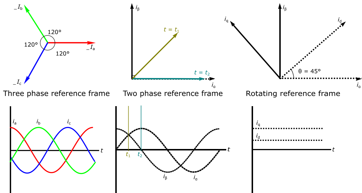
Figure 91: Transformations of a three-phase system (5)
