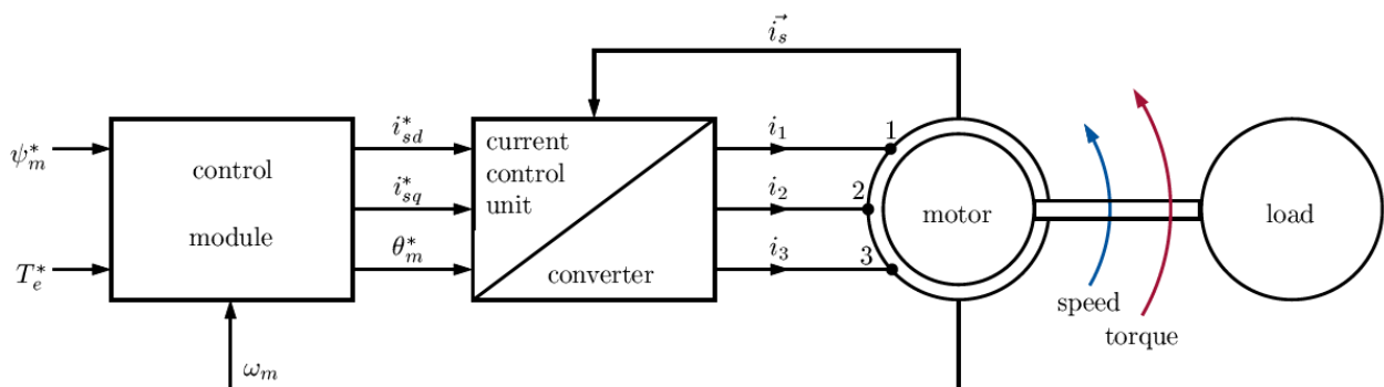
Figure 12: Field-oriented control drive structure (5) (7)
