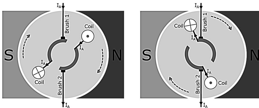
Figure 28: Simplified cross section of a permanent magnet DC machine with two possible commutator positions, right after (left) and shortly before (right) next commutation
