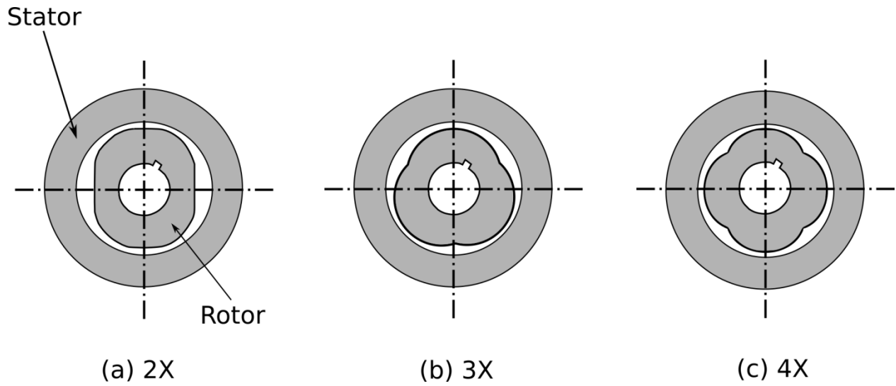
Figure 88: Examples of rotor shapes of the VR-type resolvers (5)
