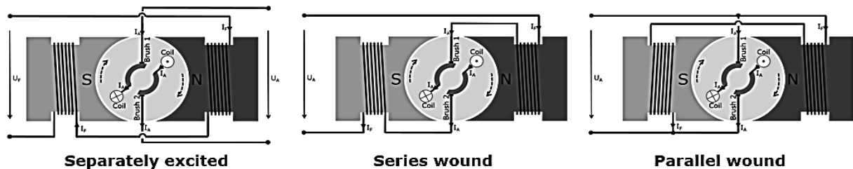
Figure 31: Overview of the three different DC-motor types
