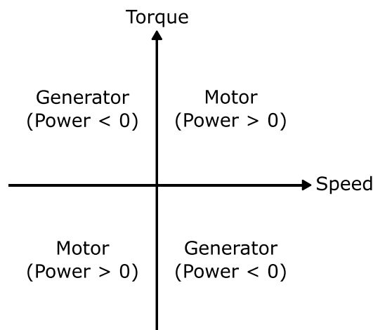
Figure 76: Operation quadrants of electrical drives (5)
