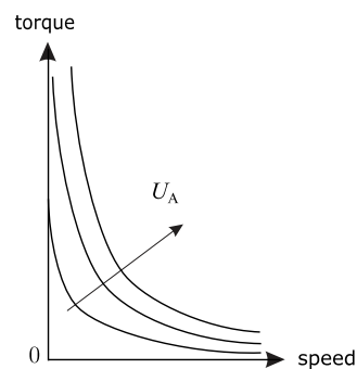
Figure 35: Torque-speed characteristic curve of the series wound machine (5)
