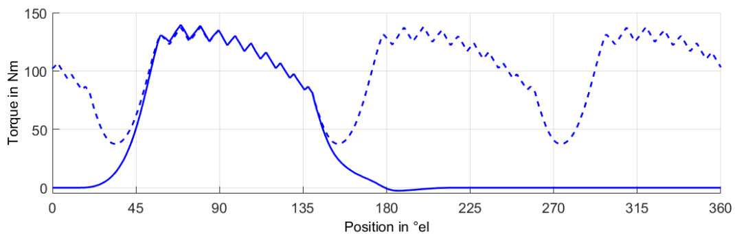
Figure 57: Torque production of a three-phase SRM (5)
