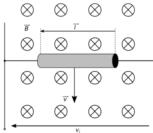
Figure 83: Generation of an induced voltage (5)
