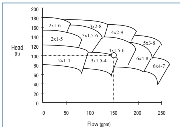
Figure 11. Family of Pump Performance Curves
