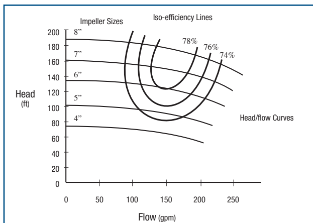
Figure 12. Performance Curves for Different Impeller Sizes
