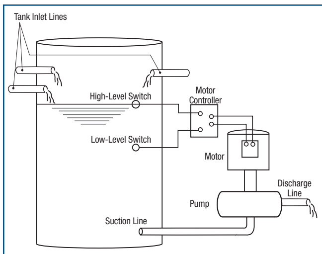
Figure 16. Typical Tank Level Control
