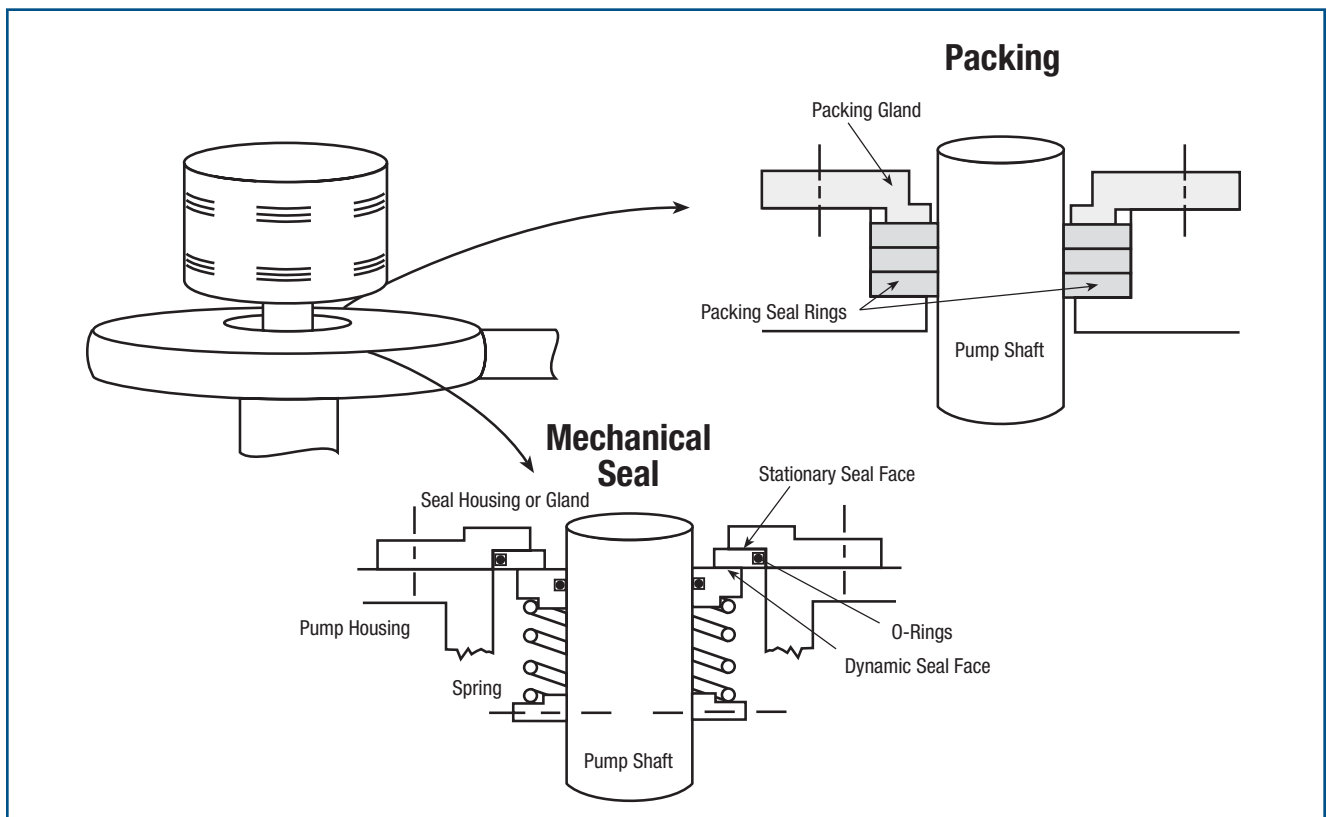
Figure 6. Two Types of Sealing Methods: Packing and Mechanical Seals
