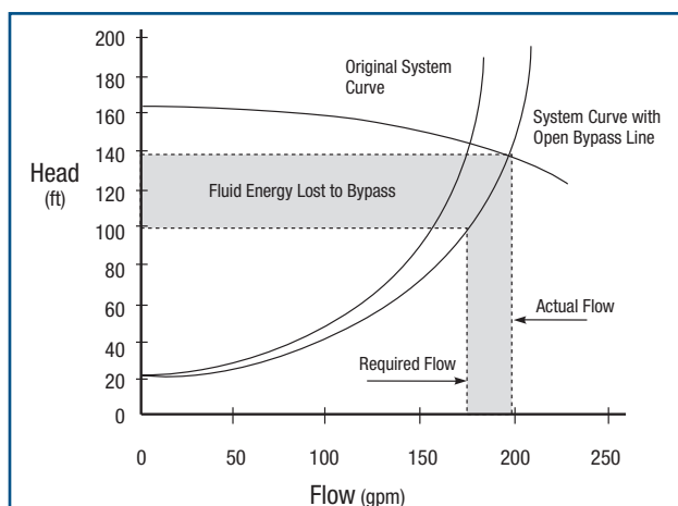
Figure 19. Power Lost through a Bypass Line
