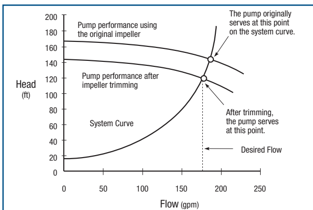
Figure 17. Effect of Impeller Trimming on Pump Performance
