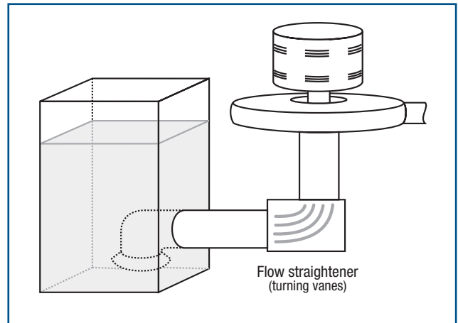
Figure 8. Flow Straighteners
