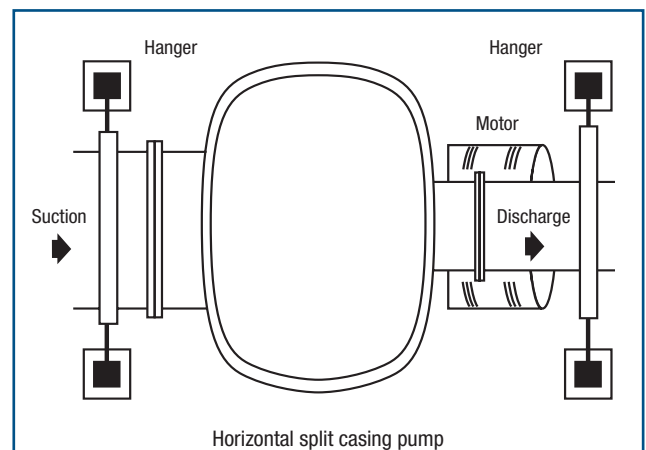
Figure 9. Proper Support of Suction and Discharge Piping
