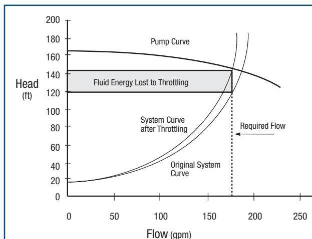
Figure 20. Fluid Power Lost across a Throttle Valve
