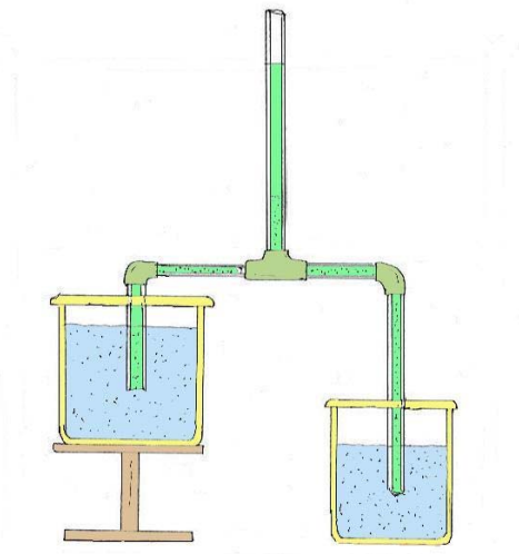
PASCAL'S SIPHON
