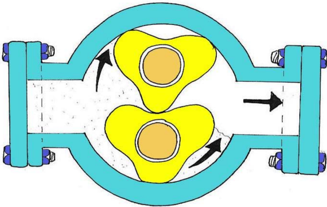
LOBE PUMP
