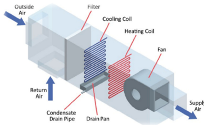
Figure 8. Structure of AHU condensate collection system
