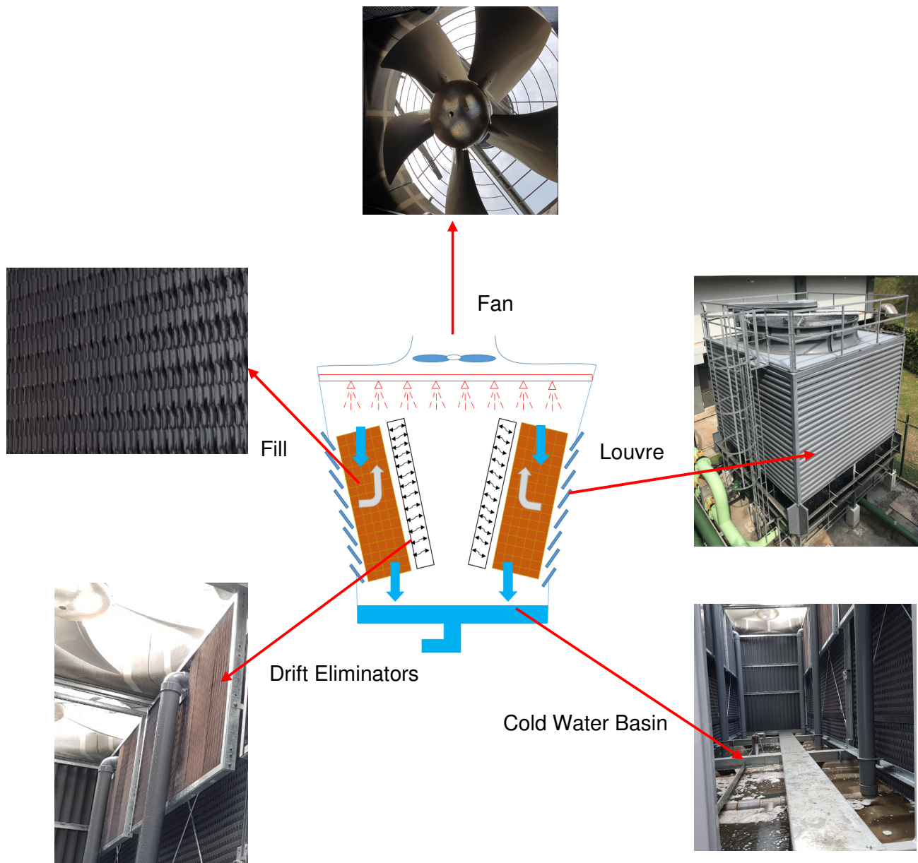
Figure 5. Photos of cooling tower components
