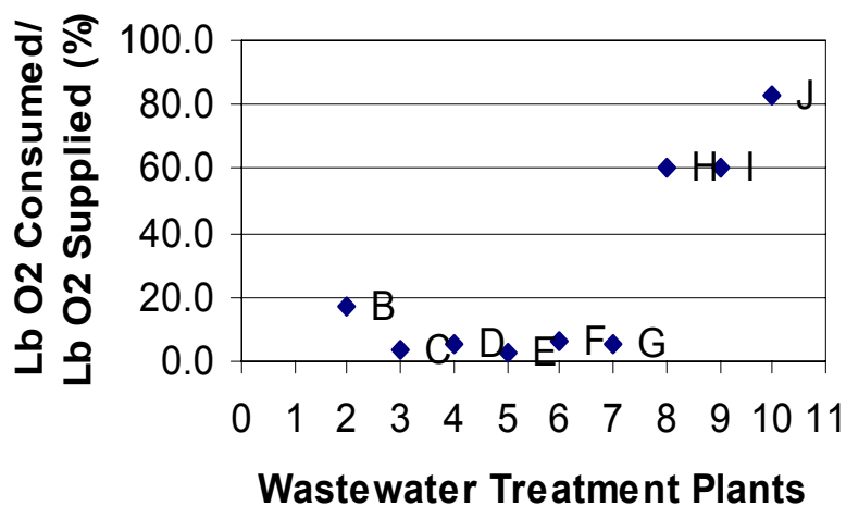
Figure 5. Oxygen Transfer Efficiency
