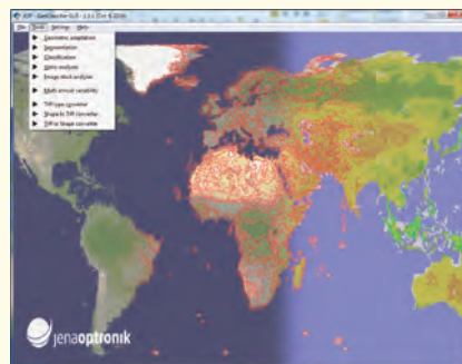
Figure 48: Geoclassifier toolbox
