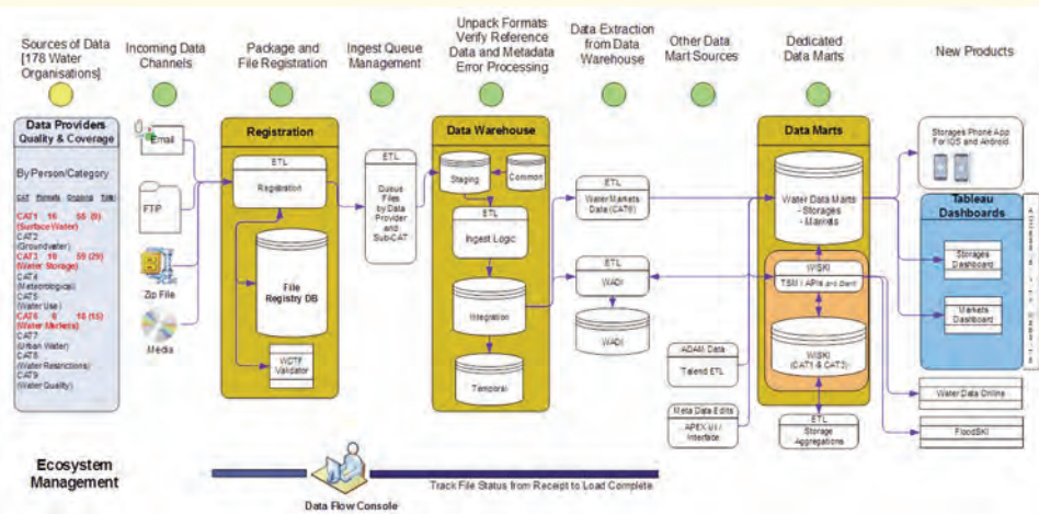
Figure 29: AWRIS ecosystem
