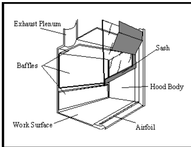
Hood and vent components
