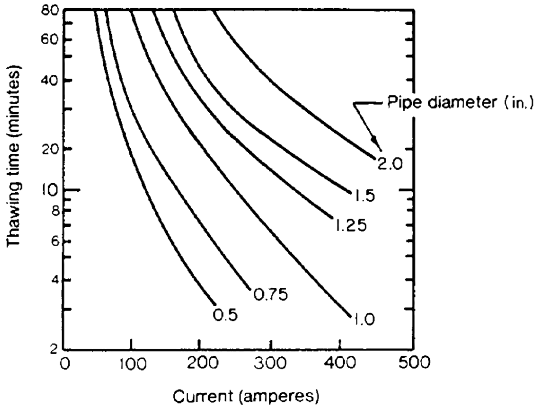
Figure 13 Approximate times and current for thawing steel pipes
