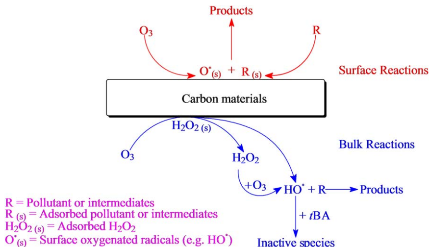
Figure 4.3 Illusion of the mainly reaction mechanism for the pollutant degradation during ozonation in the presence of carbon materials. Reproduced from ref. 127 with permission from Elsevier, Copyright 2009.
