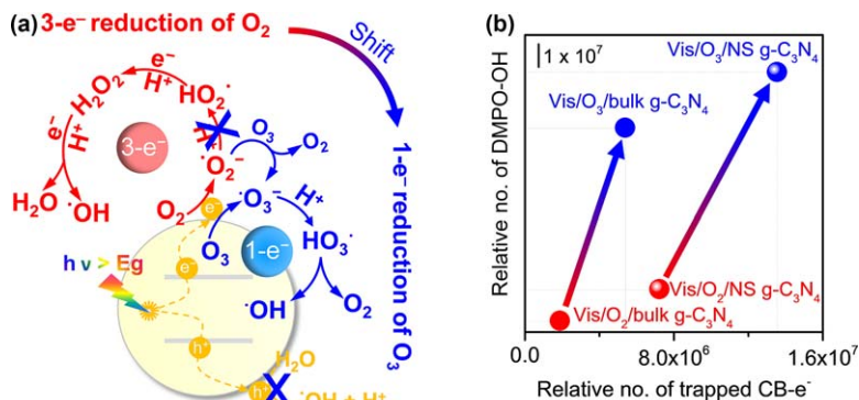
Figure 7.5 (a) Proposed pathways of \bullet\text{OH} generation in vis/ \text{O}_3/\text{g-C}_3\text{N}_4 . (b) Relative number of DMPO–OH as a function of the number of trapped \text{CB-e}^- . Adapted from ref. 13 with permission from American Chemical Society, Copyright 2020.
