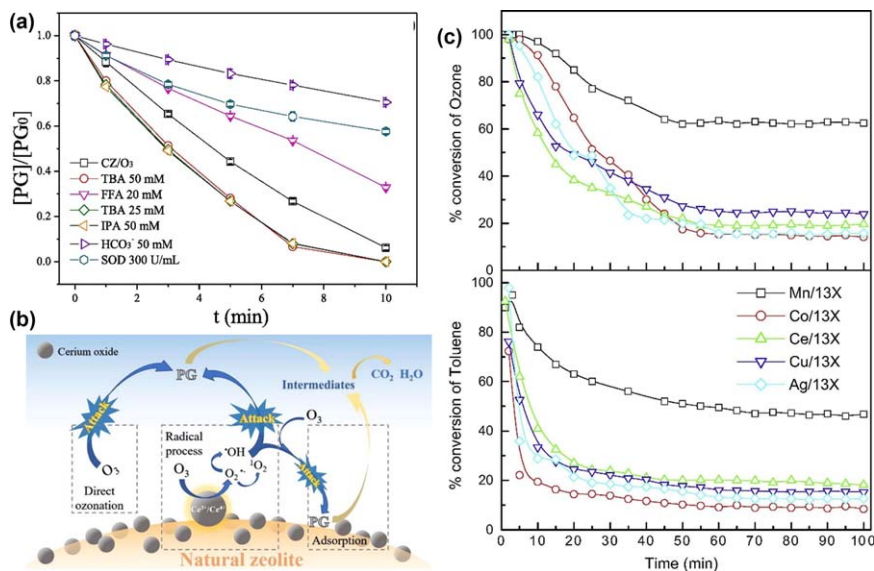
Figure 2.2 (a) Effect of scavengers on penicillin G removal efficiency in Ce-loaded natural zeolite catalytic ozonation system. (b) Reaction mechanism of penicillin G degradation in Ce-loaded natural zeolite catalytic ozonation system. Reproduced from ref. 35 with permission from Elsevier, Copyright 2019. (c) Change in the conversions of toluene and ozone with time on Mn/13X, Co/13X, Ce/13X, Ag/13X and Cu/13X catalysts. Reproduced from ref. 38 with permission from Elsevier, Copyright 2019.
