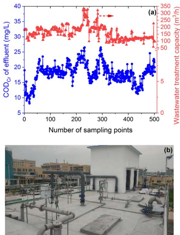
Figure 4.4 (a) Variations of \text{COD}_{\text{Cr}} of effluent and wastewater treatment capacity. (b) Full-scale application of ozonation of the wastewater from a fine chemical industry park in the presence of AC-supported iron oxide. Reaction conditions: ozone gas concentration: 30 \text{ mg L}^{-1} ; \text{COD}_{\text{Cr}} of influent: 35\text{--}40 \text{ mg L}^{-1} ; reaction time: 20 min.
