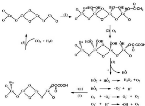
Figure 8.3 Catalytic mechanism of CeO 2 in the O 3 /H 2 O 2 process. Reproduced from ref. 20 with permission from Elsevier, Copyright 2018.
