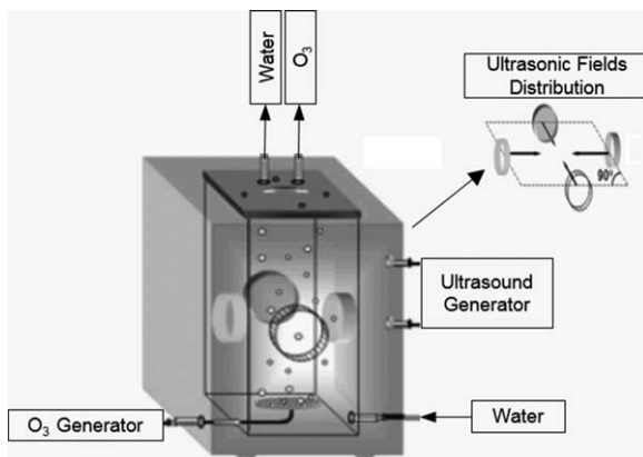
Figure 10.2 Device diagram of ultrasonic reactor with multifields.
