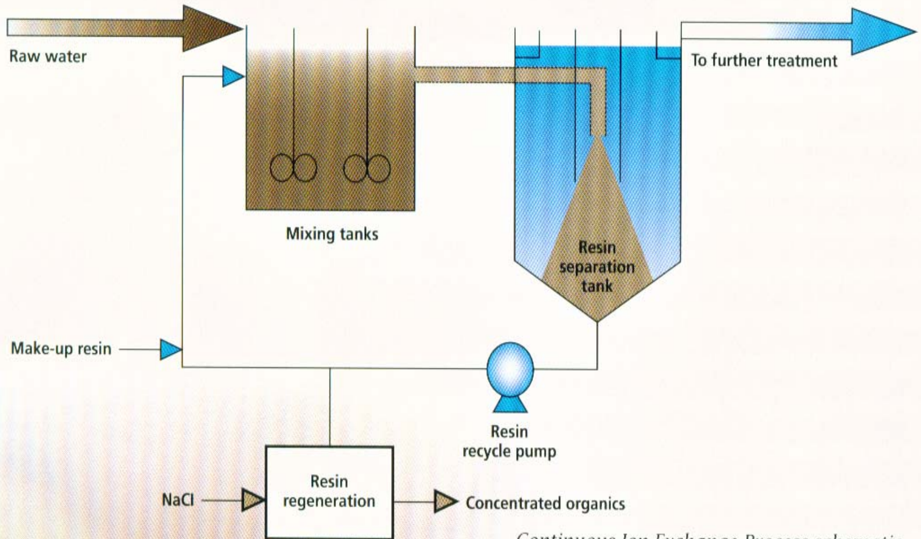
Continuous Ion Exchange Process schematic.
