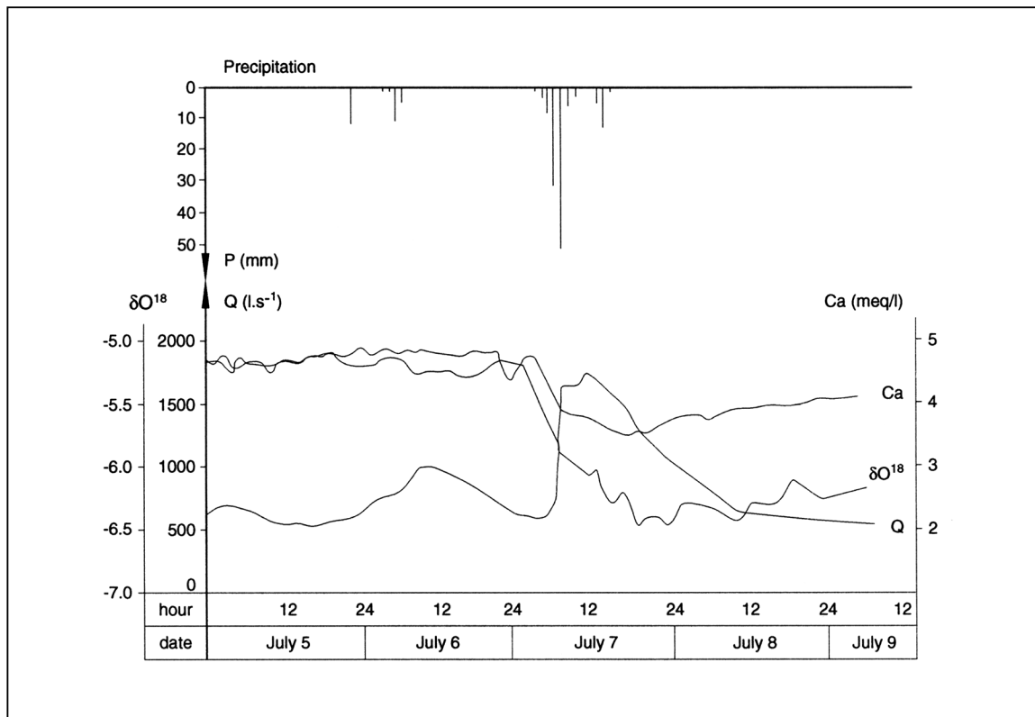
Figure 14.5 The hydrological, hydrochemical and isotopic response to a storm of S31 karst spring near Yaji, Guilin, China 1986 (Yuan Daoxian, 1988)
