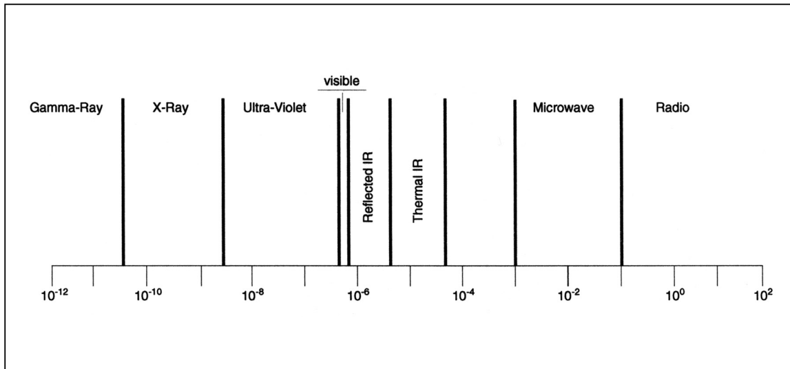
Figure 5.1 Electromagnetic spectrum
