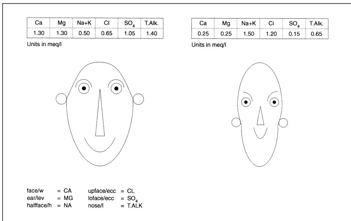
Figure 4.11 Chernoff faces of water chemistries
