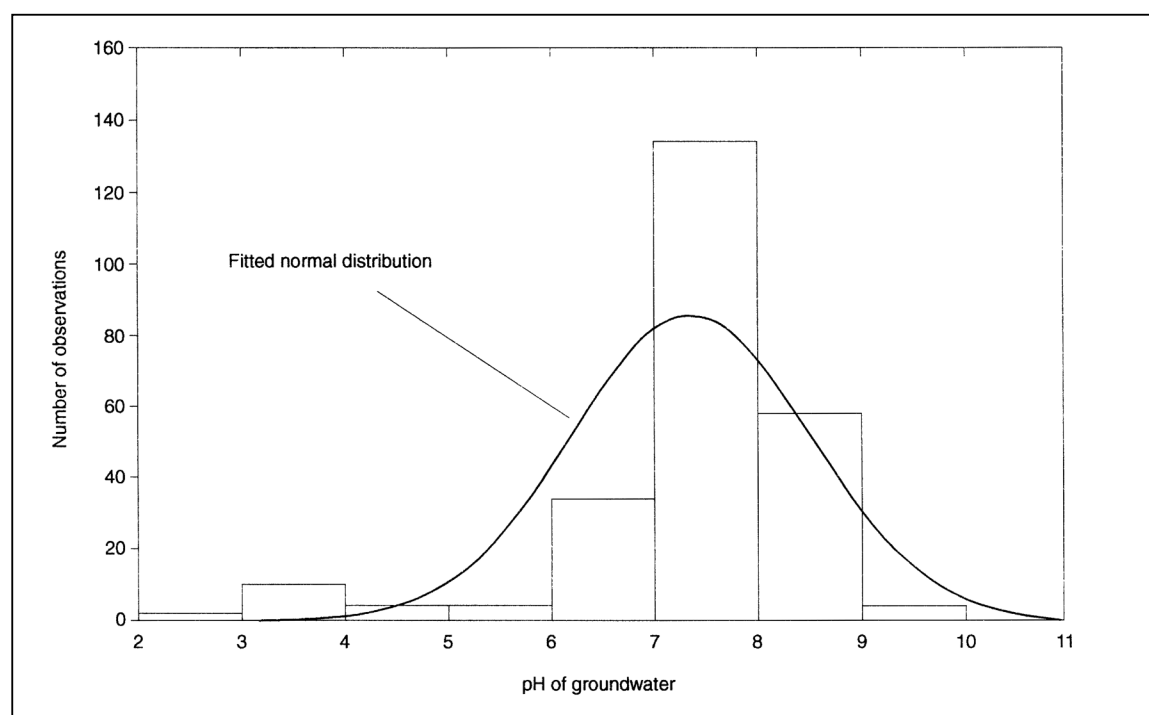
Figure 4.15 Histogram of groundwater pH levels from a mining environment
