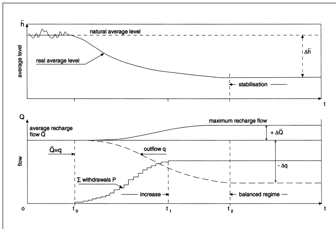
Figure 12.2 Exploitation under a dynamic balance strategy after a necessary transitional phase: diagram of changing average levels – global indicator of the state of the storage – and flows. P is less than Q . The stabilisation of levels (on average) is deferred (in t_2 ) in relation to that of withdrawals (in t_1 ). After a withdrawal phase from t_0 to t_2 , there is a time lag until the levels stabilise; the effect of the withdrawals in t_1 results in the levels at t_2
