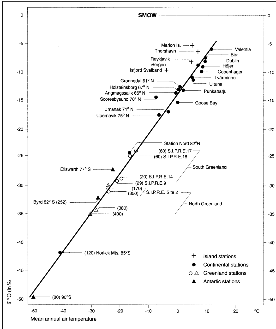
Figure 9.1 The annual mean \delta^{18}\text{O} of precipitation as a function of the mean annual air temperature at surface. The figures in parentheses indicate the total thickness (in cm) of the investigated snow layers (Modified after Dansgaard, 1964)
