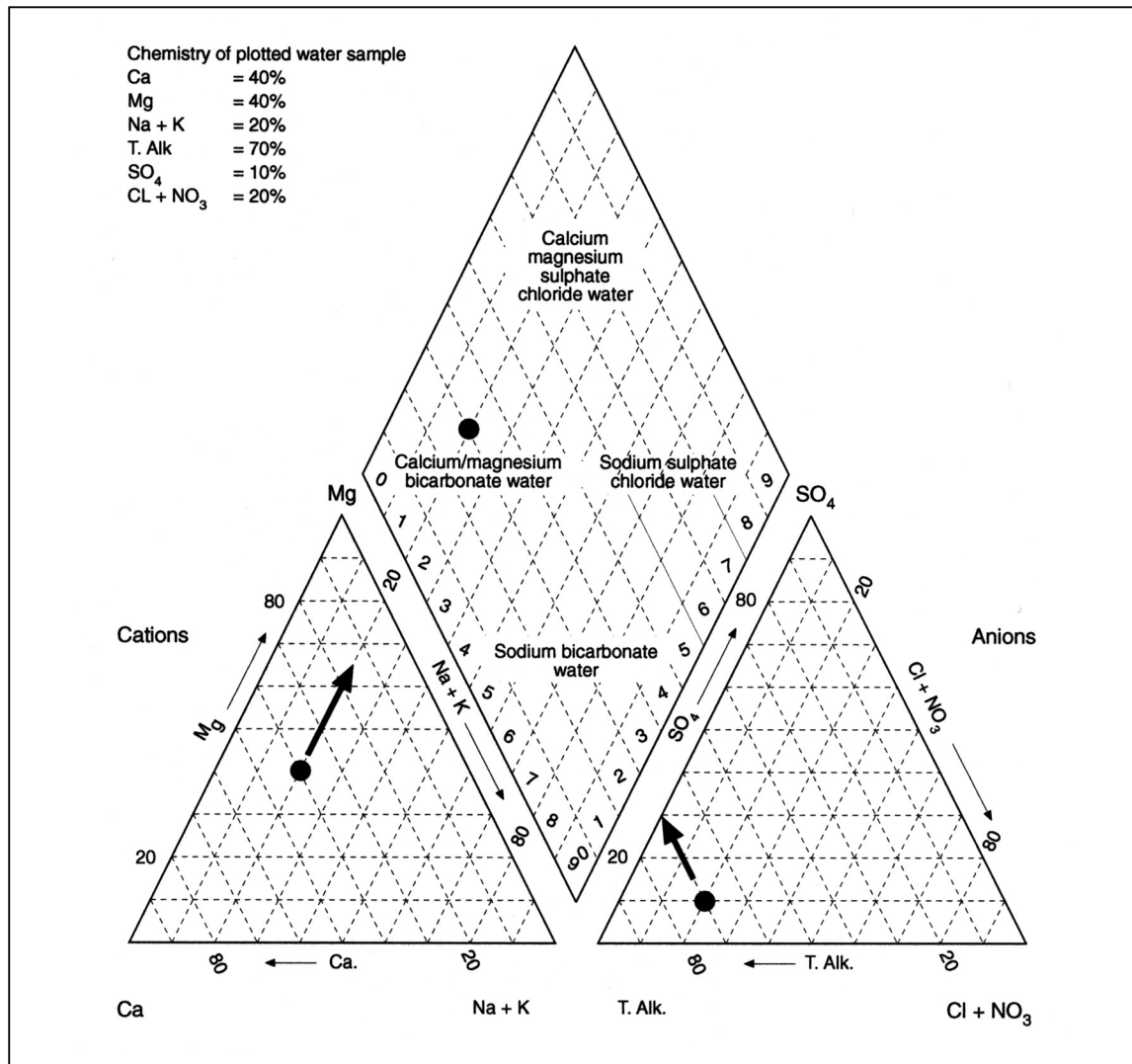
Figure 4.3 Plotting procedures for the Piper diagram: Convert mg/l to meq/l by division (Ca/20, Mg/12, Na/23, K/39, T.Alk./50, \text{SO}_4/48 , \text{Cl}/35.5 , \text{NO}_3/62 . Add Na +K and Cl + \text{NO}_3 . Calculate percentage of cations and anions. Plot cations by scaling off Ca, then Mg. Plot anions by scaling off T.Alk. then \text{SO}_4 . Project cation and anion points to triangle
