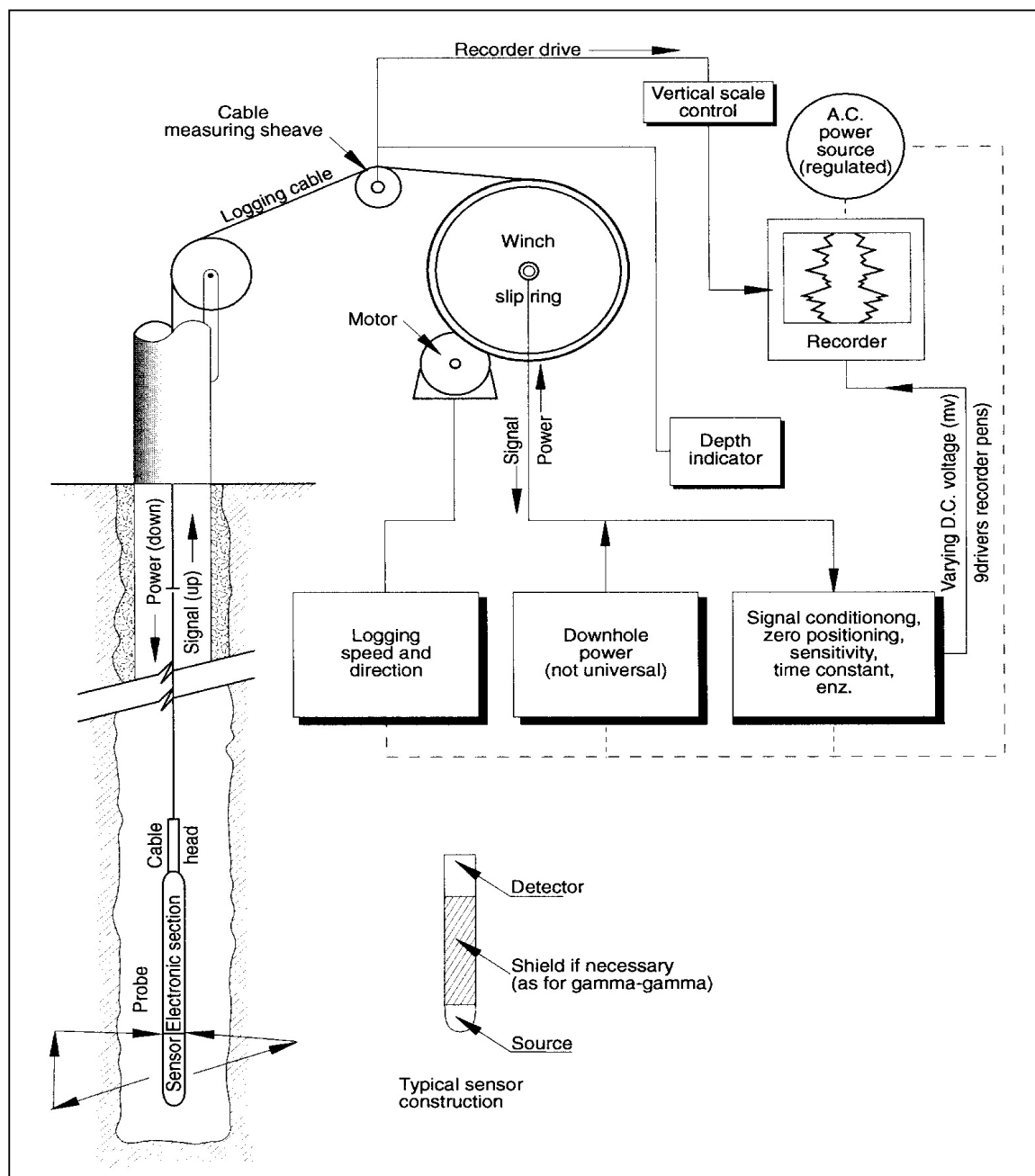
Figure 6.27 Basic components of geophysical borehole logging (Keys and MacCary, 1971)
