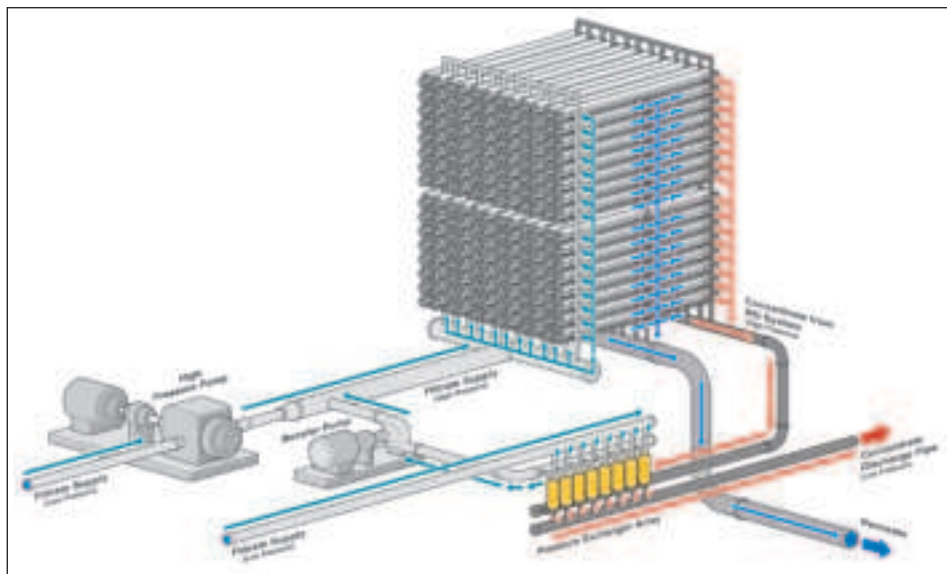
Figure 3. Pressure exchanger energy recovery system.
