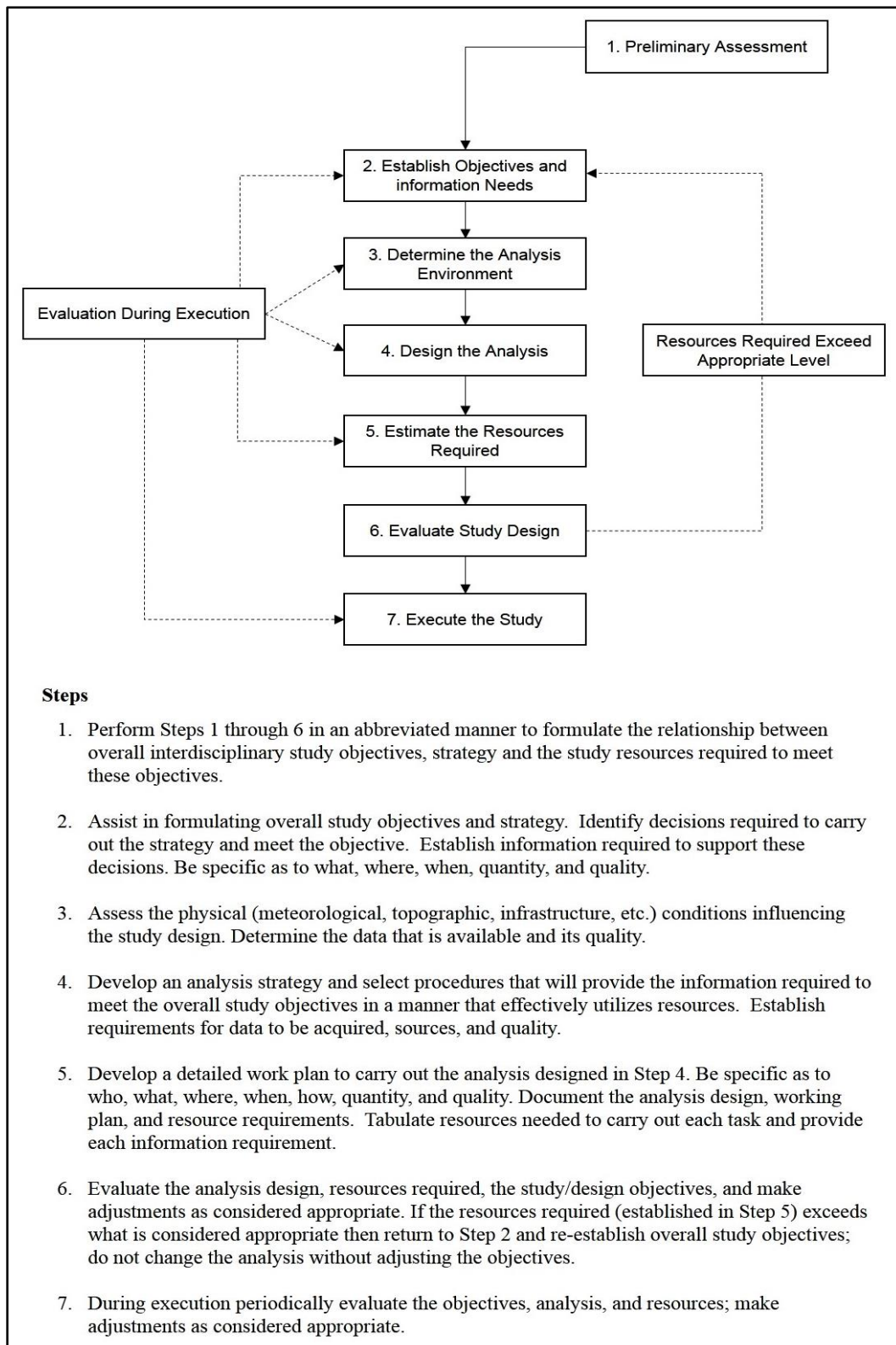
Figure 3-1. Formulation steps.
