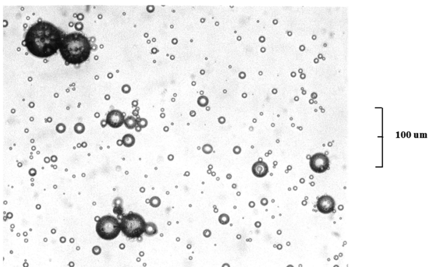
Example of offshore produced water droplet size distribution - note very few solids particles presents
