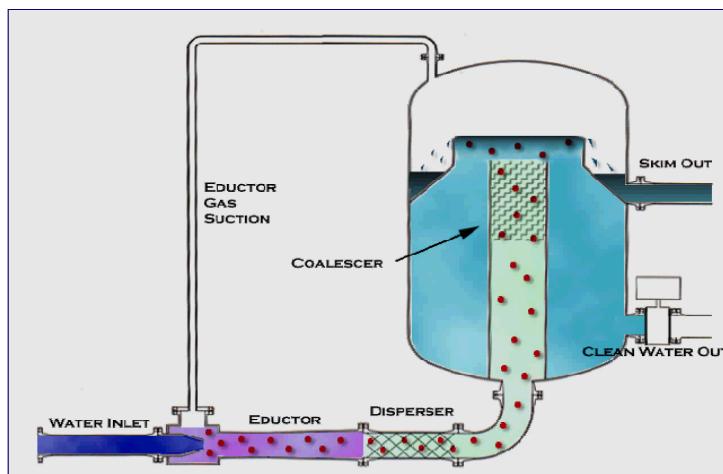
Unicel IGF design
