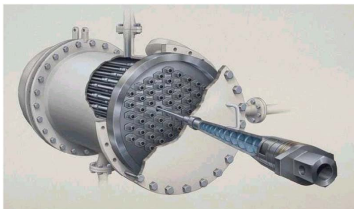
Packaging of many liners within a single pressure vessel. This figure shows the reject header.
