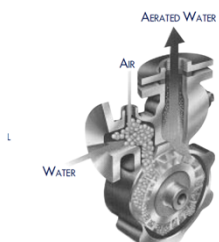
The New DAF pump
