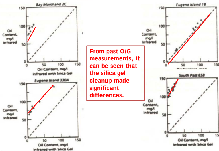
Figure 9. Correlations of infrared versus infrared with silica gel analyses of produced brine samples. 9
