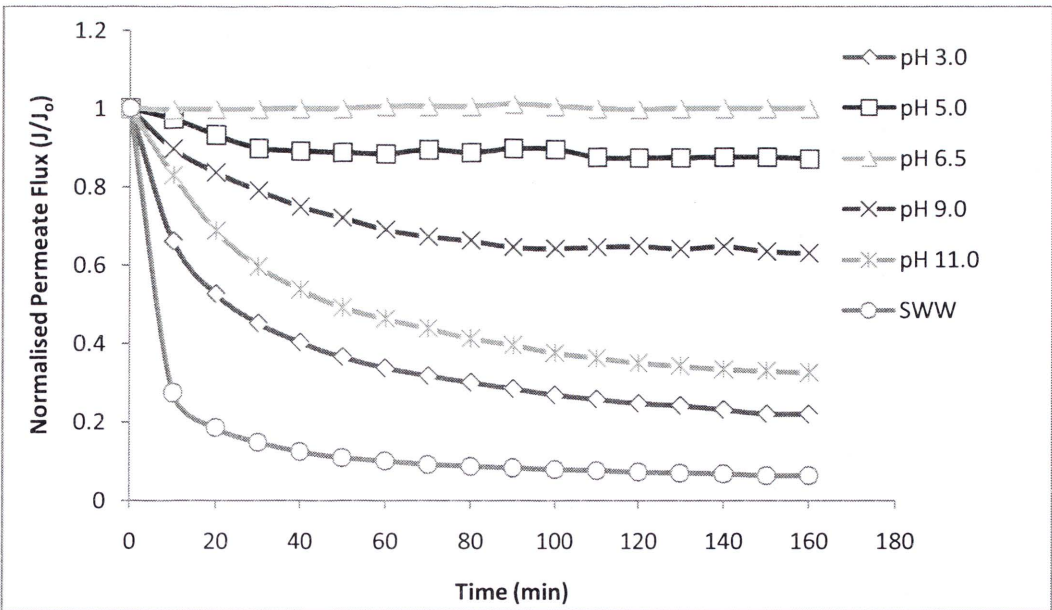
Figure 4.15 Normalised permeate flux through MF for chemical coagulation (transmembrane pressure 10 kPa, cross flow velocity 0.5 l min -1 ).
