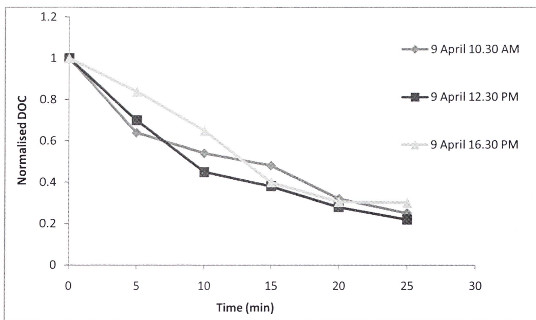
Figure 4.25 Variation of DOC at three different times in a day. (Initial turbidity = 80 NTU, initial UV= 0.150 cm -1 , electrodes gap= 2 cm, pH= 8.0 and current density= 2.11 mA cm -2 ).
