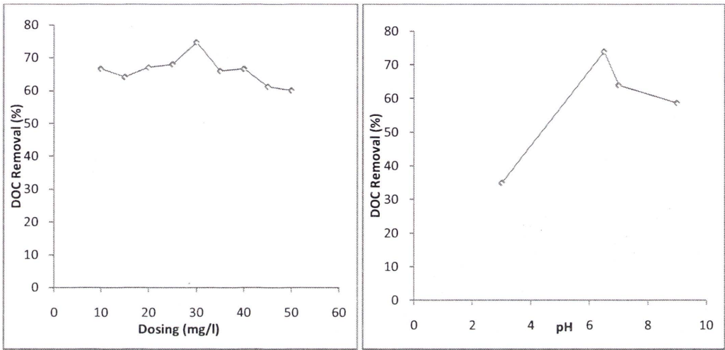
Figure 4.5 DOC removal at different dosing at neutral condition (left) and at different pH with optimum dosing (right).
