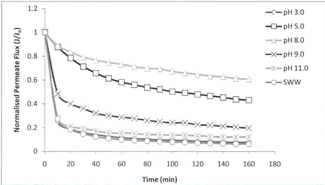
Figure 4.14 Normalised permeate flux through MF for EC using aluminium plates (transmembrane pressure 10 kPa, cross flow velocity 0.5 l min -1 ).
