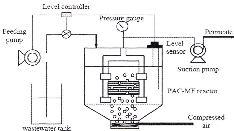
Figure 2.2 Experimental set-up of submerged membrane adsorption hybrid system (Adapted from Guo et al., 2006)
