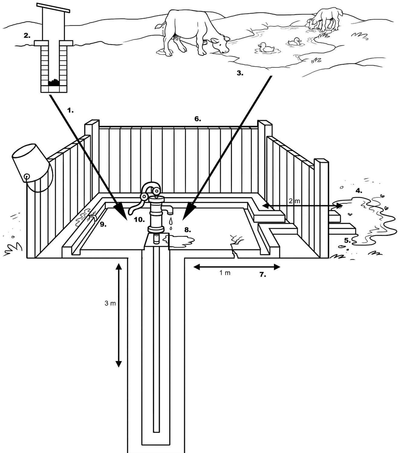
Illustration of Borehole with Hand Pump
