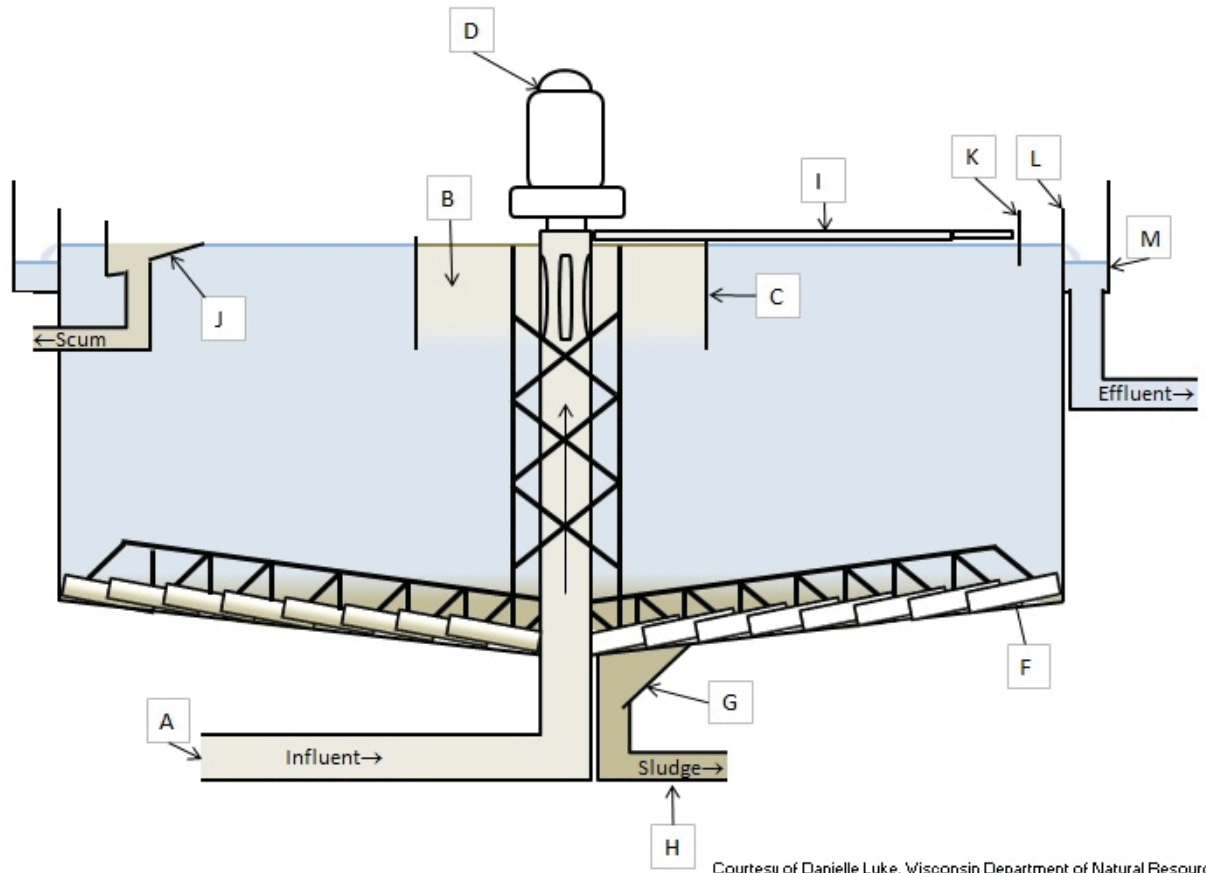
Cross Section of a Primary or Intermediate Circular Center-Feed Clarifier
